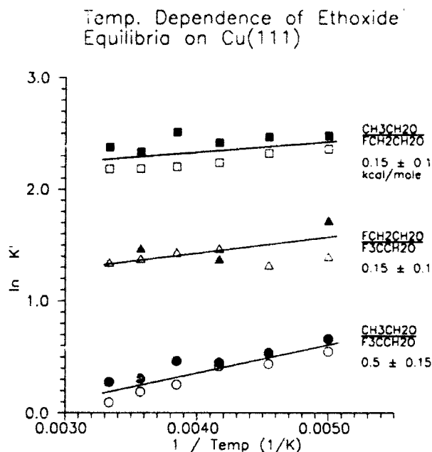
Figure 7. \ln(K') vs 1/T for mixtures of ethanol, monofluoroethanol, and trifluoroethanol on the Cu(111) surface. K' is the ratio of desorption signals of the two ethoxides on the surface and is proportional to the equilibrium constant K for reaction between gas-phase ethanols and surface ethoxides. The slopes in kcal/mol are given on the figure. Exposure was 30 L.
