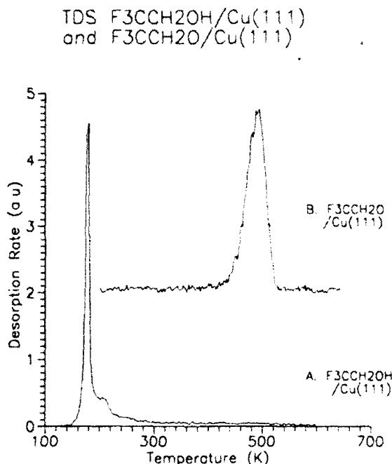
Figure 1. (A) Thermal desorption of F_3CCH_2OH on Cu(111) surface. m/q = 31 amu, \beta = 5 K/s. (B) Thermal desorption of F_3CCH_2OH on preoxidized Cu(111). Desorbing species is F_3CCHO from F_3CCH_2O_{(ad)} decomposition. m/q = 98 amu, \beta = 5 K/s.
