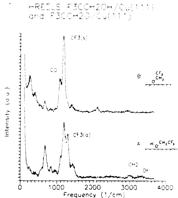
Figure 2. (A) HREELS of F_3CCH_2OH on Cu(111) ( I_d = 0.7 \times 10^3 cps, FWHM = 75 cm^{-1} ). (B) HREELS of F_3CCH_2O on Cu(111) ( I_d = 1.1 \times 10^3 cps, FWHM = 70 cm^{-1} ). E_i = 5.5 eV.
