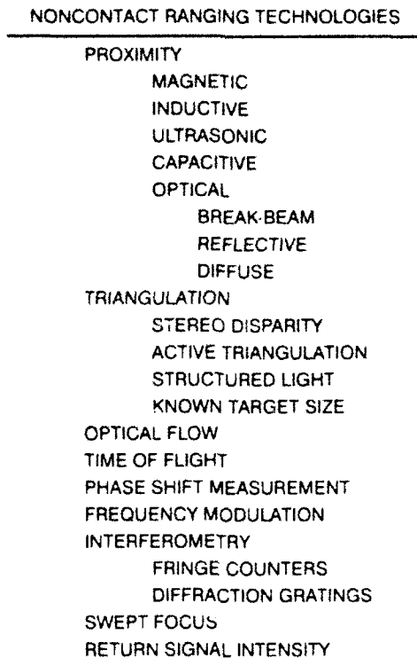
Figure 1. Taxonomy of noncontact ranging methods for mobile robots (Everett, 1987).
