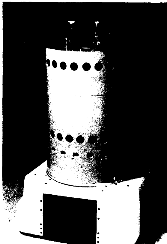
Figure 41. Quantic's Wide Angle Optical Ranging System will be employed on this modular robot developed by NCCOSC.
