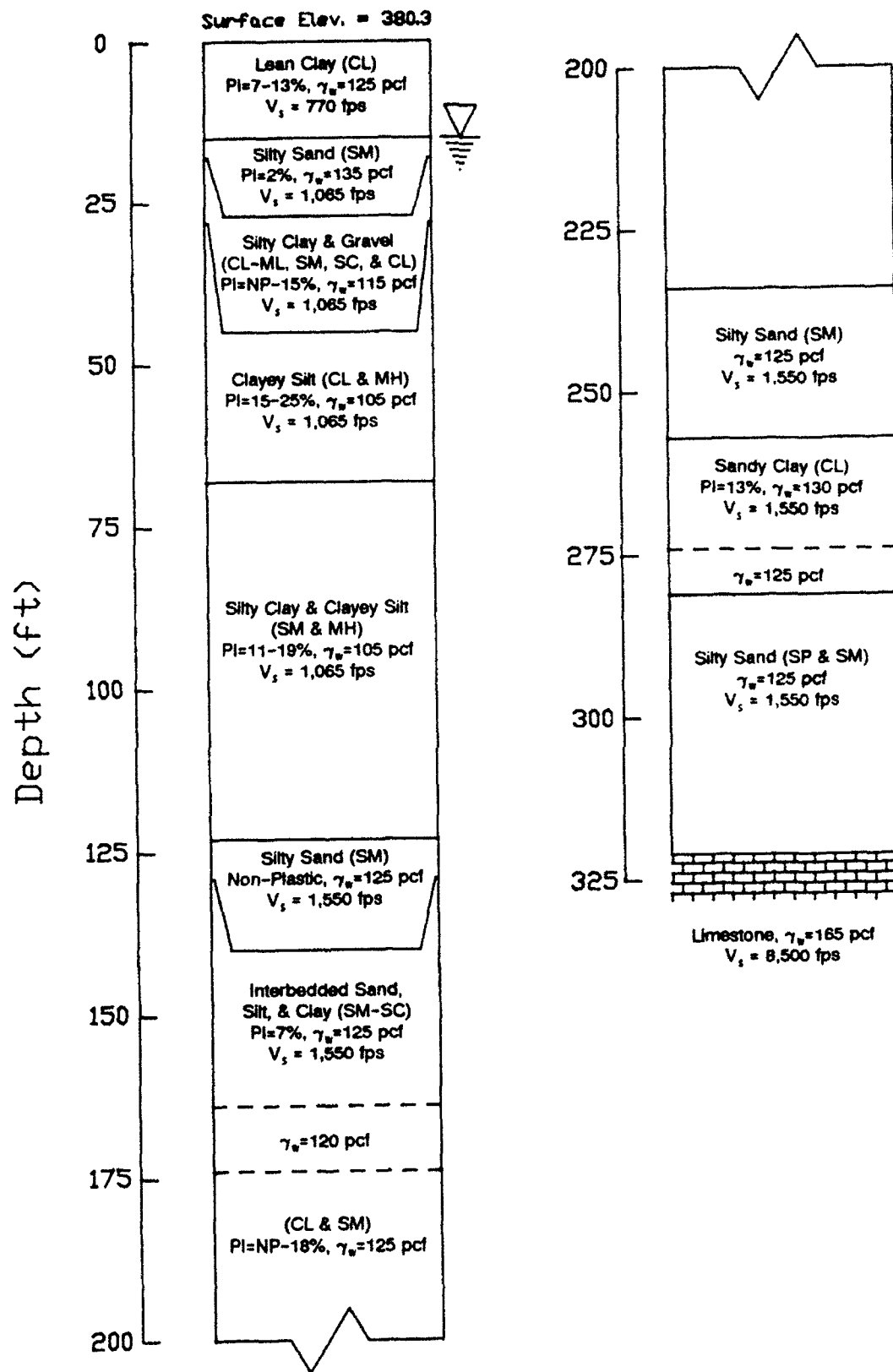
Figure 19. Soil column for Site 1
