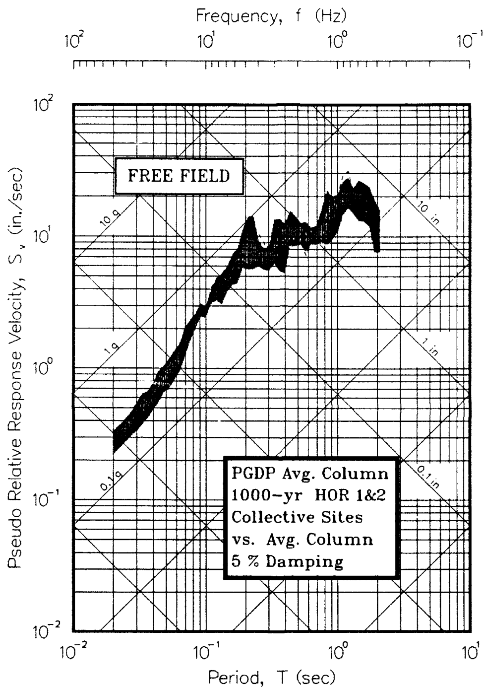
Figure 51. Comparison of results for average column and range produced from individual sites
