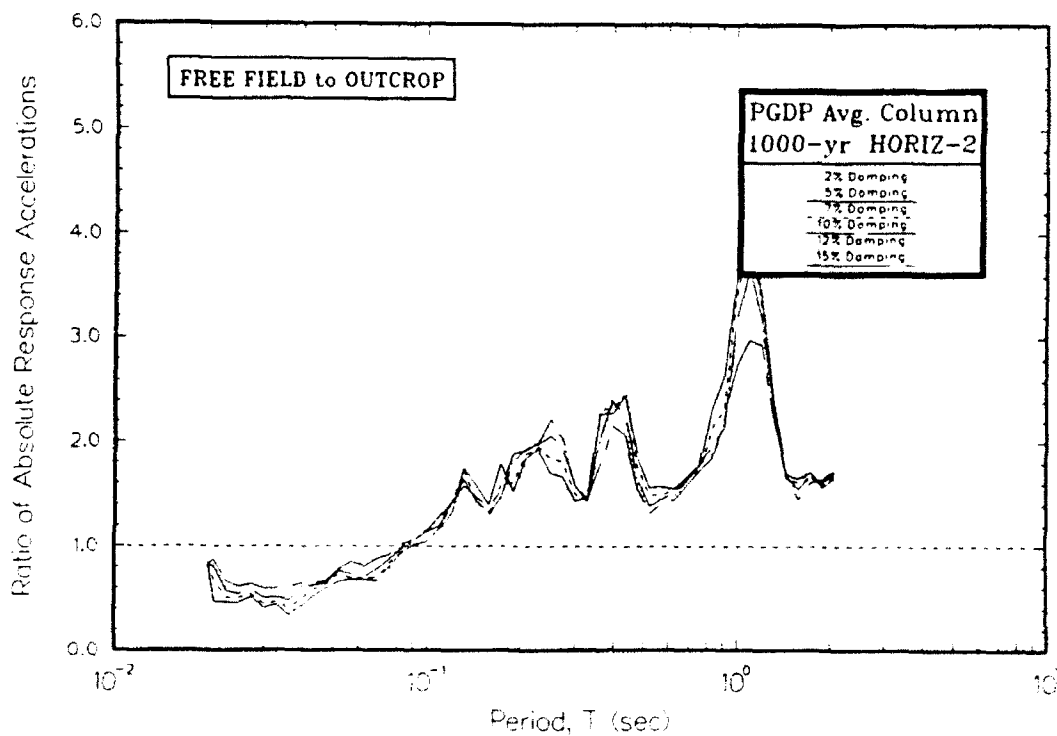
Figure U13. Ratio of absolute acceleration response spectra at free field to rock using best estimate of modulus for average column
