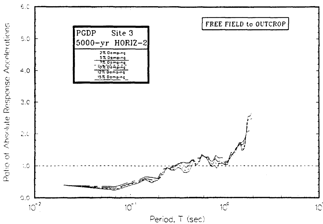
Figure R3. Ratio of absolute acceleration response spectra at free field to rock for Site 3
