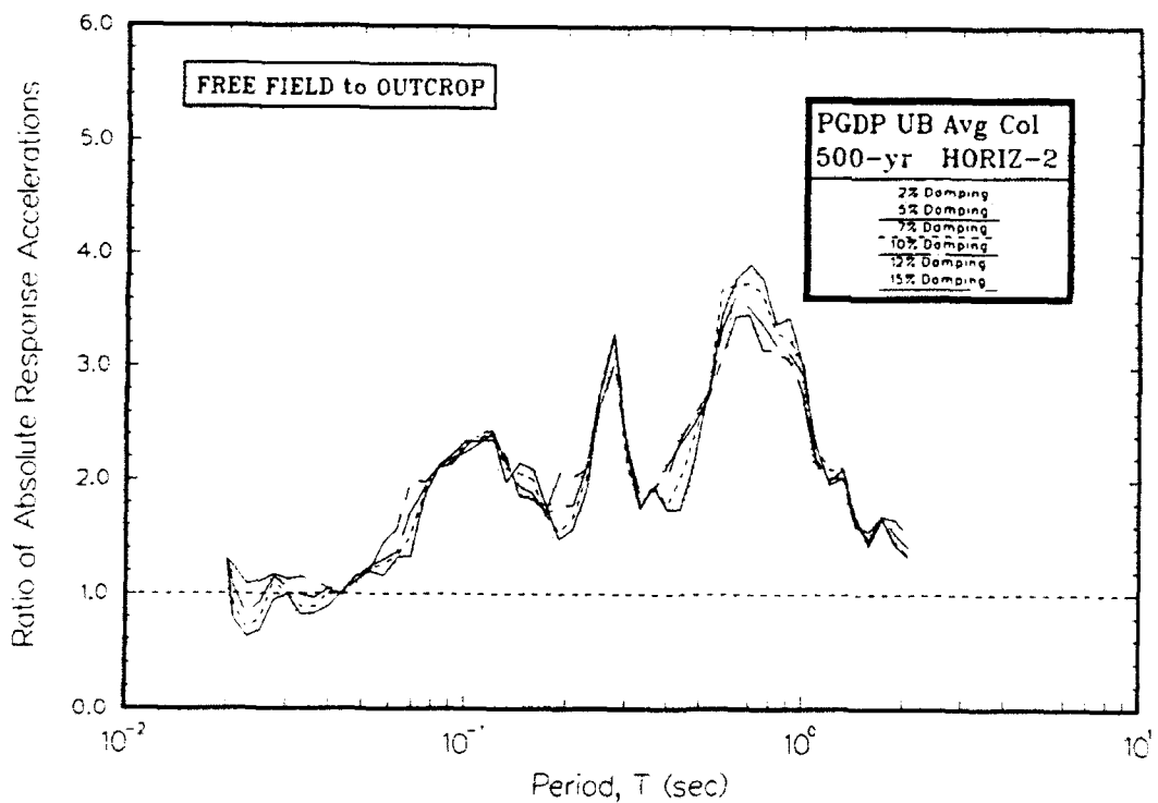
Figure T15. Ratio of absolute acceleration response spectra at free field to rock using upper bound of modulus for average column
