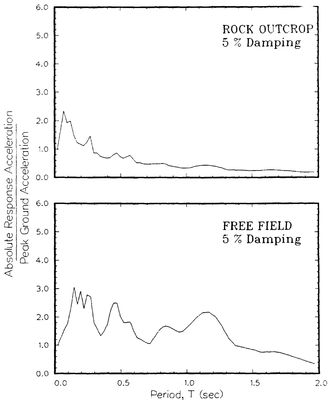
Figure 38. Example figure showing the amplification ratios (absolute acceleration response spectra normalized to peak horizontal acceleration) for rock outcrop and free field motions
