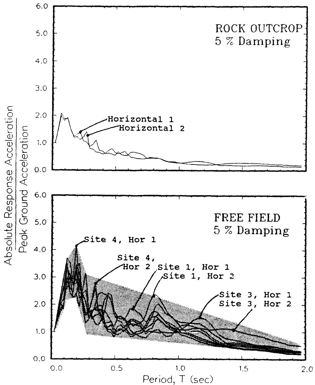
Figure 42. Amplification ratio for 500-year event
