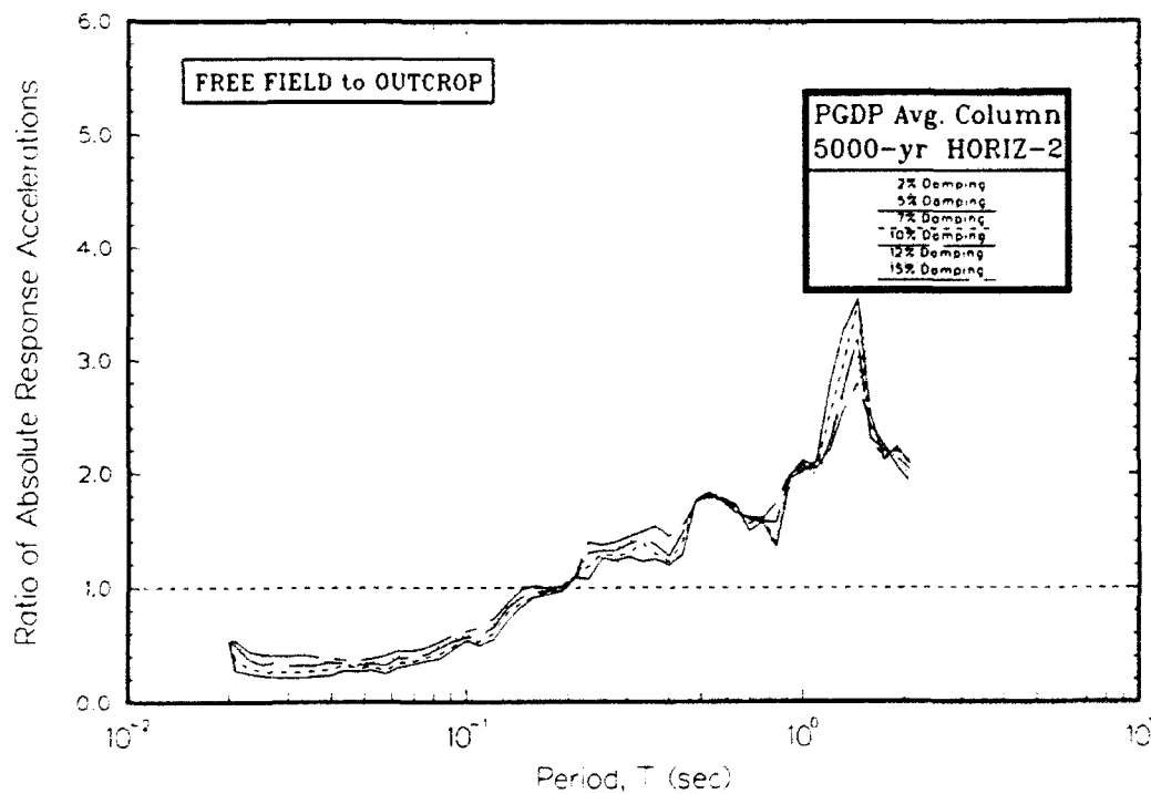
Figure V9. Ratio of absolute acceleration response spectra at free field to rock using best estimate of modulus for average column
