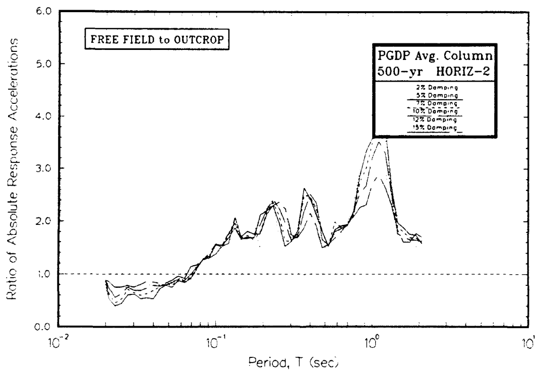
Figure T13. Ratio of absolute acceleration response spectra at free field to rock using best estimate of modulus for average column
