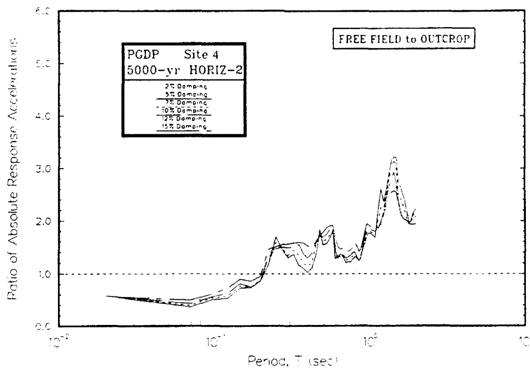
Figure R4. Ratio of absolute acceleration response spectra at free field to rock for Site 4
