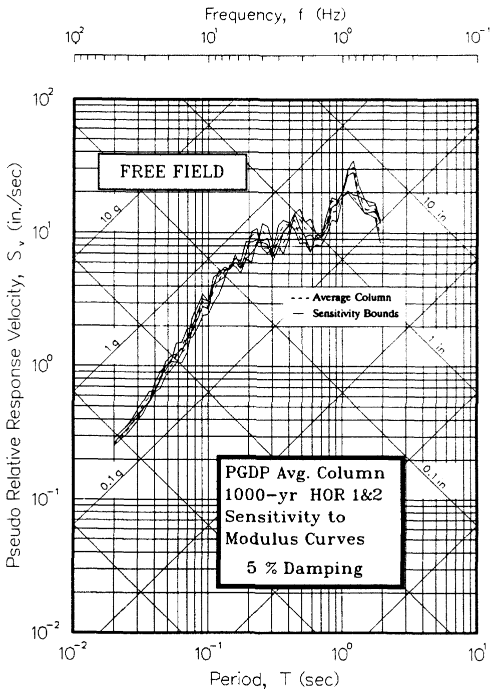
Figure 56. Pseudo-velocity response spectra showing sensitivity of results to modulus curves
