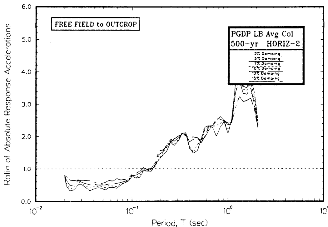
Figure T14. Ratio of absolute acceleration response spectra at free field to rock using lower bound of modulus for average column
