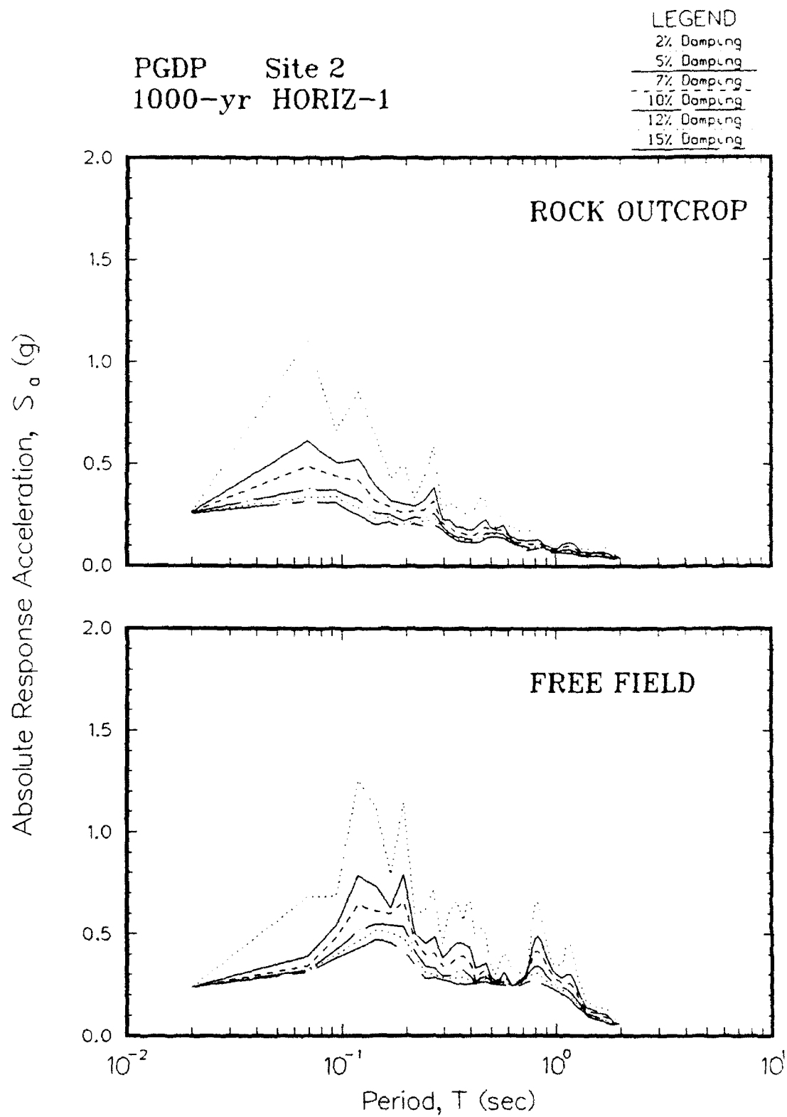
Figure 36. Example figure showing the absolute acceleration response spectra for rock outcrop and free-field motions
