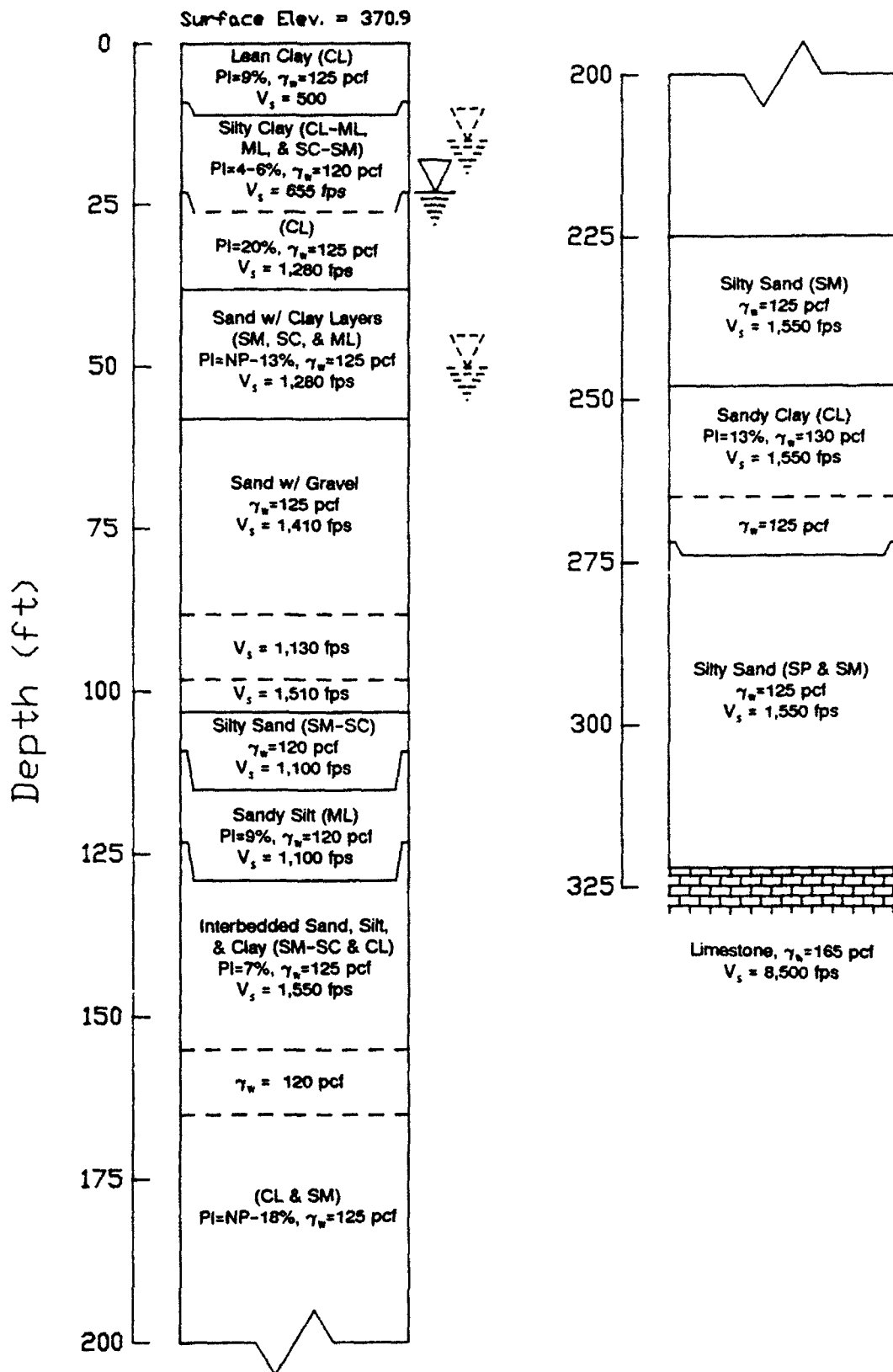
Figure 22. Soil column for Site 4
