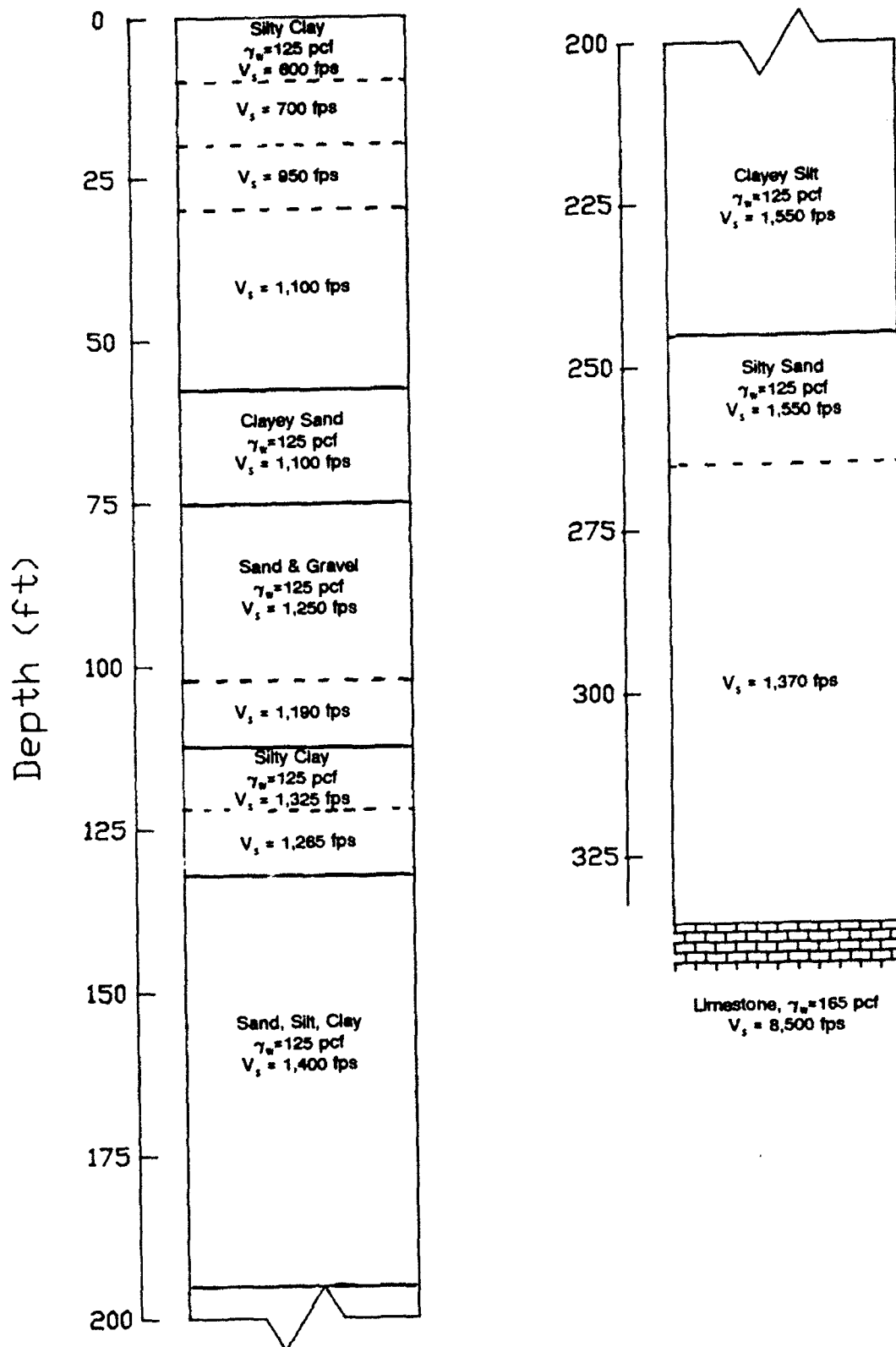
Figure 30. Average soil column
