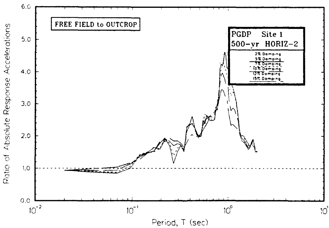
Figure F1. Ratio of absolute acceleration response spectra at free field to rock for Site 1
