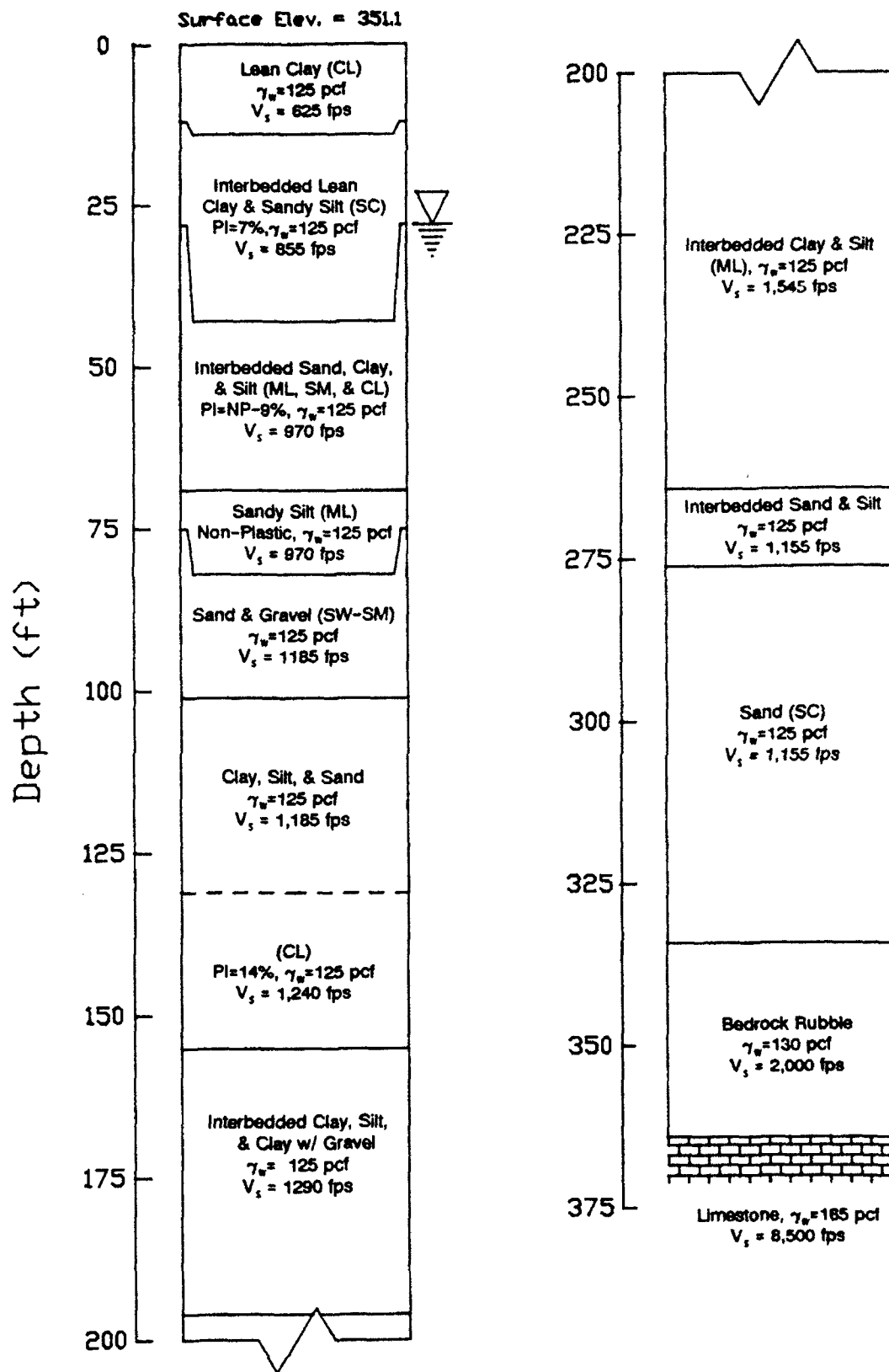
Figure 21. Soil column for Site 3
