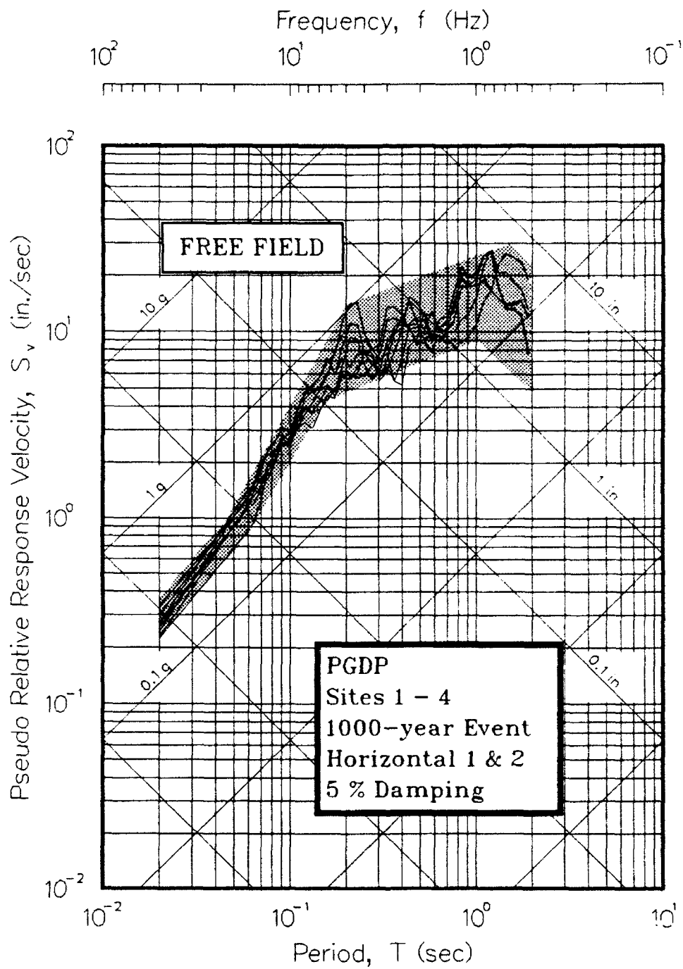
Figure 43. Pseudo-velocity response spectra for 1000-year event
