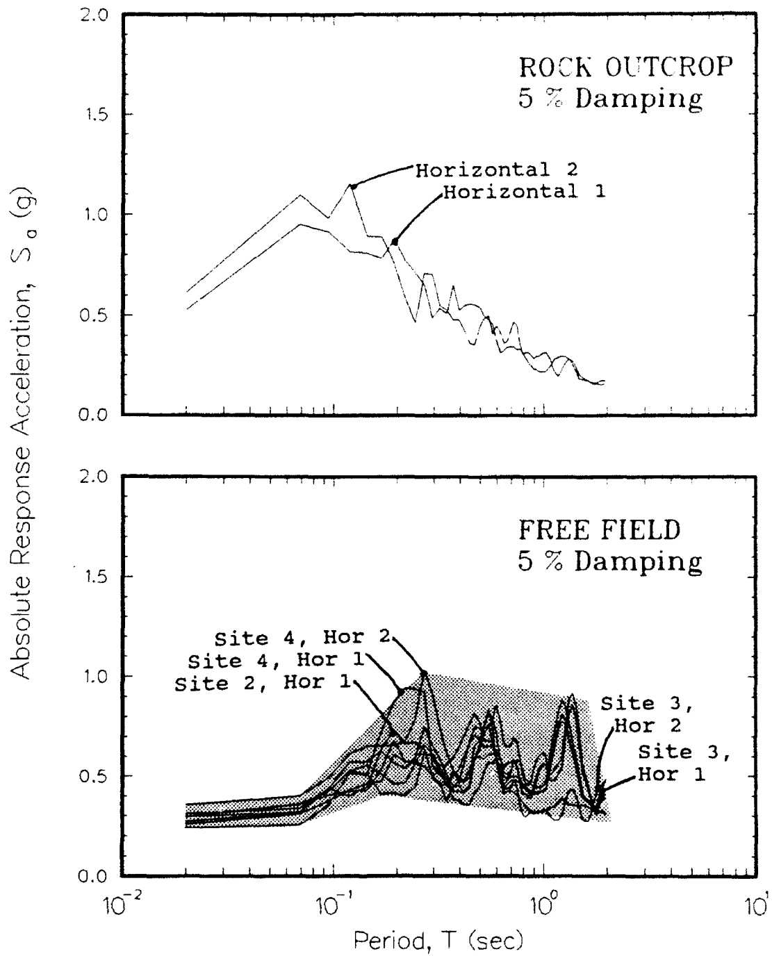
Figure 48. Absolute response acceleration spectra for 5000-year event
