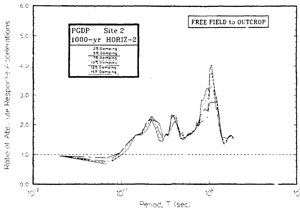
Figure L2. Ratio of absolute acceleration response spectra at free field to rock for Site 2
