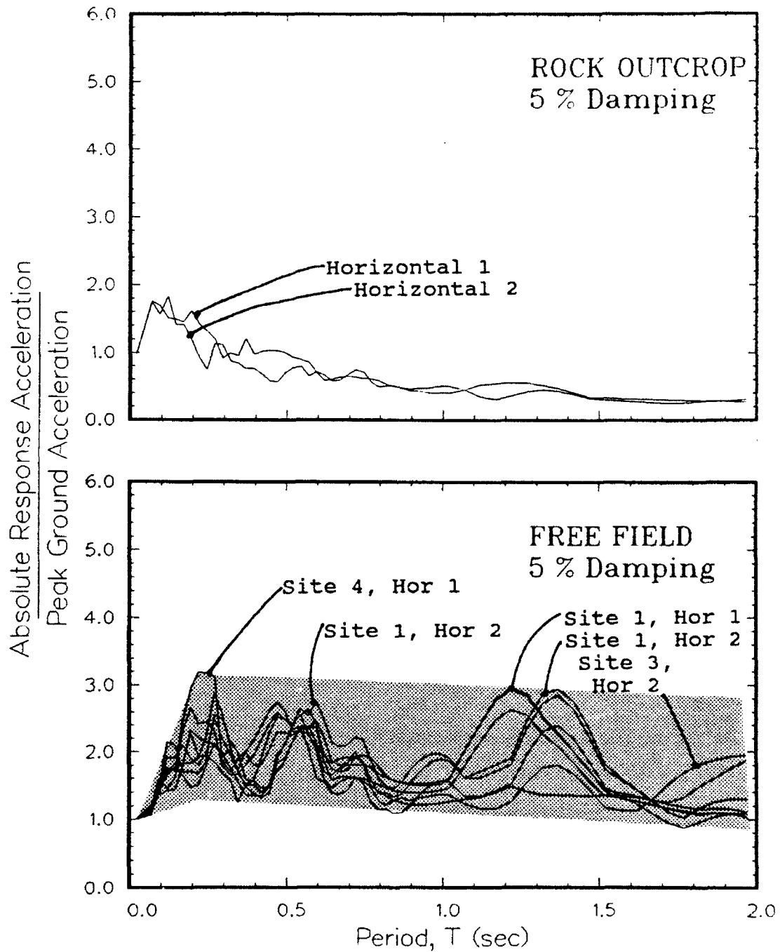
Figure 50. Amplification ratio for 5000-year event
