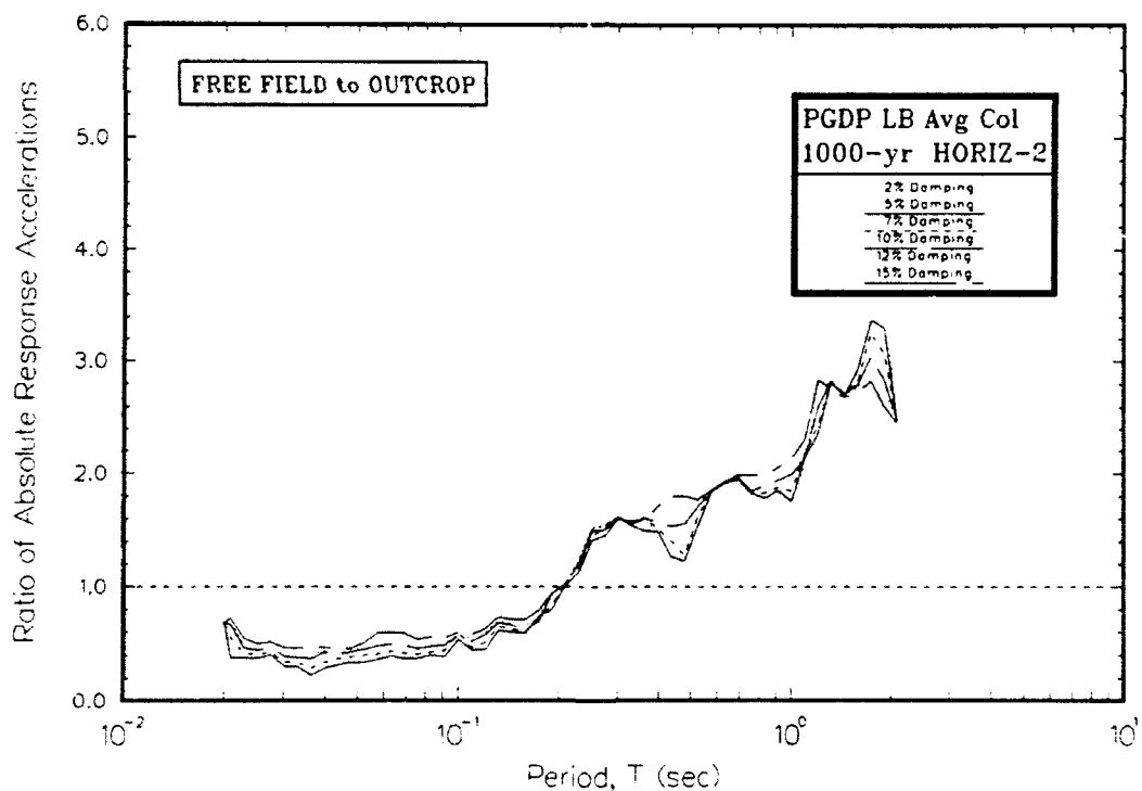
Figure U14. Ratio of absolute acceleration response spectra at free field to rock using lower bound of modulus for average column
