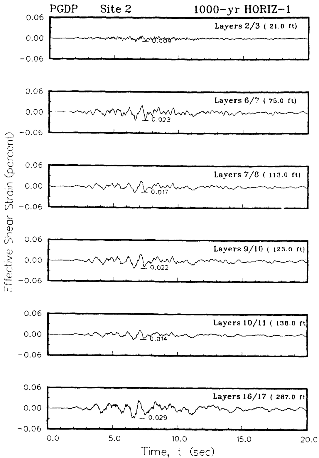
Figure 34. Example figure showing a profile of the variation of effective shear strain with time
