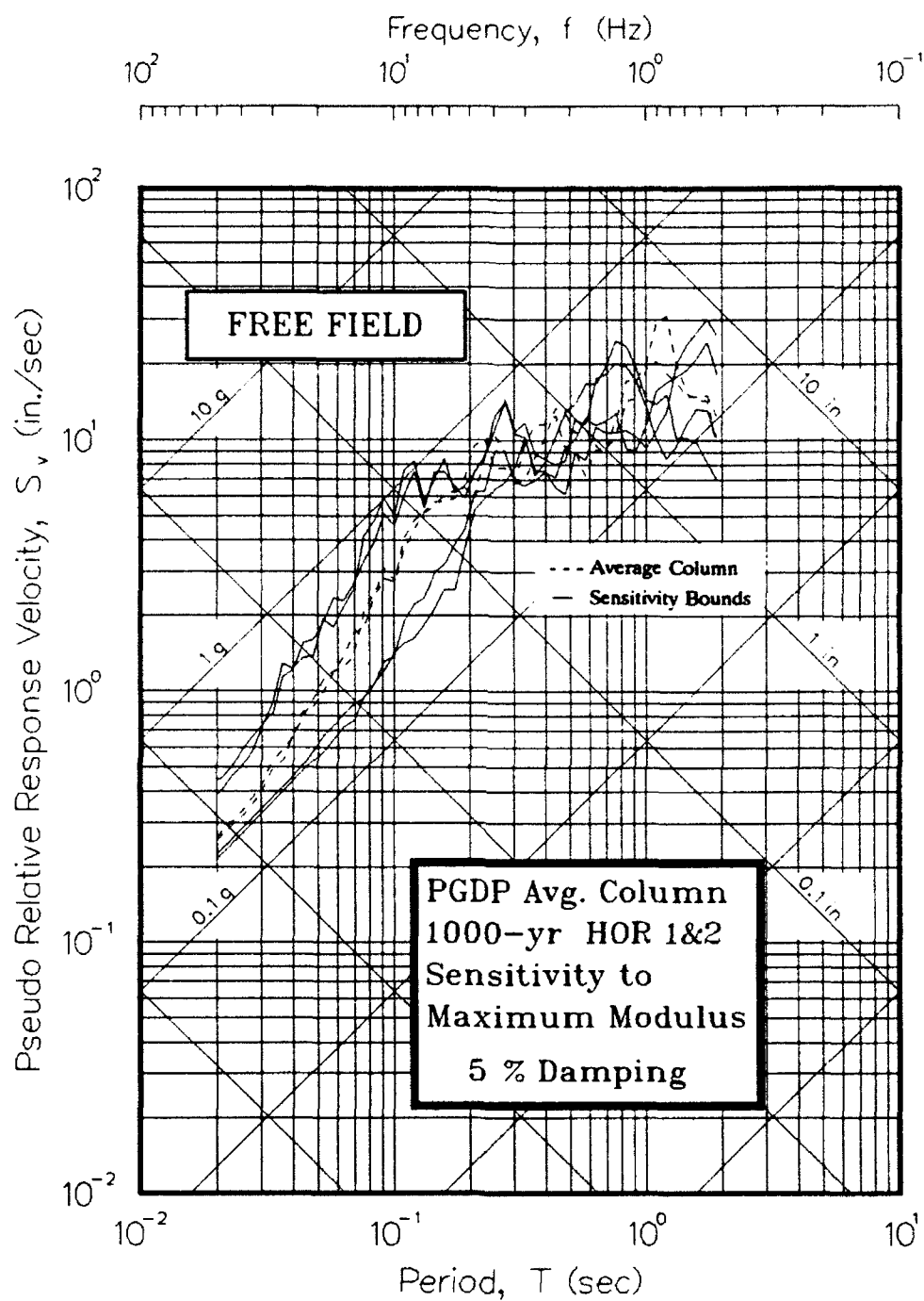
Figure 59. Pseudo-velocity response spectra showing sensitivity of results to maximum shear modulus
