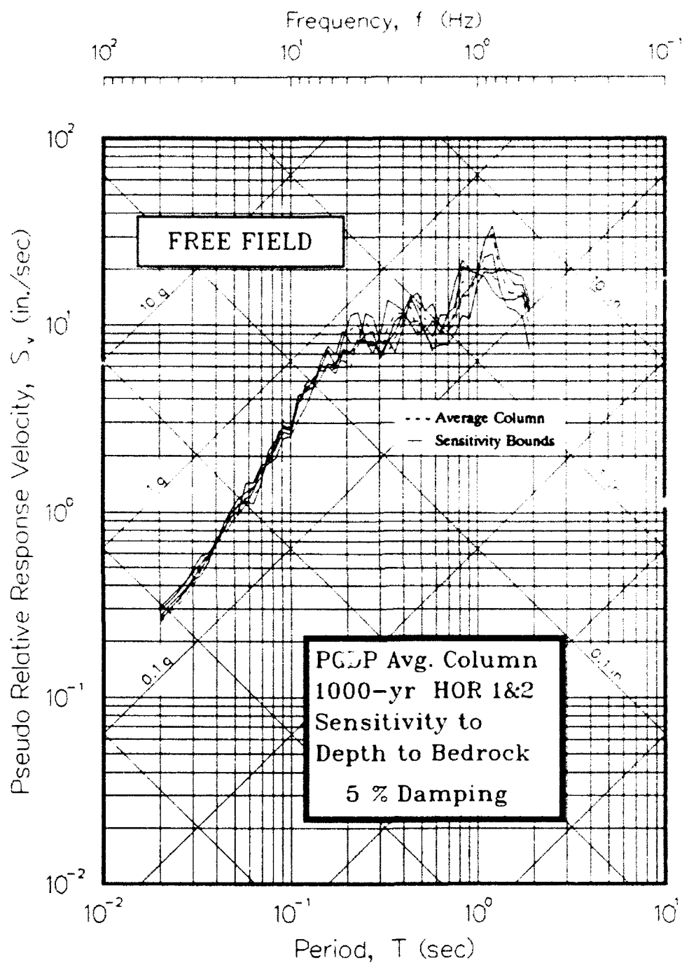
Figure 54. Pseudo-velocity response spectra showing sensitivity of results to depth of bedrock
