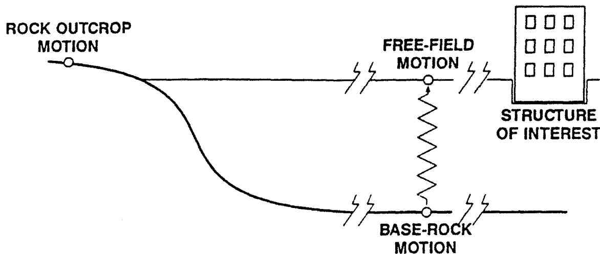
Figure 3. Three primary control points for a site response analysis
