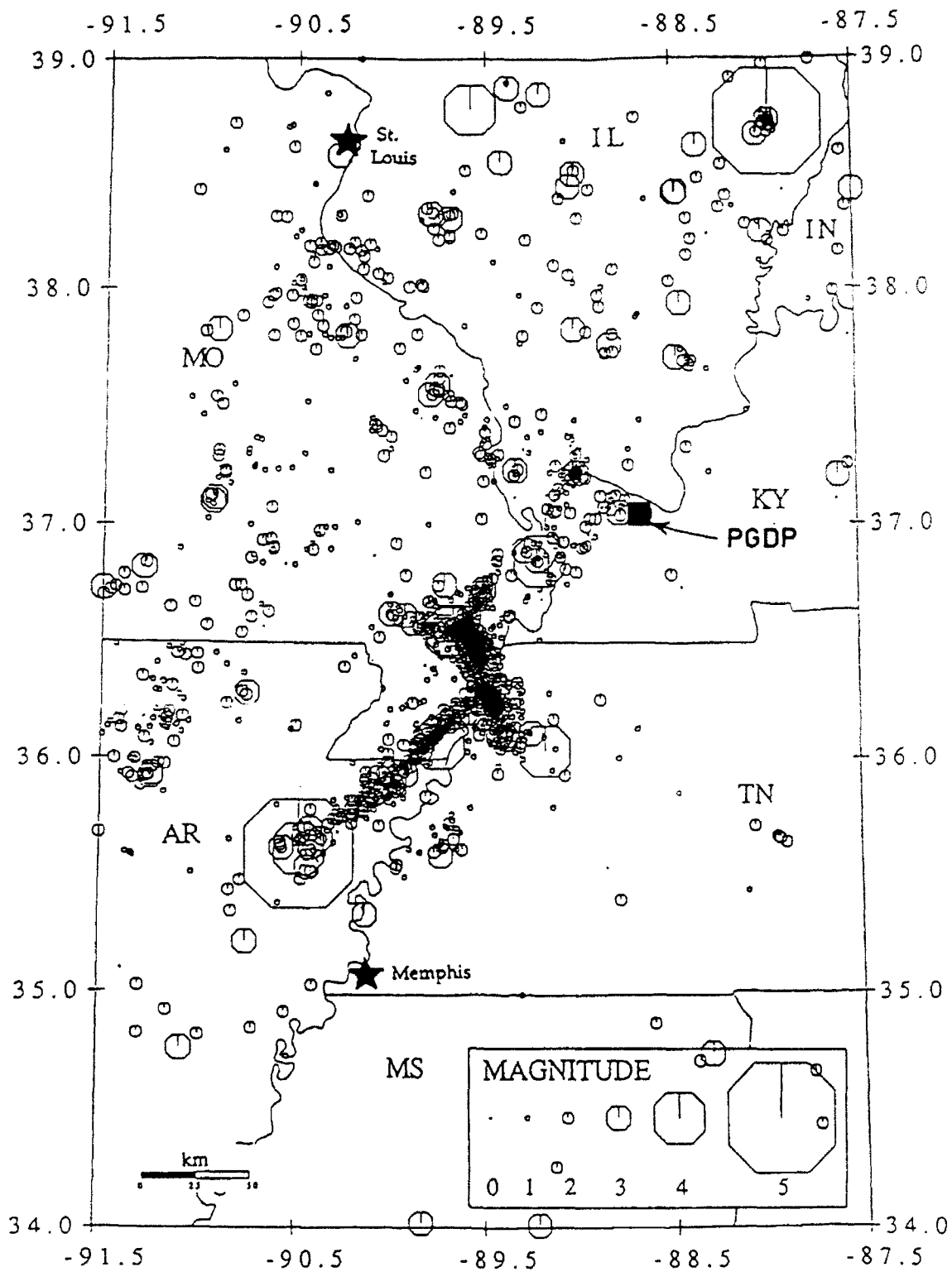
Figure 4. Seismic activity in central U.S. during 189-month period between 1974 and 1990 (courtesy of Saint Louis University)
