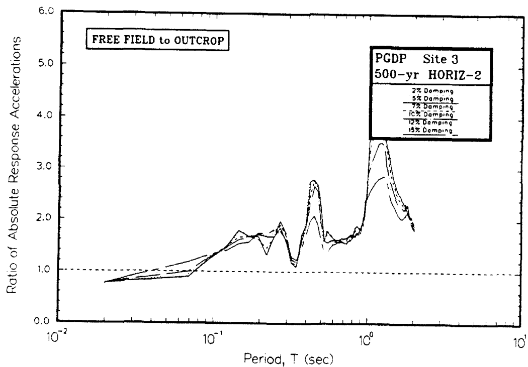
Figure F3. Ratio of absolute acceleration response spectra at free field to rock for Site 3
