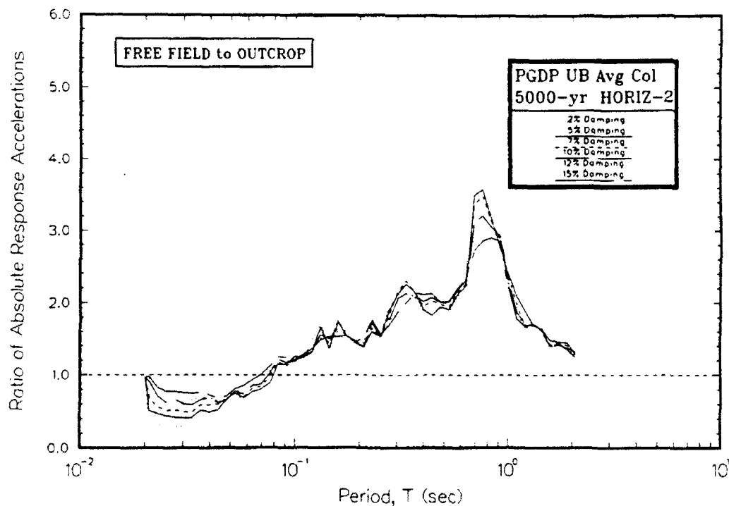
Figure V10. Ratio of absolute acceleration response spectra at free field to rock using upper bound of modulus for average column
