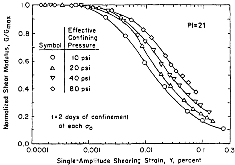
b. San Francisco Bay mud (Stokoe and Lodde 1978)
