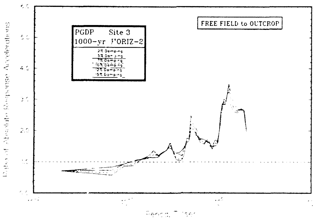
Figure L3. Ratio of absolute acceleration response spectra at free field to rock for Site 3
