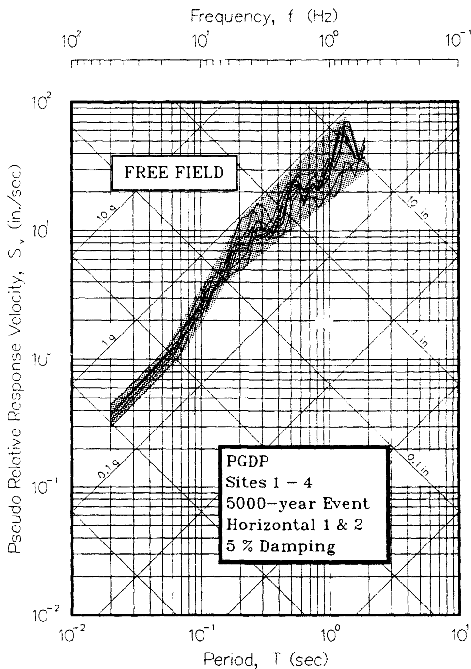
Figure 47. Pseudo-velocity response spectra for 5000-year event
