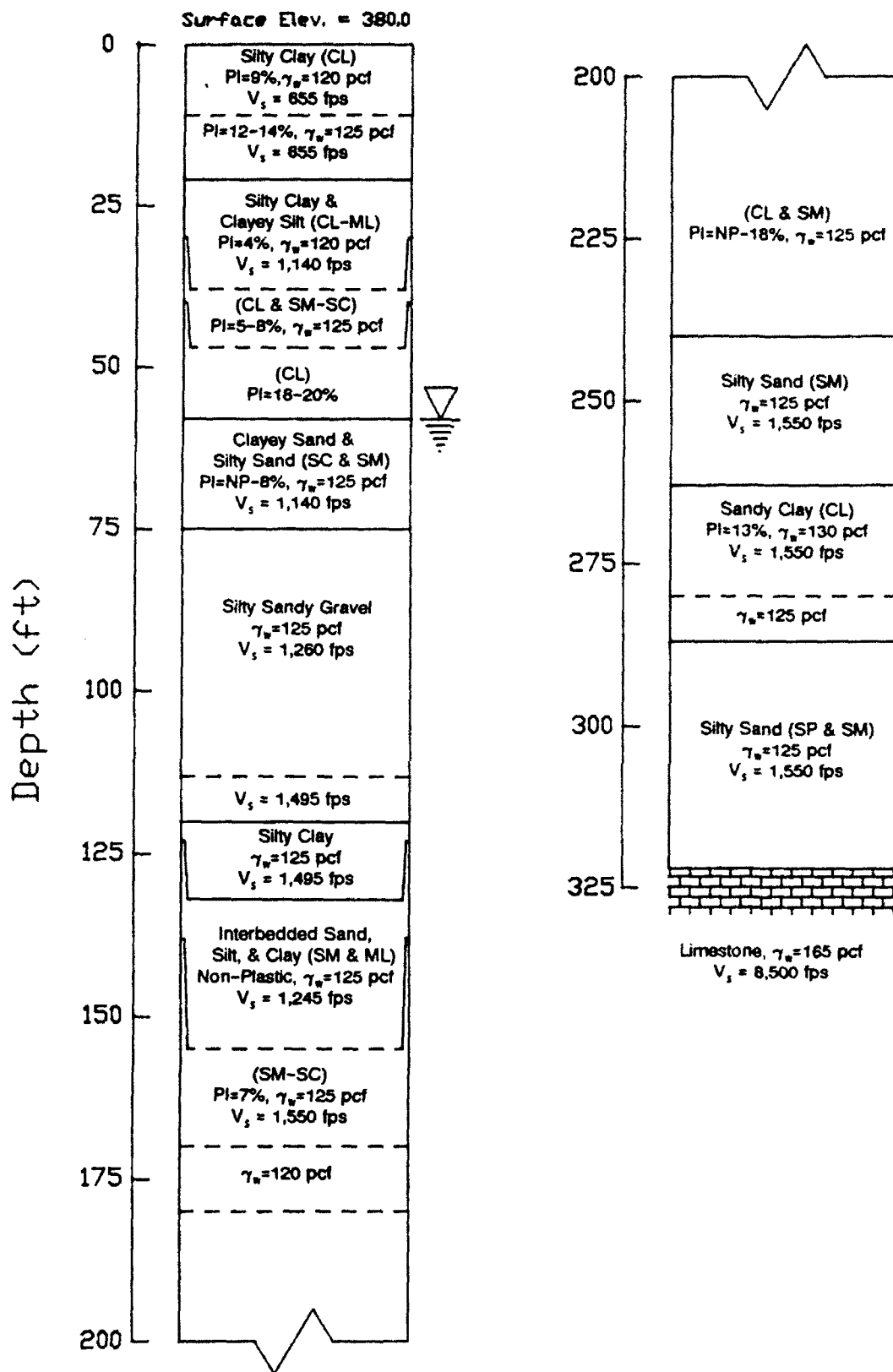
Figure 20. Soil column for Site 2
