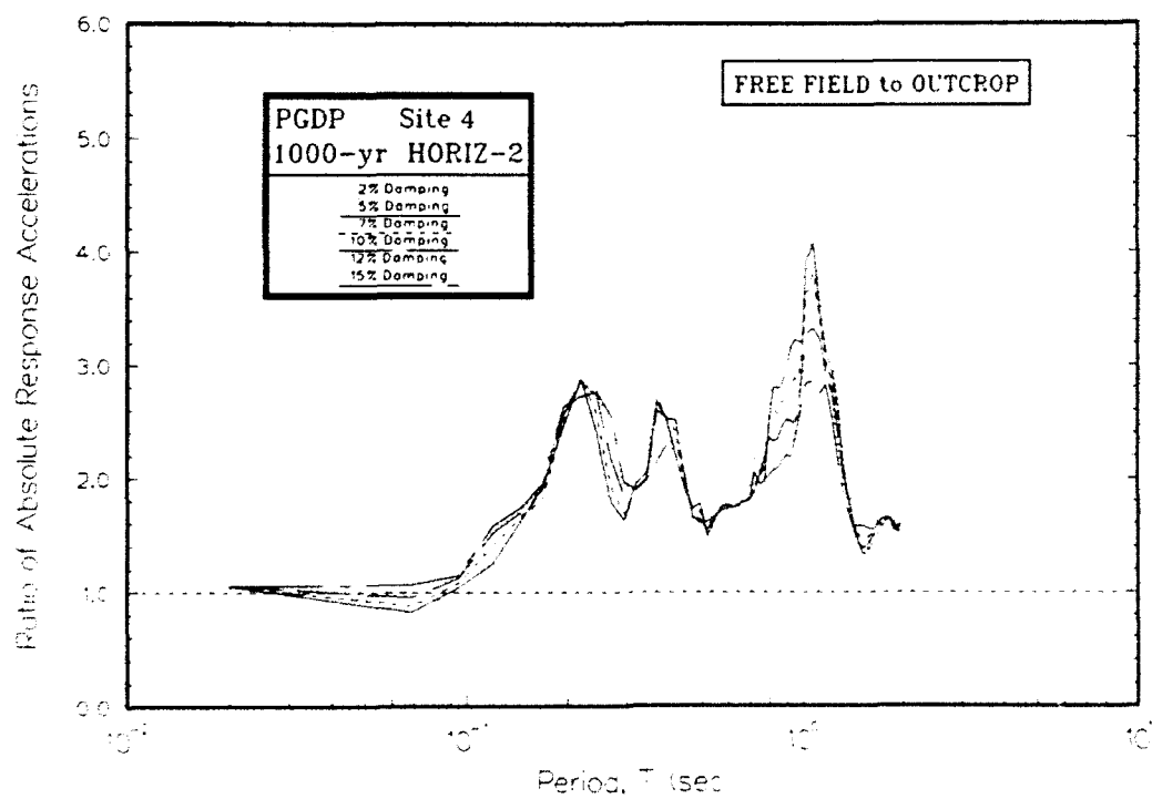
Figure L4. Ratio of absolute acceleration response spectra at free field to rock for Site 4
