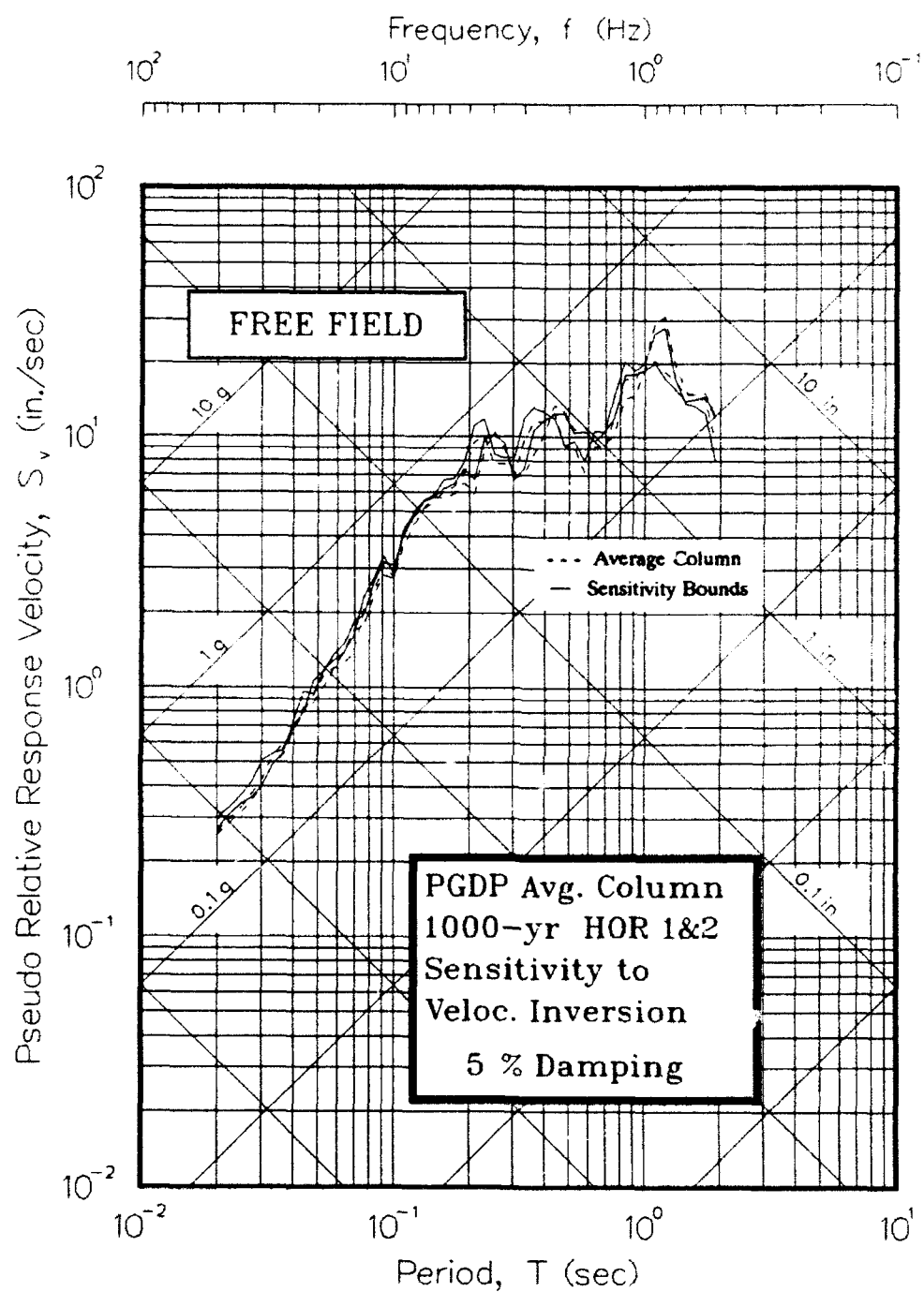
Figure 53. Pseudo-velocity response spectra showing sensitivity of results to shear wave velocity inversion
