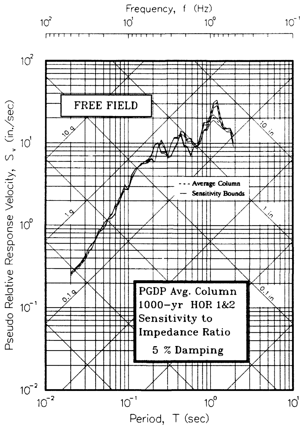
Figure 55. Pseudo-velocity response spectra showing sensitivity of results to impedance ratio
