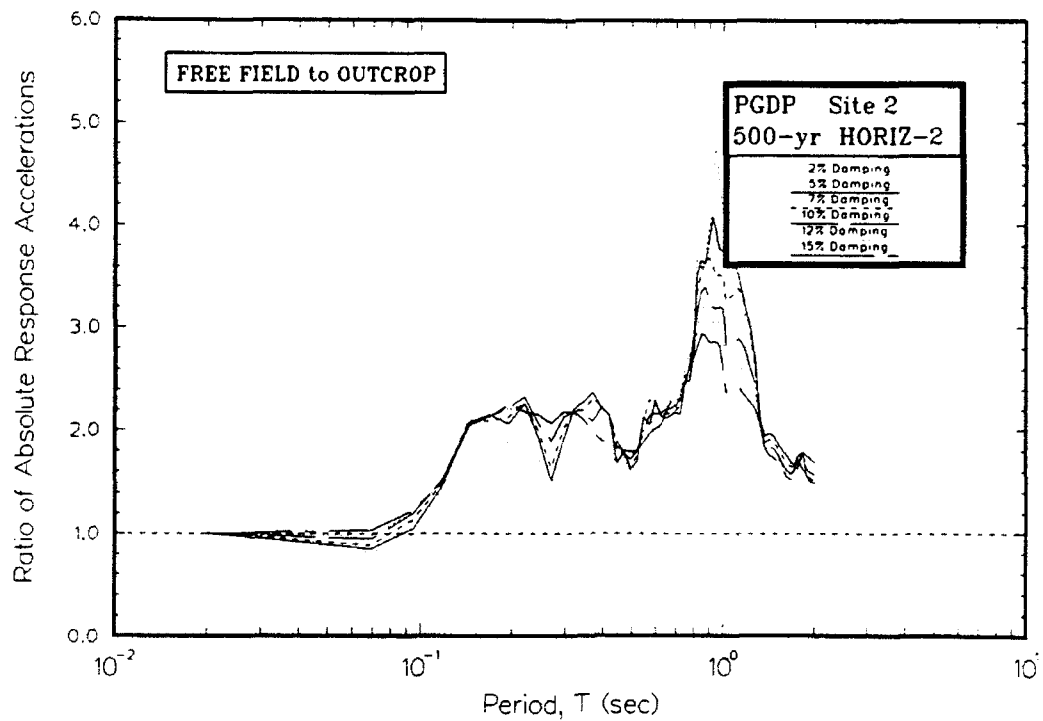
Figure F2. Ratio of absolute acceleration response spectra at free field to rock for Site 2
