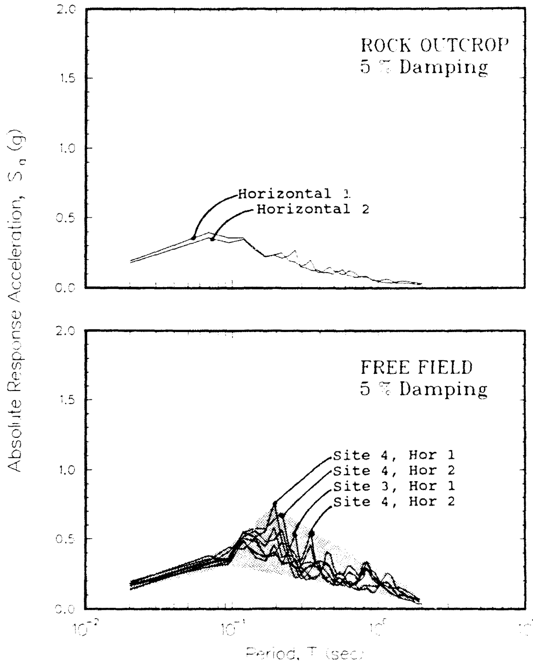
Figure 40. Absolute response acceleration spectra for 500-year event
