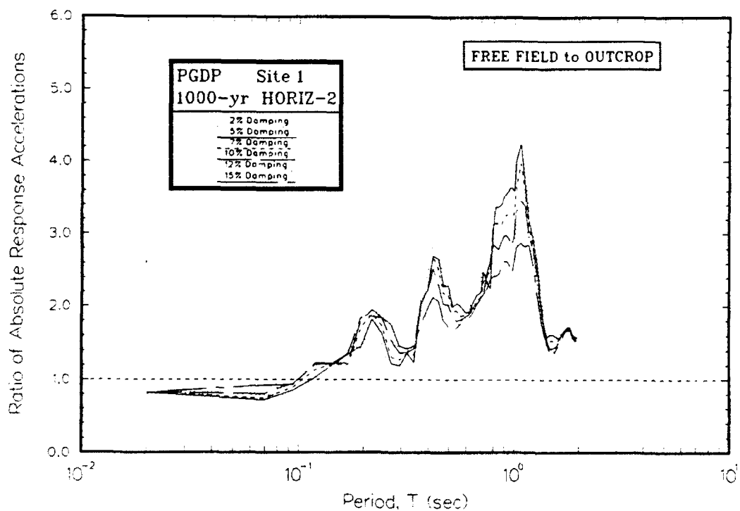
Figure L1. Ratio of absolute acceleration response spectra at free field to rock for Site 1
