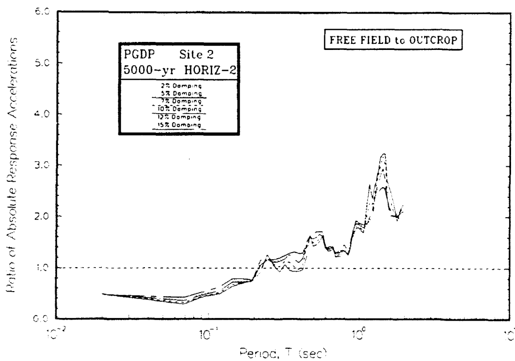
Figure R2. Ratio of absolute acceleration response spectra at free field to rock for Site 2
