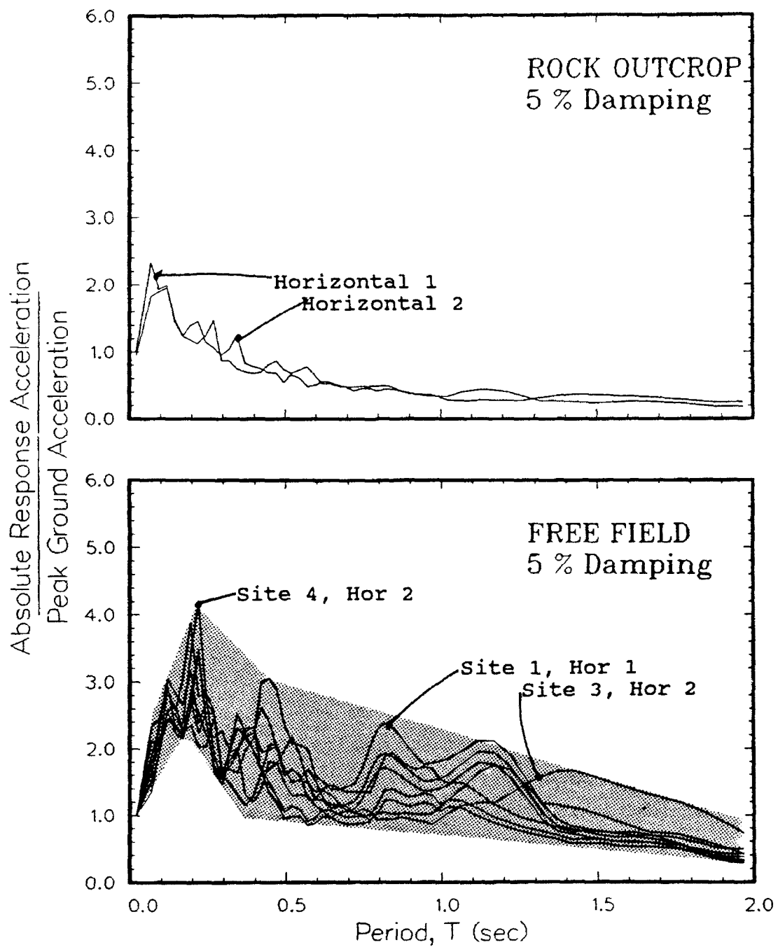
Figure 46. Amplification ratio for 1000-year event
