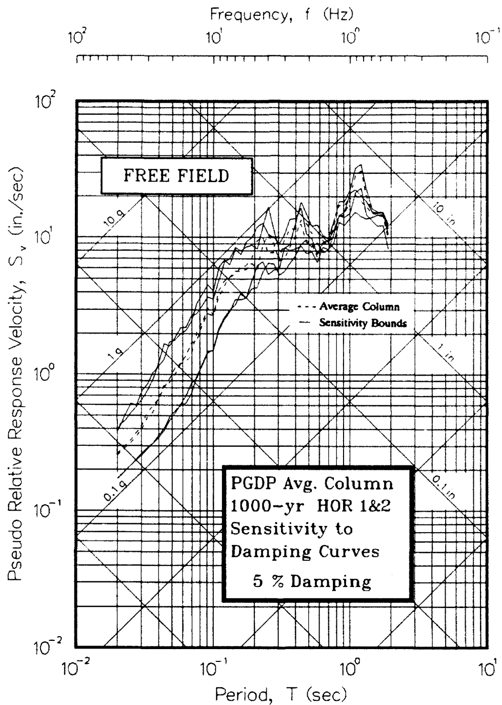
Figure 57. Pseudo-velocity response spectra showing sensitivity of results to damping ratio curves
