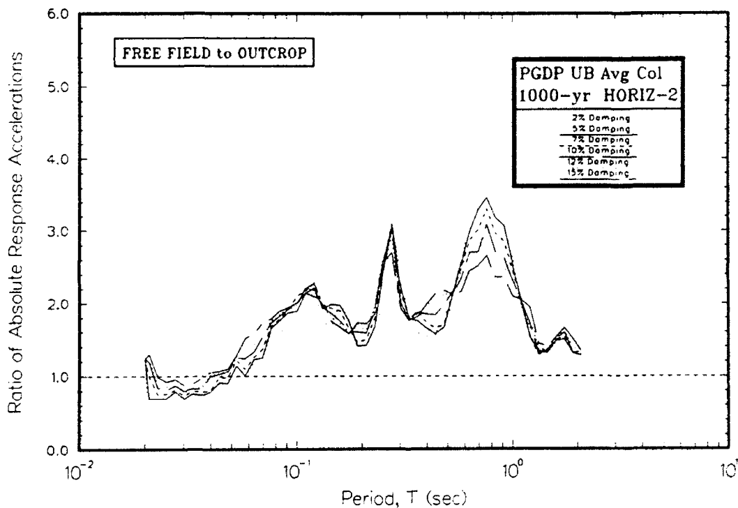
Figure U15. Ratio of absolute acceleration response spectra at free field to rock using upper bound of modulus for average column
