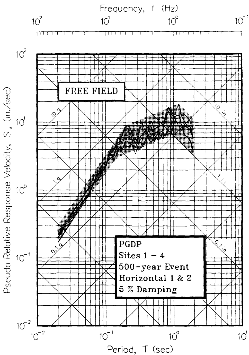
Figure 39. Pseudo-velocity response spectra for 500-year event
