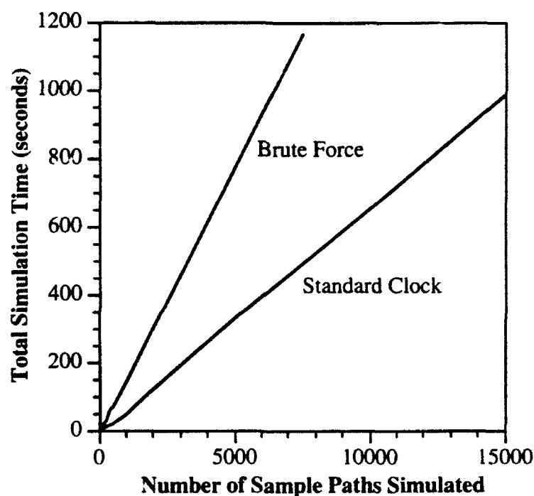
Fig. 12 — Time required to perform SC and BF simulations of the circuit-switched voice network
