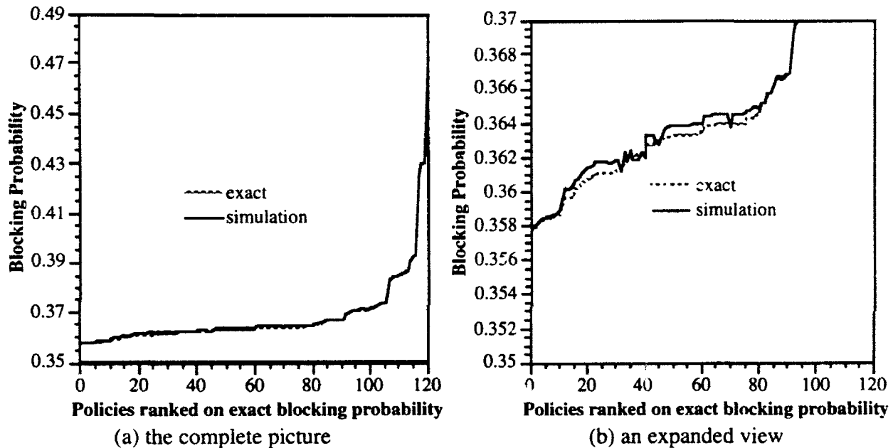
Fig. 14 — Probability of blocking across the range of policies; \rho^V = 4 , simulation duration = 10^6 voice arrival events
