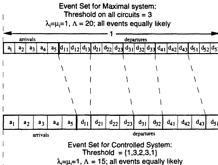
Fig. 11 — Ratio yardsticks showing event sets for the circuit-switched network
