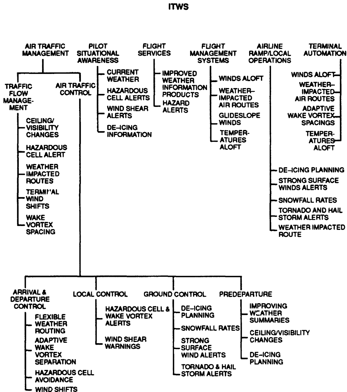
Figure 34. Terminal area operations supported by ITWS.
