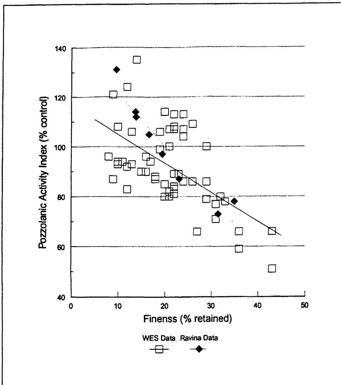
Figure 2. Effect of fineness (% retained on a 45\mu sieve) on pozzolanic activity index
