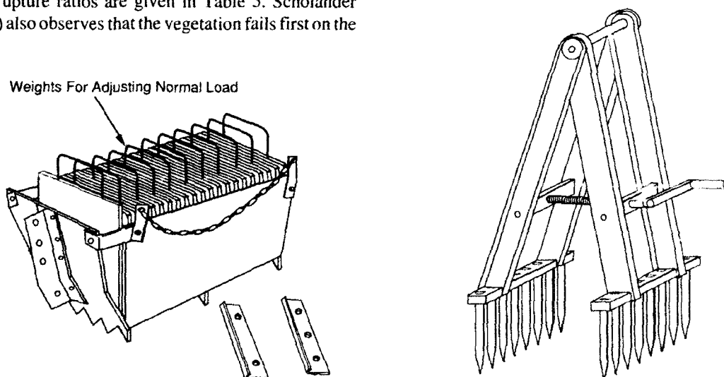
Figure 17. Instruments used by Niemi and Bayer (1970) to measure (a) shear resistance and (b) tensile strength of the vegetation mat.
