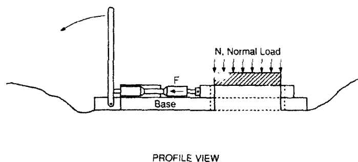
Figure 9. In situ direct shear apparatus.
