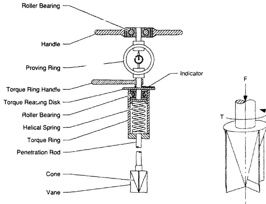
Figure 4. Vane-cone (after Yong and Youssef 1978).
