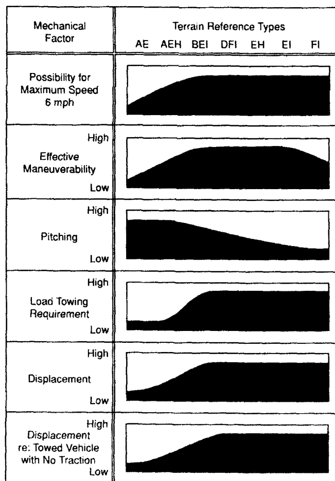
Figure 14. Vehicle performance on seven common muskeg terrains (after Radforth and Evel 1959).
