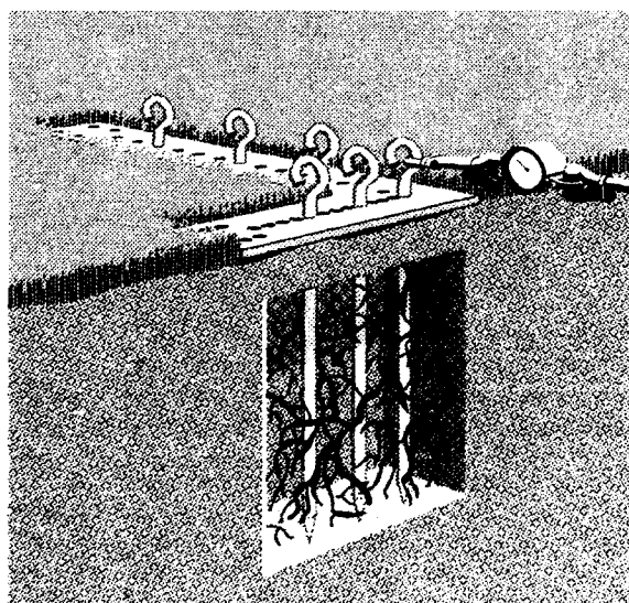
Figure 16. The muskeg fluke (from MacFarlane 1969).
