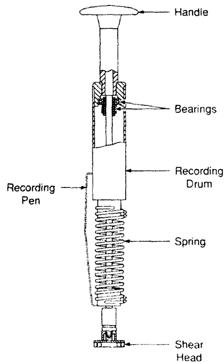
Figure 5. Cohron sheargraph (after Karafiath and Nowatzki 1978).
