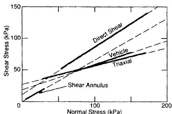
Figure 12. Yield envelopes on silty sand for different test methods (after Shoop 1989).
