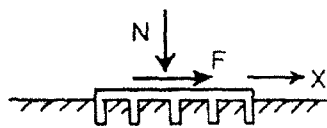
Figure 8. Grouser shear plate.
