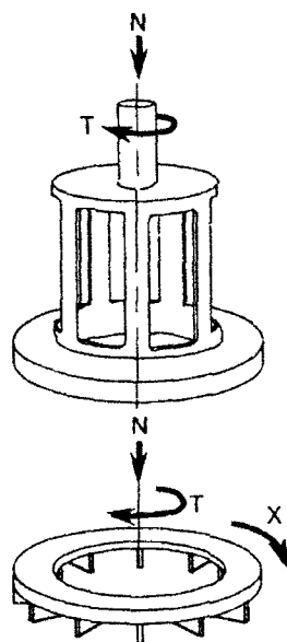
Figure 6. Shear annulus.
