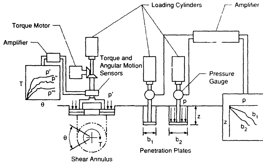
Figure 2. Components of a bevameter (after Bekker 1969).
