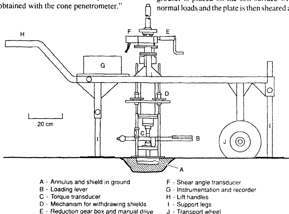
Figure 7. Portable shear annulus (after Stafford and Tanner 1982).
