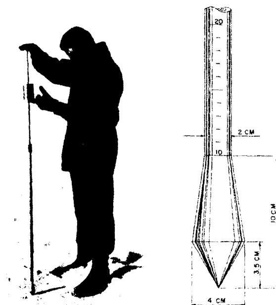
Figure 22. Rammsonde penetrometer (after Abele 1990).
