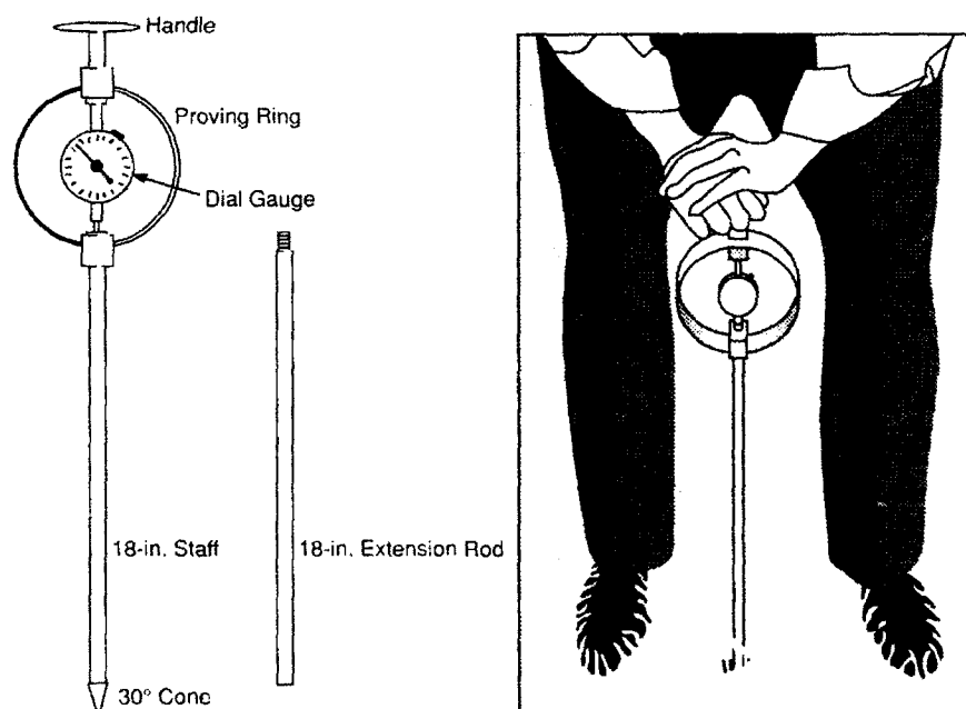
Figure 1. Hand-held cone penetrometer (after ASAE 1985, SAE 1967).
