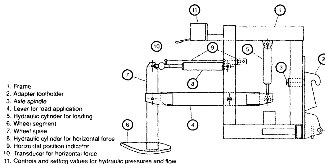
Figure 10. Wheel arc test rig (after Wasterlund 1990).
