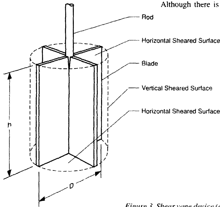
Figure 3. Shear vane device (after Kogure et al. 1988).
