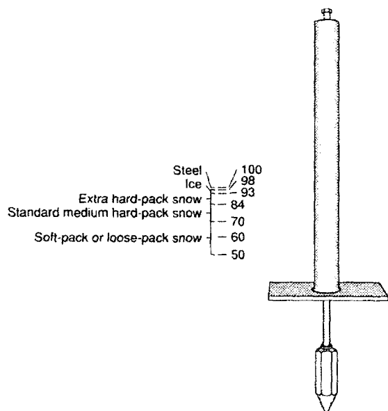
Figure 21. Snow compaction gauge, also called a drop cone (after SAE 1985).
