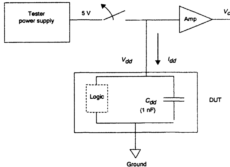
Figure 2. Keating circuit.
