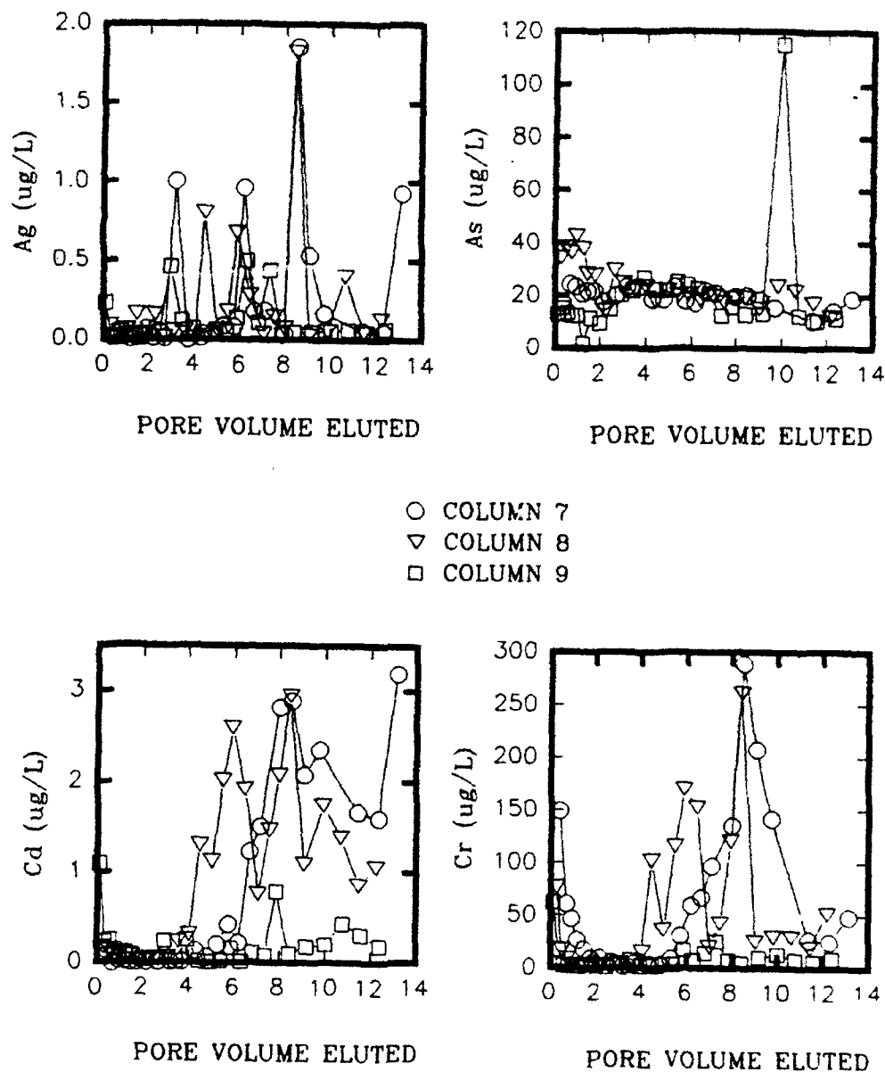
Figure V-12. Silver, arsenic, cadmium, and chromium elution curves
