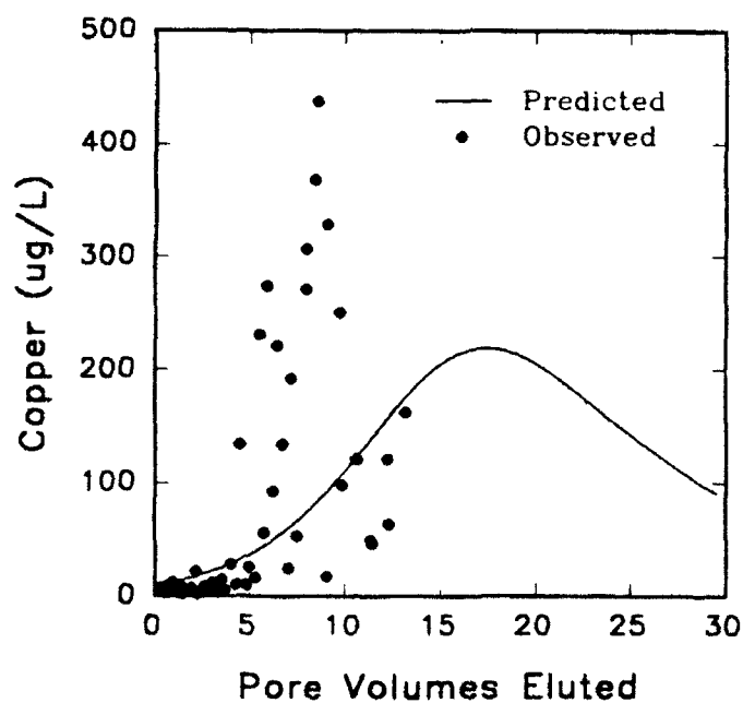
Figure V-20. Predicted and observed elution curves for cadmium and copper
