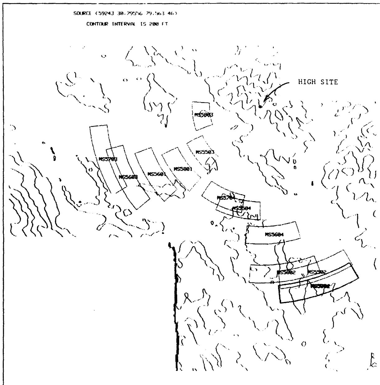
Figure 1. MSFD radar test high site data coverage
