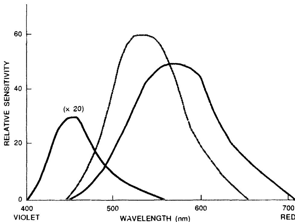
Fig. 8 — Response characteristics of the eye (Fig. 17.16 from Overheim and Wagner (1982))
