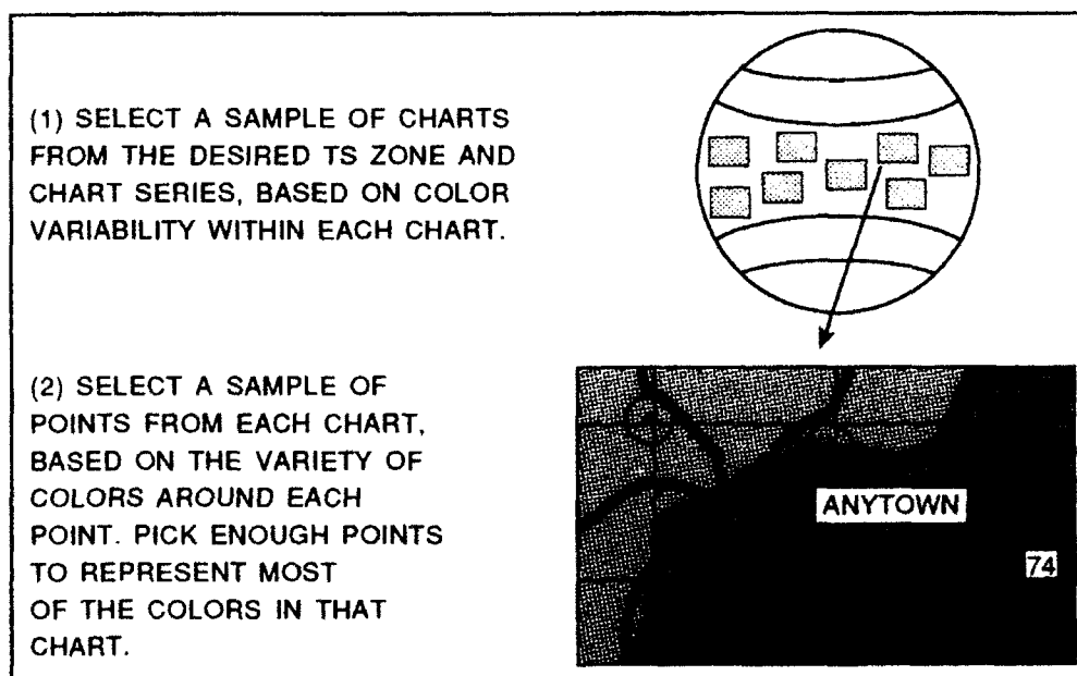
Fig. 4 — Sample chart and point selection for median-cut palette
