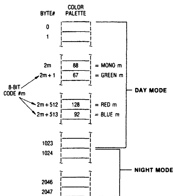
Fig. 3 — CAC color palette file layout
