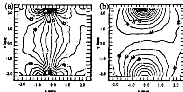
FIGURE 2. u_x (a) AND u_y (b) DISPLACEMENT COMPONENTS OF X-0344 UNDER LOAD IN THE BRAZILIAN TEST
