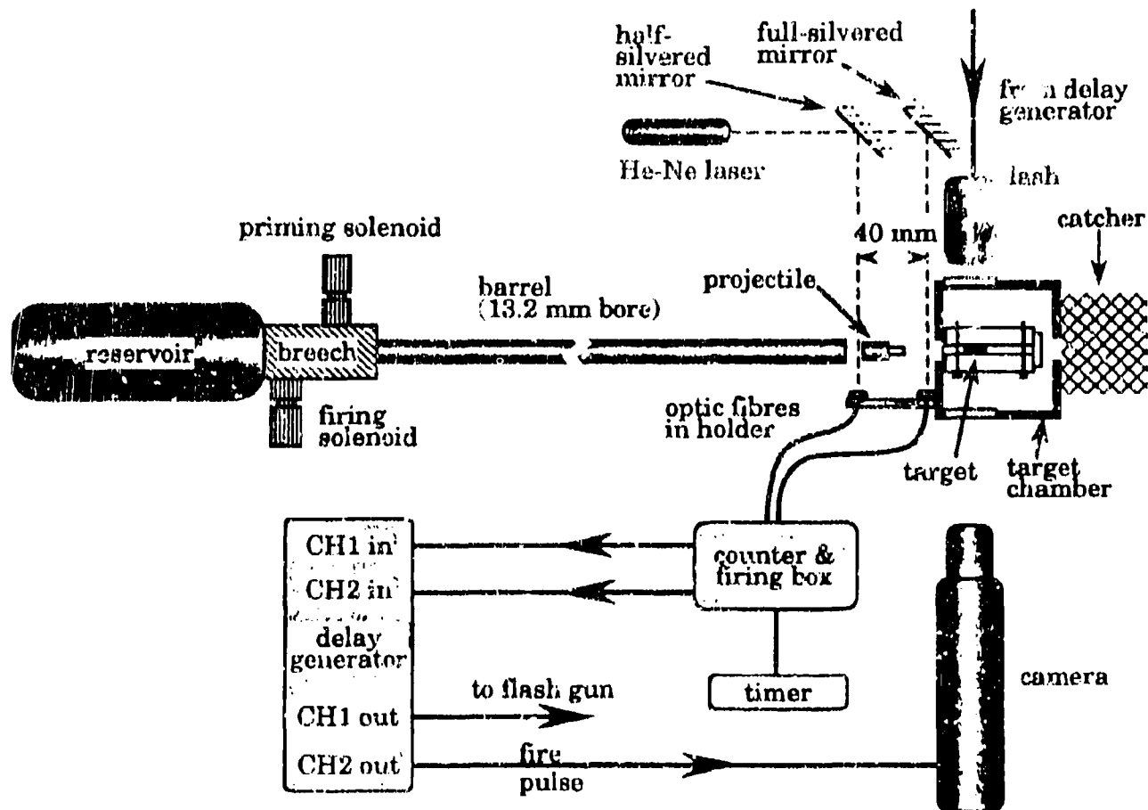
FIGURE 4. SCHEMATIC DIAGRAM OF THE EXPERIMENTAL ARRANGEMENT.
