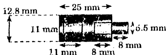
FIGURE 1. SCHEMATIC DIAGRAM OF THE SABOT-PROJECTILE COMBINATION.
