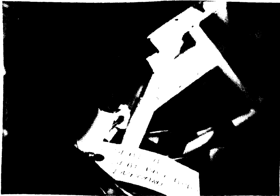
FIGURE 41. POST TEST SEAT 11, BROKEN SEAT BACK ATTACHMENT
