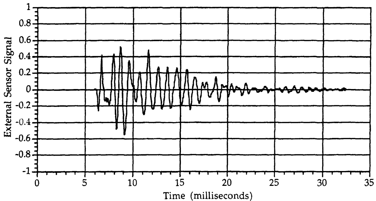
Figure 3.10b: Net Externally Measured Error Signal with Controller Operative and Imperfectly Subtracting the Coupling Model Signal
