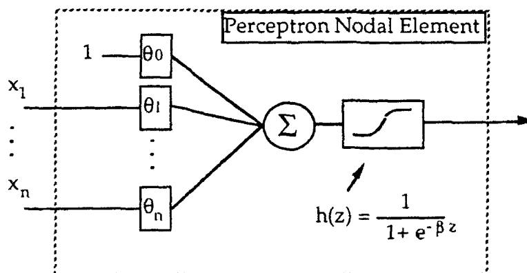
Figure A.6: An MLP Network Element
