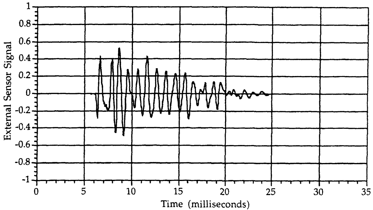
Figure 3.3b: Net Externally Measured Error Signal with Controller Operative Using Zero-Padded Measurement Data
