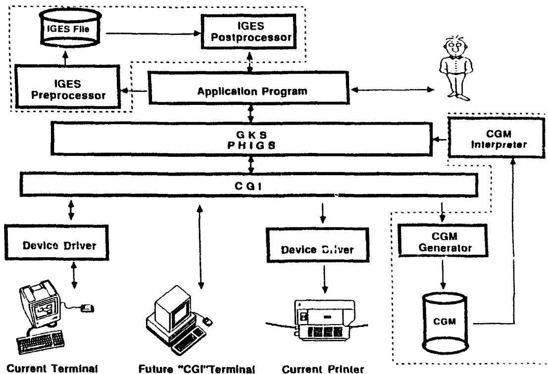
Figure 2. Standards in the Computer Graphics Reference Model
