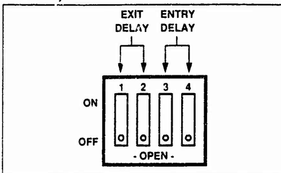
Figure 17. EXIT/ENTRY DELAY Switch
