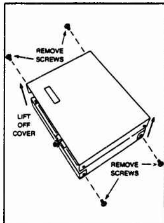
Figure 12. Removing the SSR-32 Case Cover
