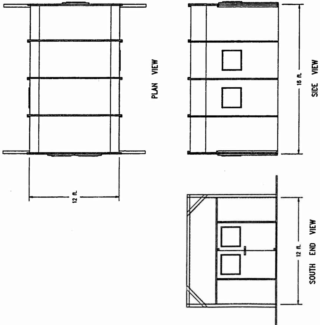
Figure B-3. Dimensions of Test Structure
