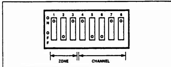
Figure 6. Example Channel Coding Switch
