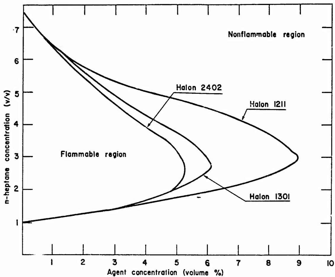
Figure A-1. Comparison of Halon Extinguishment Characteristics
