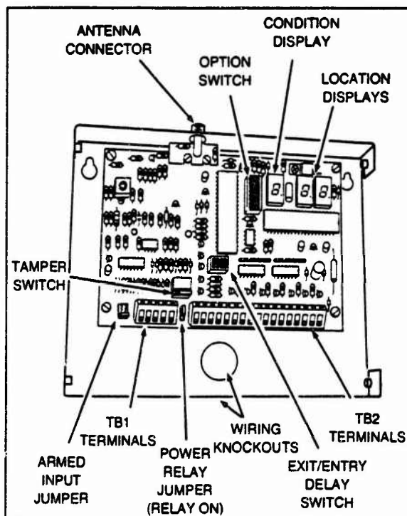
Figure 13. SSR-32 Circuit Board
