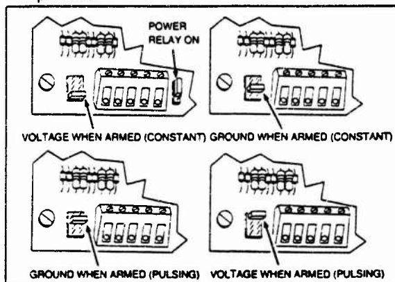
Figure 14. Armed Input Jumper Positions
