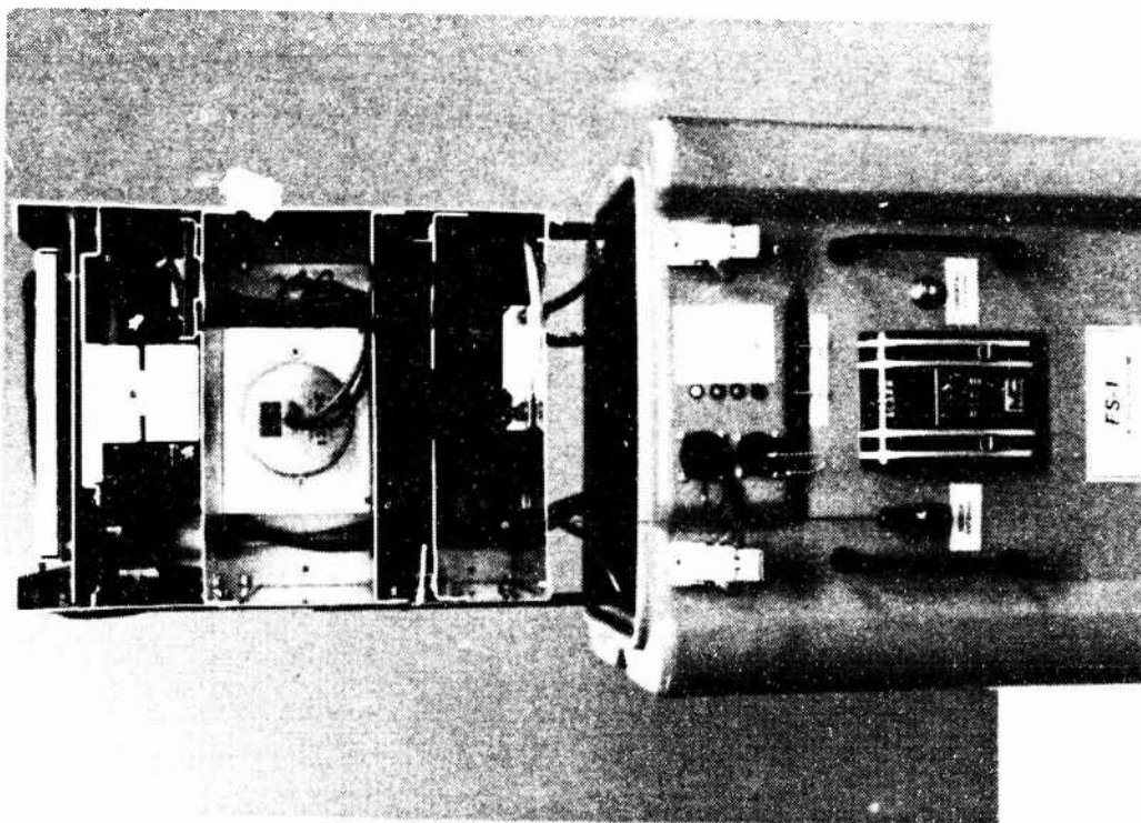
Figure C-4. Prototype AFS Equipment Rack in Extended Position
