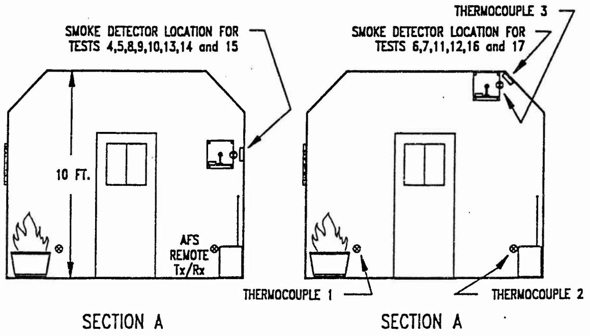
Figure C-A-1. Equipment Layout (Live Tests)
