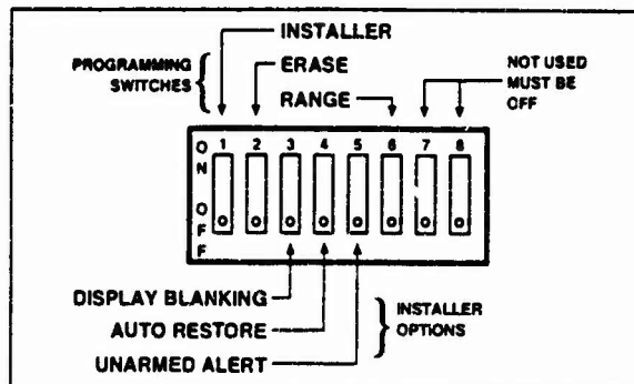
Figure 15. OPTION Switch
