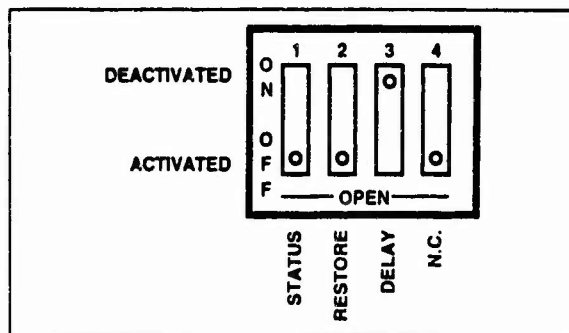
Figure 9. Typical MODE Switch Settings
