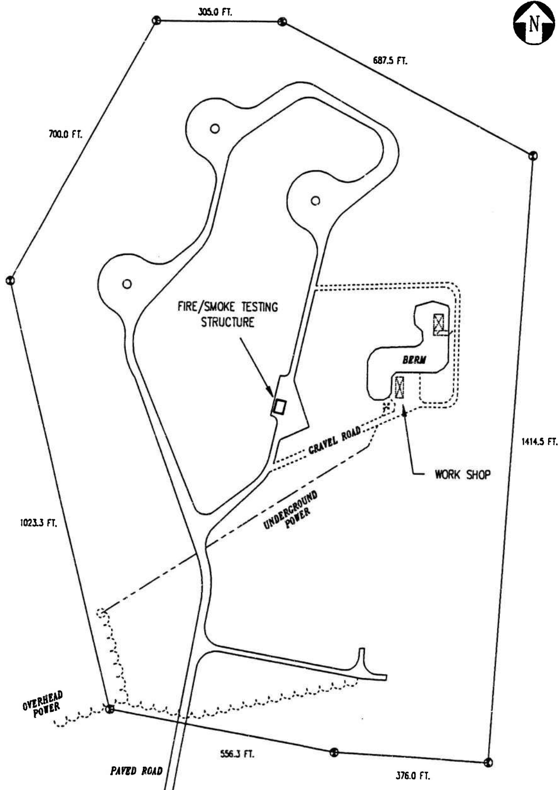
Figure B-2. Test Site Detail
