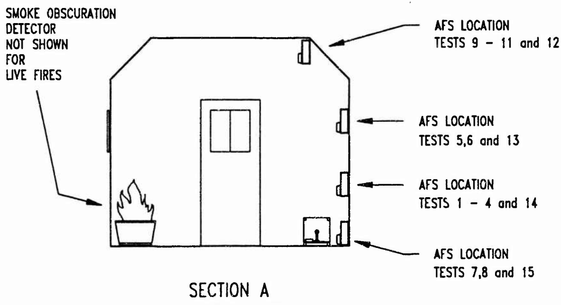
Figure B-10. Equipment Layout in Structure
