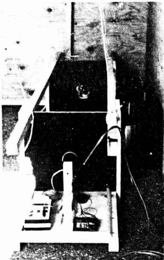
AFS Remote Unit Prior to Test at Floor Level
