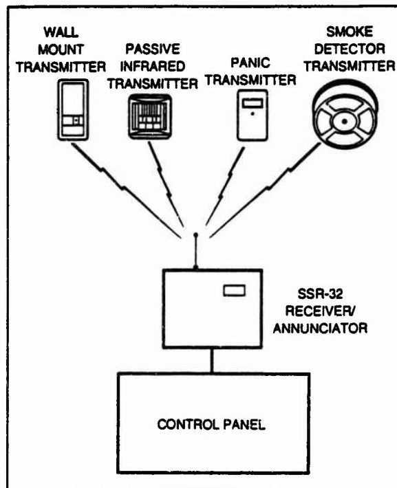
Figure 1. Typical Supervised System Configuration
