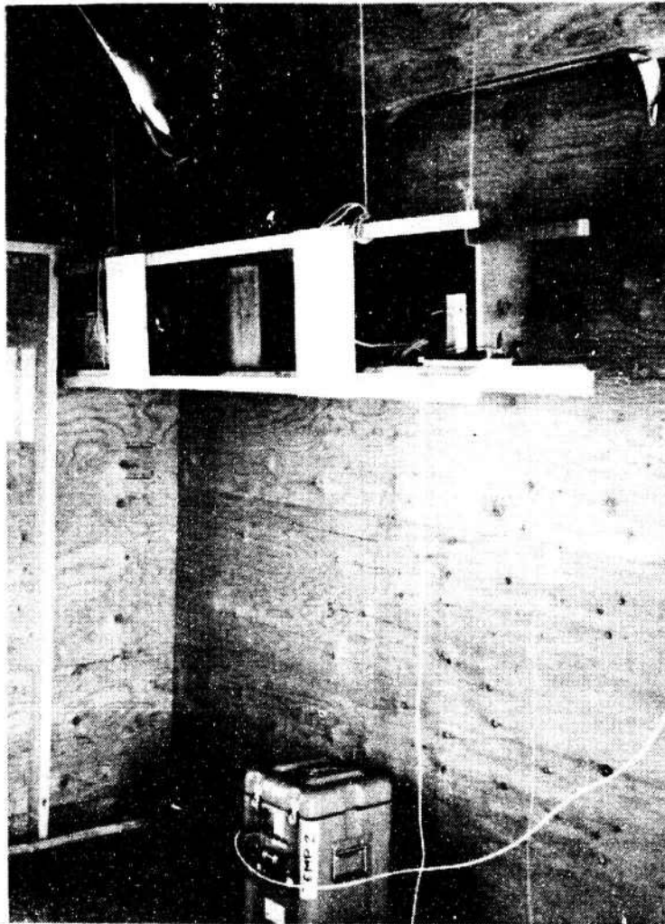
Figure C-5. Smoke Obscuration Detector Installed at 6 ft. Height in Test Structure
