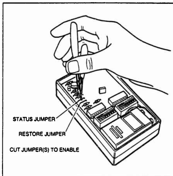
Figure 3. Cutting the ST-1 Status and Restore Jumpers
