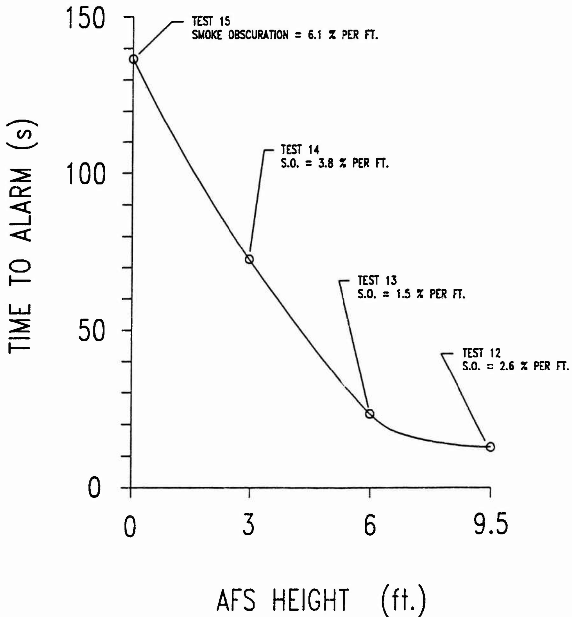
Figure B-26. Response Time and Obscuration vs. Height - Fire Tests
