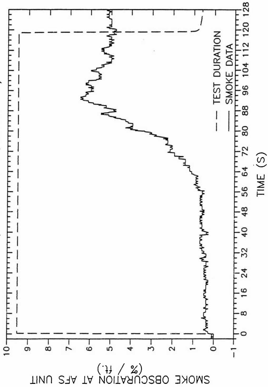
Figure B-11. Smoke Obscuration Near AFS vs. Time - Test 3
