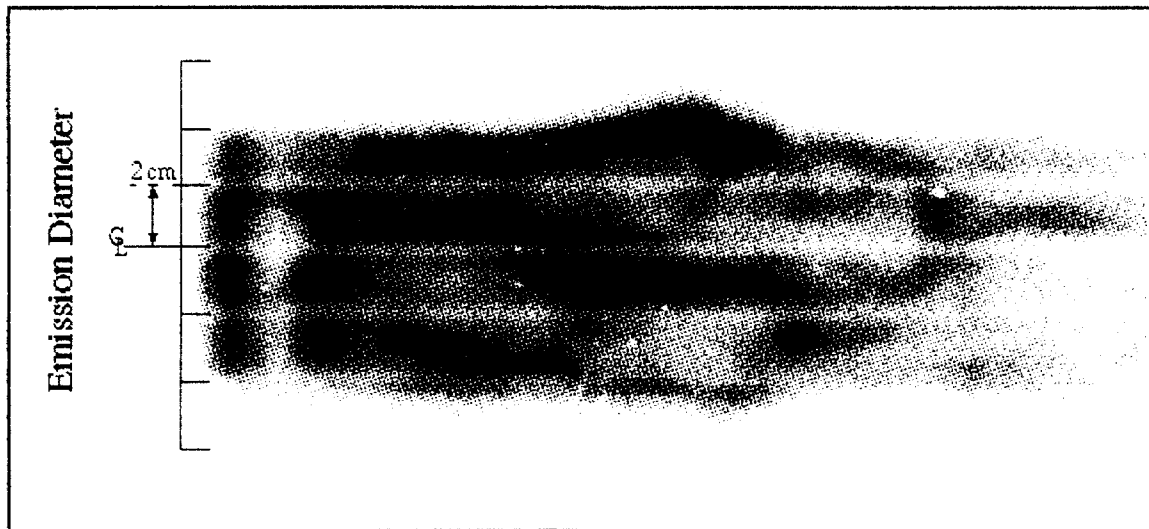
Figure 6. Streak photograph showing the emitted beam diameter from a 4.6 cm radius CsI cathode.
