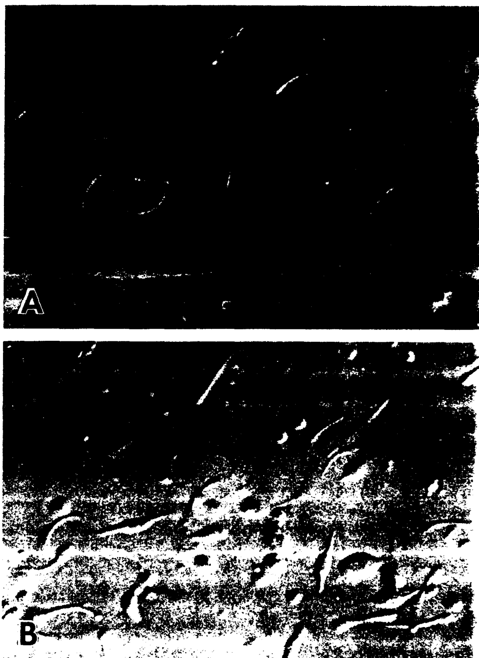
FIGURE 3. A, appearance of normal, mature sperm of Lutzomyia longipalpis . B, the typical appearance of the abnormal sperm produced by intercolony F_1 hybrid males, in this case the product of a cross between a Brazil female and a Colombia male. (Magnification \times \times 2,000 .)
