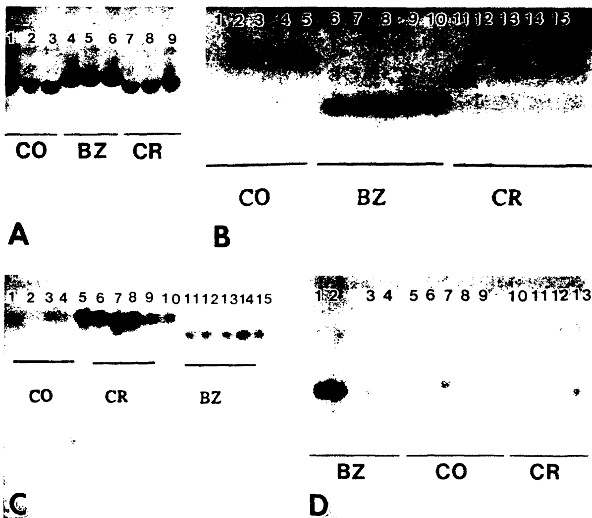
FIGURE 2. Gels illustrating the phenotypes of certain diagnostic loci for species in the Lutzomyia longipalpis complex. A, malic enzyme (ME). Lanes 1-3 and 7-9 are ME 100 homozygotes and lanes 4-6 are ME 125 homozygotes. B, mannose phosphate isomerase (MPI). Lanes 1-5 are MPI 100 homozygotes, lanes 6-8 are MPI 125 homozygotes, lanes 9 and 10 are MPI 100 /MPI 125 heterozygotes, lane 11 is an MPI 100 homozygote, lane 12 is an MPI 125 homozygote, lane 13 is an MPI 100 homozygote, lane 14 is an MPI 100 homozygote, and lane 15 is an MPI 100 homozygote. C, glutamate oxaloacetate transaminase-1 (GOT-1). Lanes 1-10 are GOT 100 homozygotes and lanes 11-15 are GOT 125 homozygotes. D, peptidase-1 (PEP-1). Lanes 1-4 are PEP-1 100 homozygotes, lanes 5-9 are PEP-1 100 homozygotes, lanes 10-12 are PEP-1 100 homozygotes, and lane 13 is a PEP-1 100 /PEP-1 125 heterozygote (the products of the peptidase-2 locus can be seen as faint bands towards the top of the gel). CO = Colombia; BZ = Brazil; CR = Costa Rica.
