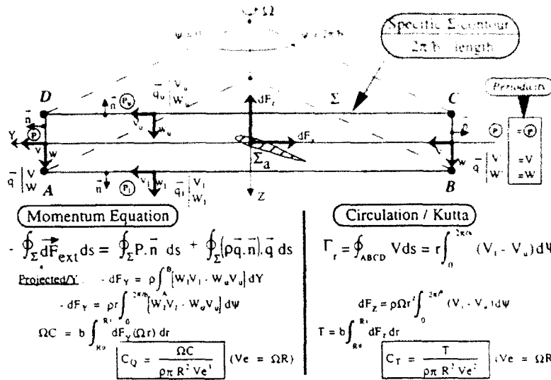
Fig. 2. - Momentum Equation Applied to Specific Contour for Hovering Rotor
