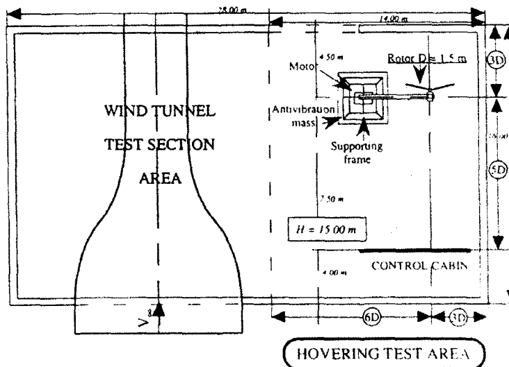
Fig. 3. - Hover Test Rig Installation at SI-Luminy
