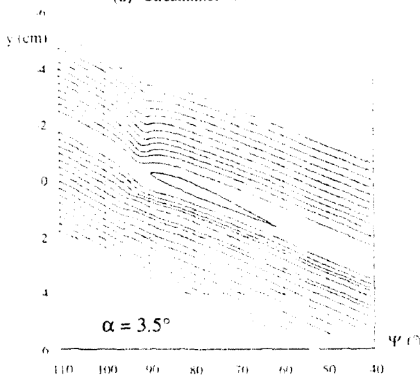
(b) Streamlines at r/R=0.75
