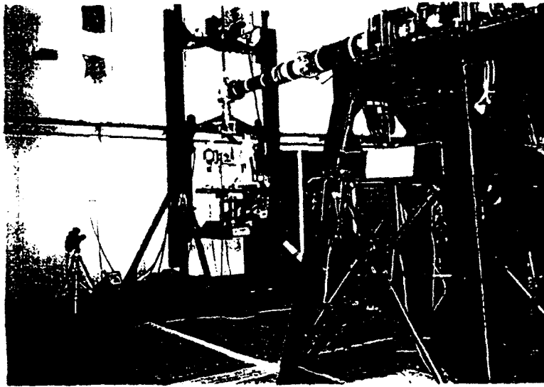
Fig. 4 - Model Rotor and Hover Test Rig at SI-Luminy Test Hall
