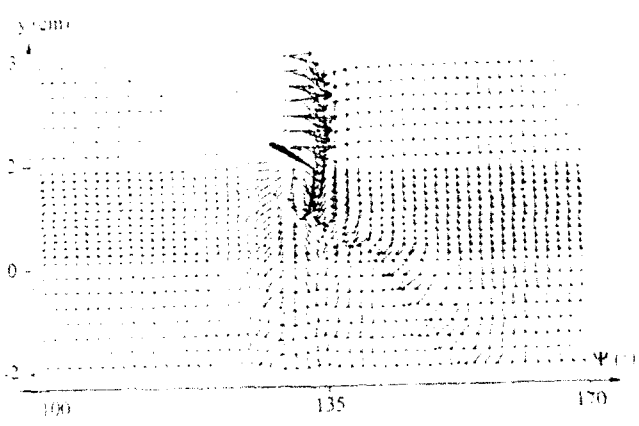
Fig. 13 - Induced Velocity Field at r/R=0.75
