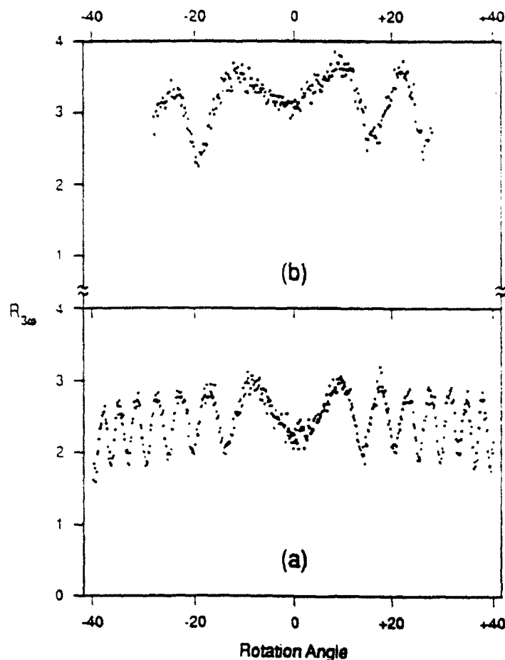
FIGURE 2 Maker Fringe Patterns for a nematic solution of PBT, with parallel polars and the incident polarization parallel to the director arrangement V-v-V (a) and H-h-H (b).
