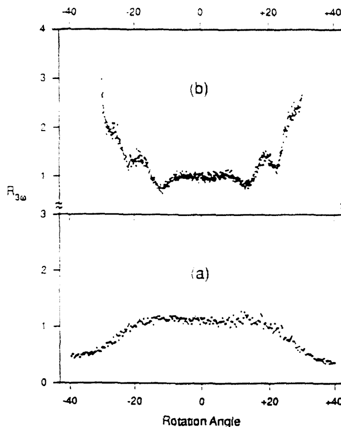
FIGURE 3 Maker Fringe Patterns for a nematic solution of PBT, with crossed polars and the incident polarization parallel to the director arrangement H-v-V (a) and V-h-H (b).
