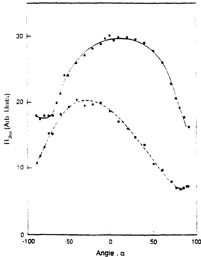
FIGURE 4 The parameter R_0(0,L) determined with vertical director, vertically polarized incident light and analyzer at angle \alpha to the polarizer for sample thickness L=385 \mu\text{m} (top curve), and L=438 \mu\text{m} (bottom curve).
