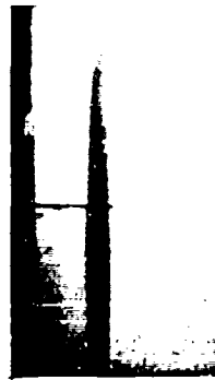
Figure 30. Flash X-Ray of Flyer Plate With Uniform Pressure Distribution Across the Back Surface of the Plate
