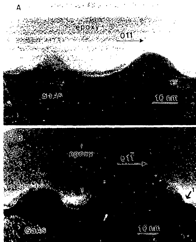
Fig. 3 : Shows coherent and incoherent islands of \text{In}_{0.5}\text{Ga}_{0.5}\text{As} on \text{GaAs} (1-0) in the 3-D island growth mode.
