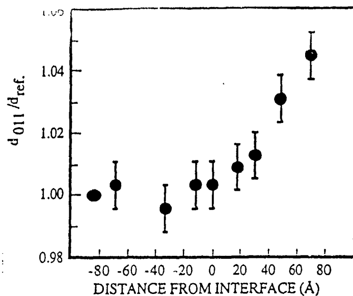
Fig. 5 : Plot of measured (011) interplanar spacing versus distance from the interface for a coherent island. The interplanar spacing is normalized to the lattice parameter value measured 84 Å below the interface in the substrate ( d_{ref} )
