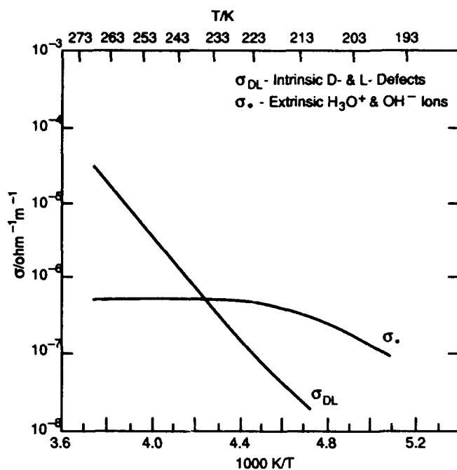
Figure 39. Temperature dependences of \text{H}_3\text{O}^+ ion conductivity \sigma_e and Bjerrum defects' conductivity \sigma_{DL} calculated from experimental results, using best-fit method. Ice doped by HF in the concentration of (1.3 \pm 0.1) \times 10^{20} molecules/ \text{m}^3 (after Camplin et al. 1978).
