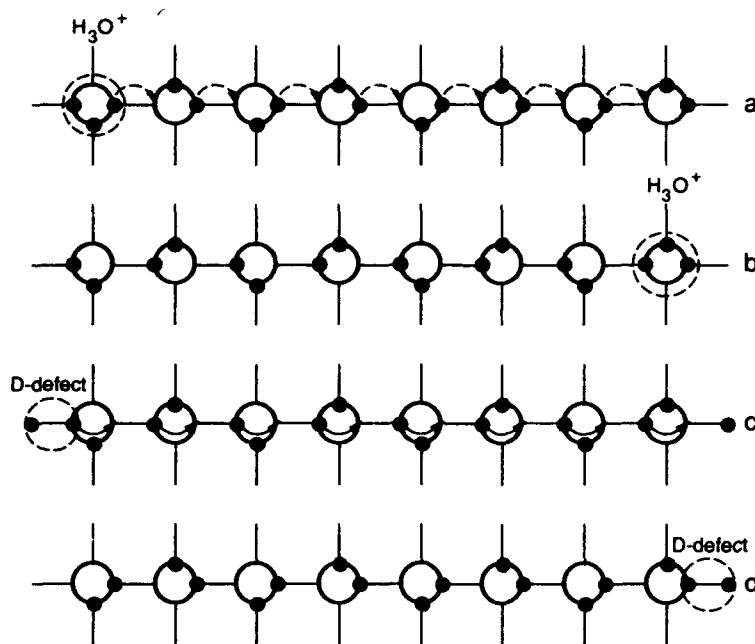
Figure 7. Schematic representation of \text{H}_3\text{O}^+ ion (a, b) and D-defect (c, d) motion along a chain of hydrogen bonds in ice. a) Initial arrangement of \text{H}_3\text{O}^+ ion and water molecules in the chain before the ion moves from the left to the right. The arrows indicate successive proton hops (along the bonds) by means of which the ion moves. b) The chain after the ion has passed. Obviously, no one \text{H}_3\text{O}^+ ion can go along the same chain in the same direction. c) D-defect motion from left to right along the same chain. The arrows indicate successive hops of protons from one bond to the next. d) The chain after the D-defect has passed. Comparison with Figure 7a shows that the motion of D-defect restored positions of the protons along the chain. It is ready (or "open") now for the passage of another \text{H}_3\text{O}^+ ion.
