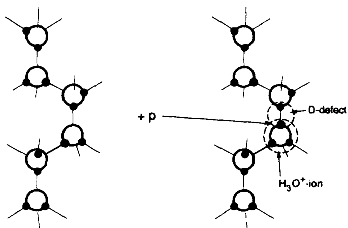
Figure 8. Creation of two point defects ( \text{H}_3\text{O}^+ ion and D-defect) when a proton is placed into a defect-free ice lattice.
