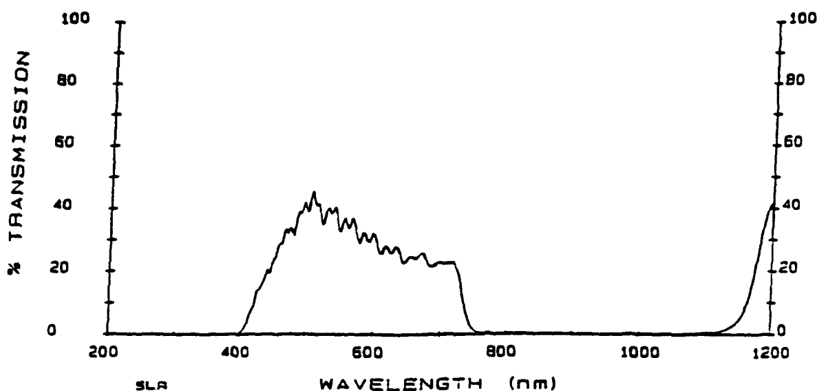
Figure 5. Spectral transmittance: SMLCS, open state, 0 degrees.
