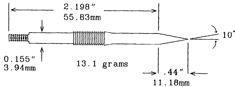
a. EM-launched tungsten penetrator.
