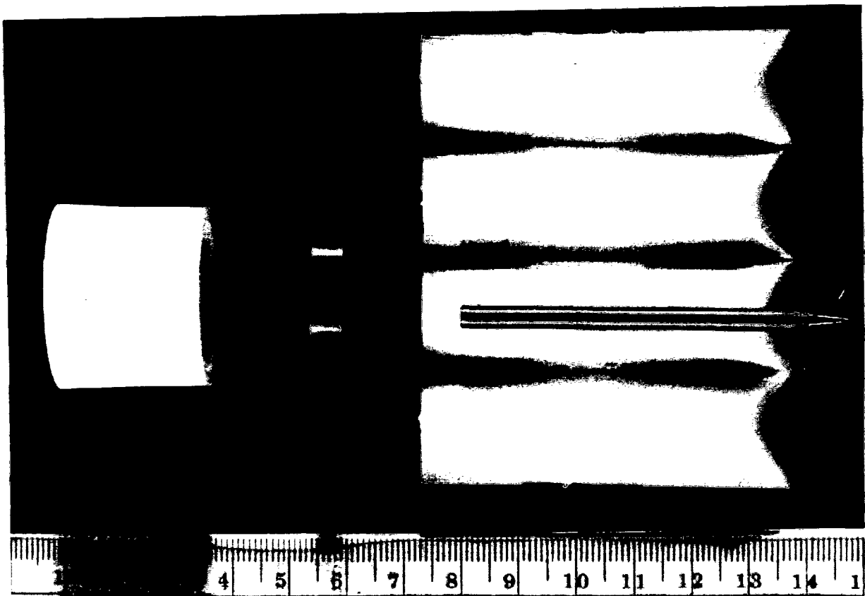
Figure 3. Terminal ballistic launch package with surrogate projectile.
