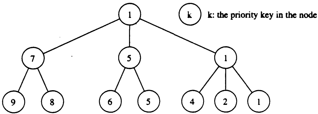
Figure 4.5: A 2-3 tree.
