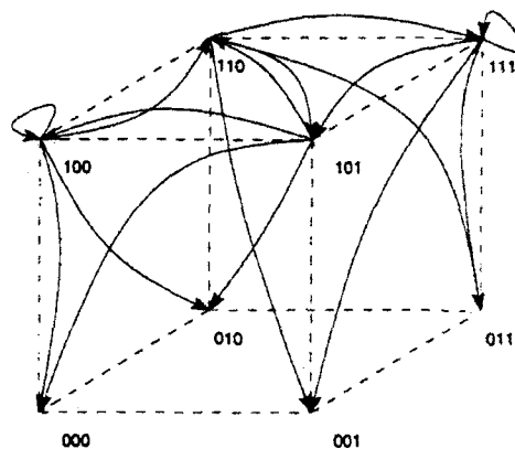
Figure 3.16: Transitions of "load" assertion.
