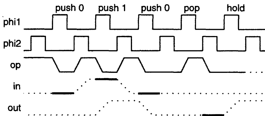
Figure 2.18: IO behavior of stack circuit. The time during which inputs must be stable, or during which outputs will be stable, is indicated by the heavy lines.
