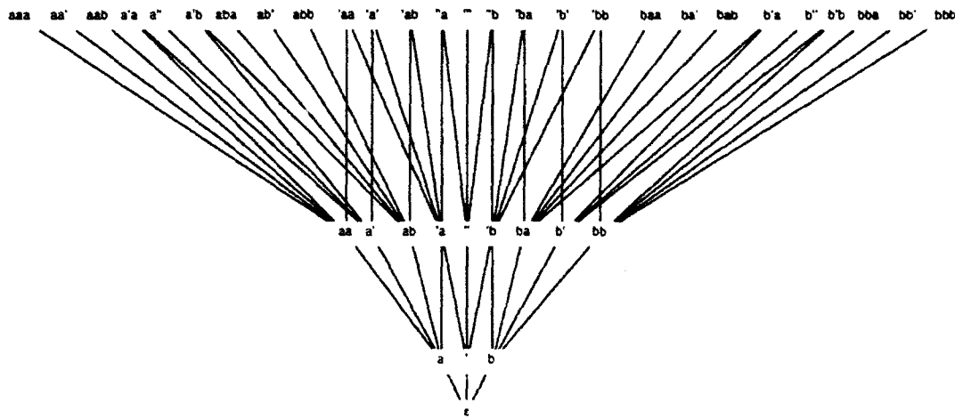
Figure A.3: Hasse diagram for the beginning of the marked prefix ordering for a two-symbol alphabet
