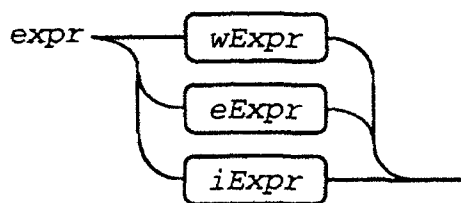
Figure 3.27: Syntax of general expressions. There are three possible kinds. A wExpr is a word-valued expression. A eExpr is an enumeration-valued expression. A iExpr is an integer-valued expression.
