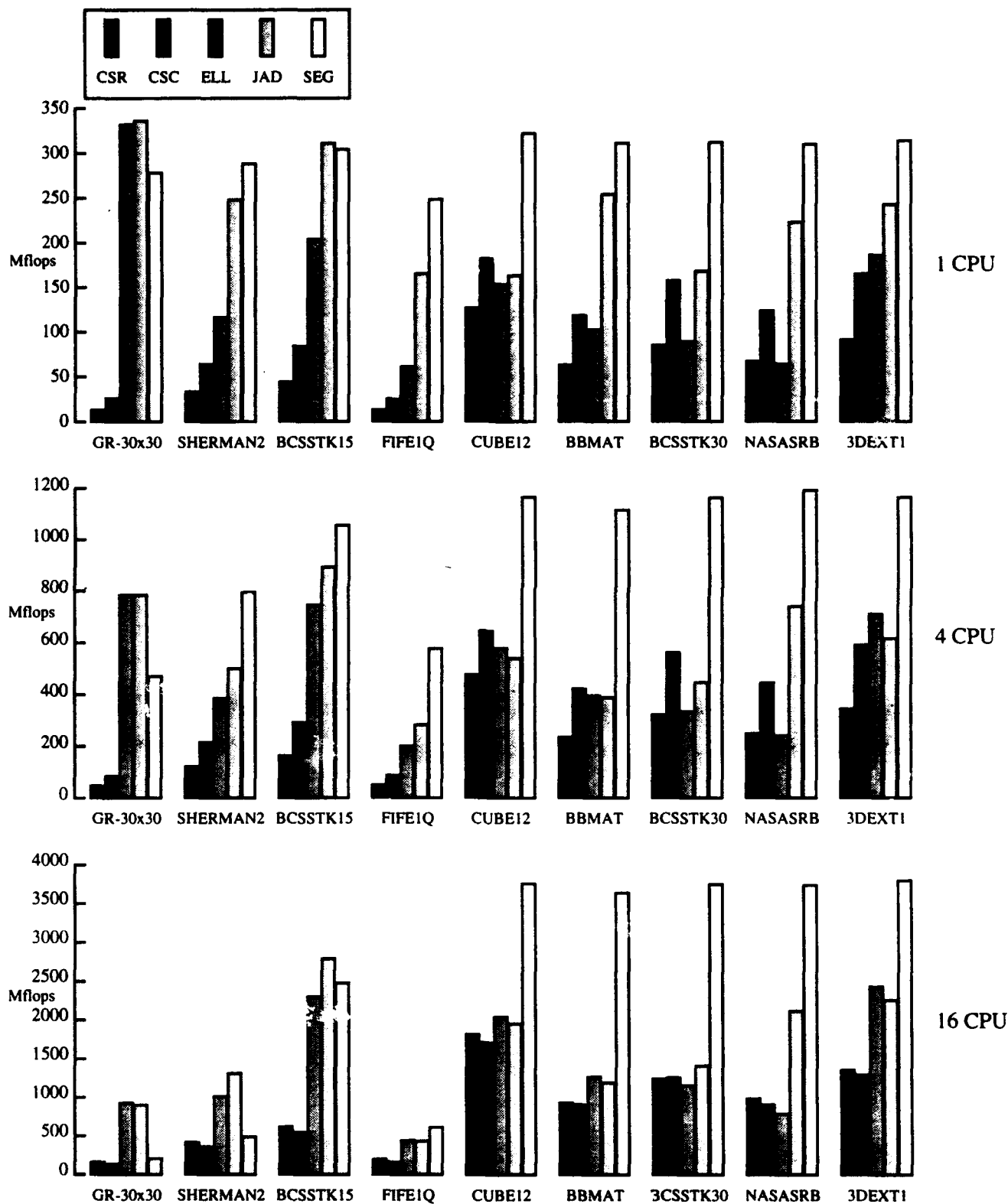
Figure 6: Performance results on a Cray Y-MP C90 comparing implementations of sparse matrix multiplication. The test matrices are shown in order of increasing number of non-zero entries. The SEGMV implementation outperforms all other implementations on the large test matrices.
