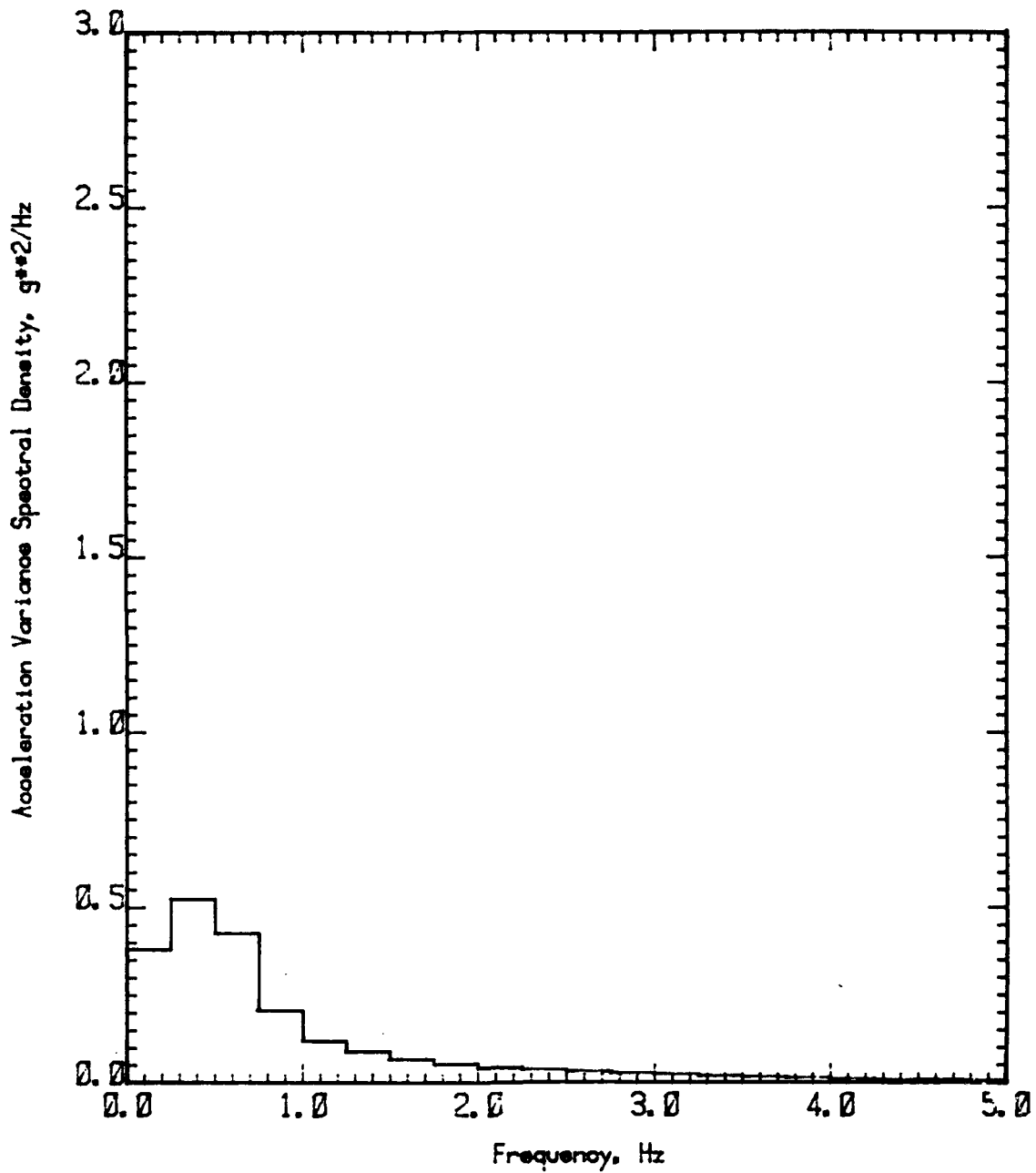
FIGURE A. 2.3 ACCELERATION VARIANCE SPECTRAL DENSITY 110 ft WPB Accelerometer No. 3 Speed Coefficient (CV) 3.00 Significant Wave Height 40.0% Beam
