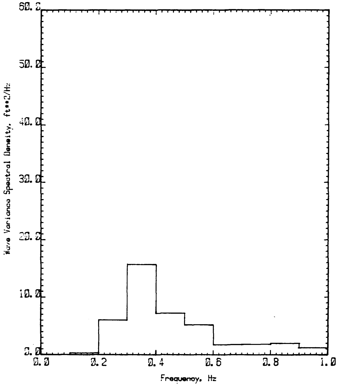
FIGURE I 1.2 WAVE VARIANCE SPECTRAL DENSITY 110 ft WPB Speed Coefficient (CV) 3.00 Significant Wave Height 40.0% Beam
