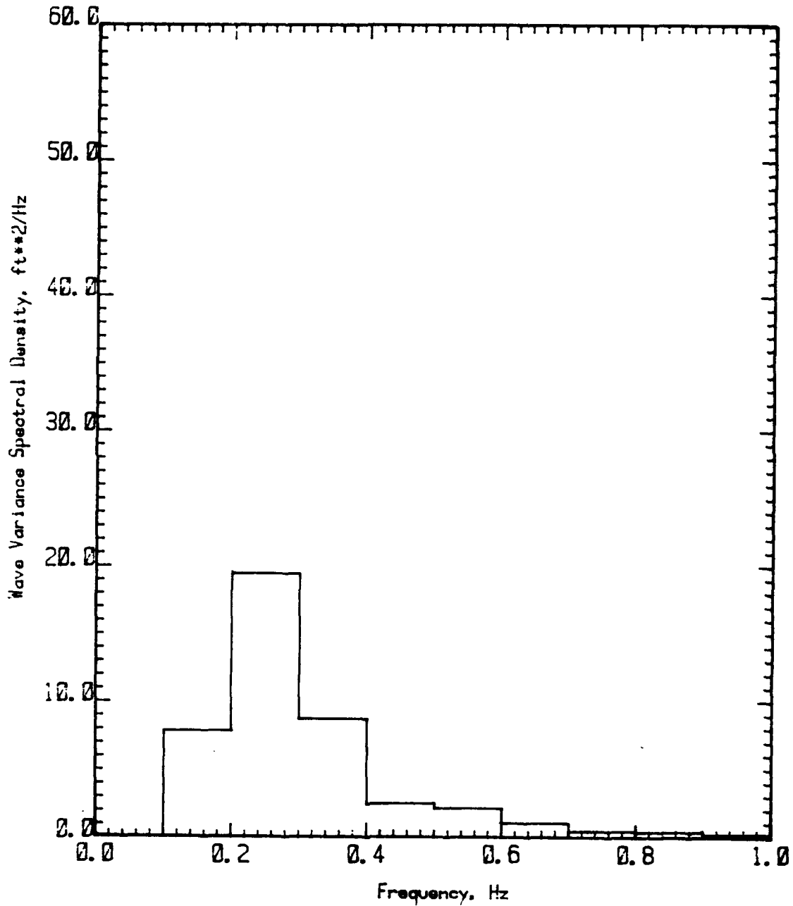
FIGURE I 1.1 WAVE VARIANCE SPECTRAL DENSITY 110 ft WPB Speed Coefficient (CV) 1.50 Significant Wave Height 40.0% Beam
