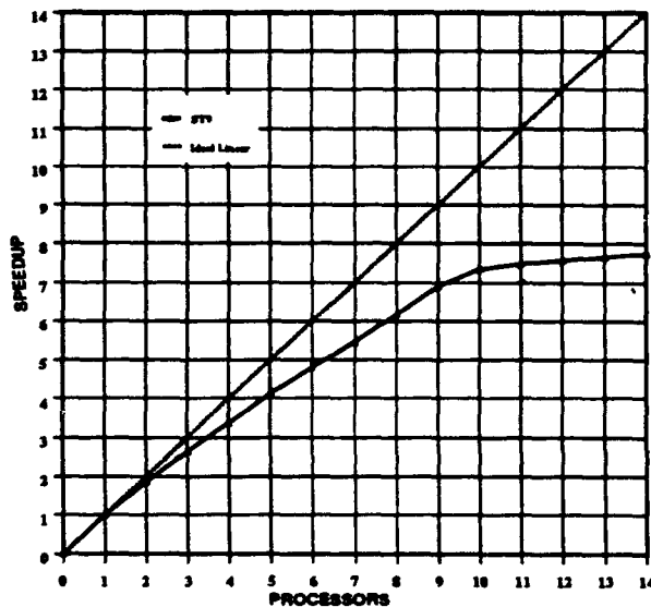
SPEEDUP VS PROCESSORS N-body Stormer Integrator
