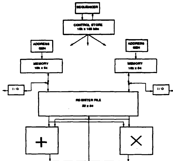
Figure 11: This is the overall architecture of a Supercomputer Toolkit processor node, consisting of a fast floating-point chip set, a 5-port register file, two memories, two integer alu address generators, and a sequencer.
