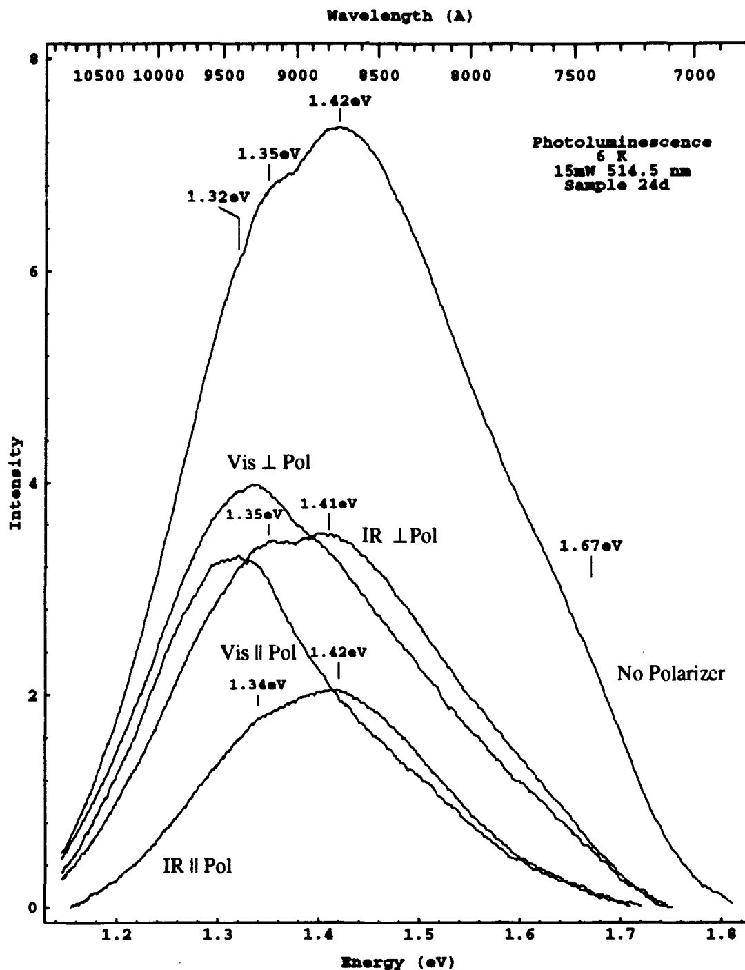
Figure 9. Photoluminescence spectra taken using 514.5 nm laser for sample 24d. Vis and IR indicate whether a visible or infrared polarizer was used. The \parallel and \perp symbols indicate whether the polarizer's pass direction was aligned along or perpendicularly to the sample's c-axis. Features marked on the spectra indicate possible transition energies.
