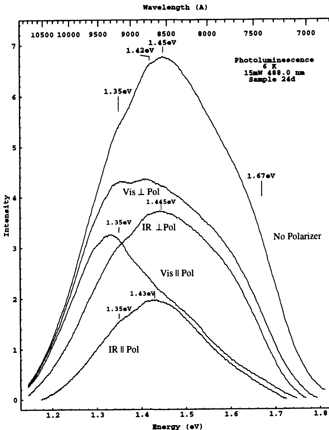
Figure 10. Photoluminescence spectra taken using 488.0 nm laser for sample 24d. Vis and IR indicate whether a visible or infrared polarizer was used. The \parallel and \perp symbols indicate whether the polarizer's pass direction was aligned along or perpendicularly to the sample's c-axis. Features marked on the spectra indicate possible transition energies.
