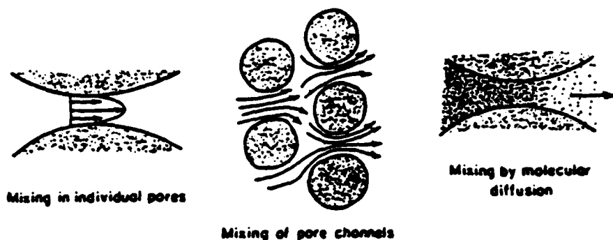
Figure 4: Processes of Dispersion on a Microscopic Scale (30:1 - 8)
