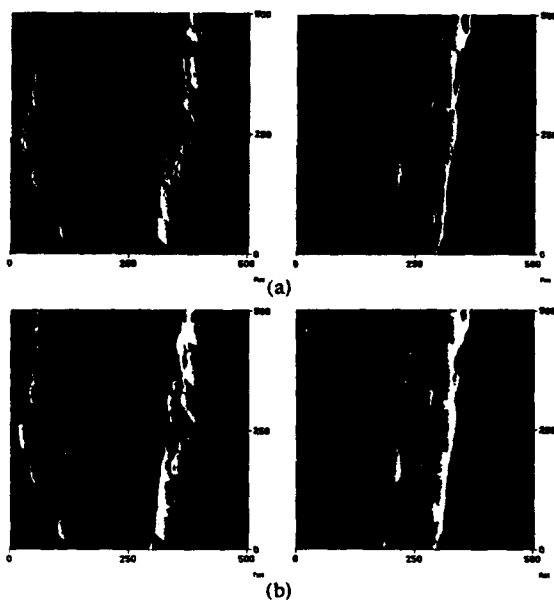
Fig. 11 Gray-scale plots of (a) the slope of the surface roughness and (b) the friction of a lubricated textured disk. The left side of the figure corresponds to the sample sliding from right to left and the right side of the figure corresponds to the sample sliding from left to right. Higher points are shown by lighter color.
