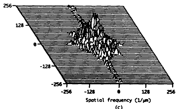
Fig. 5 Frequency spectra of (a) the surface roughness, (b) slope of the roughness, and (c) friction profile shown in Fig. 4. Vertical scale is logarithmic.
