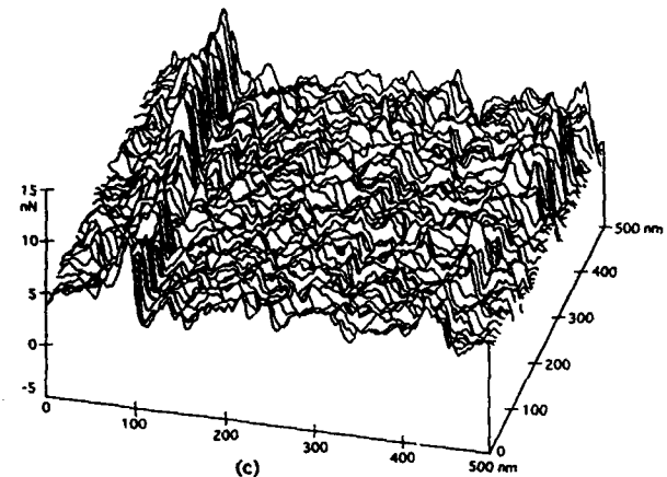
Fig. 6 (a) Surface roughness profile ( \sigma = 4.4 nm), (b) slope of the roughness profile taken along the sample sliding direction (mean = 0.023, \sigma = 0.197 ), and (c) friction profile of a textured and lubricated disk (mean = 6.2 nN, \sigma = 2.1 nN) for a normal load of 160 nN.
