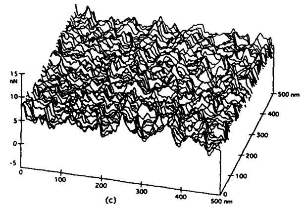
Fig. 7 (a) Surface roughness profile ( \sigma = 1.9 nm), (b) slope of the roughness profile taken along the sample sliding direction (mean = 0.001, \sigma = 0.111 ), and (c) friction profile of an as-polished and lubricated disk (mean = 6.0 nN, \sigma = 1.5 nN) for a normal load of 160 nN
