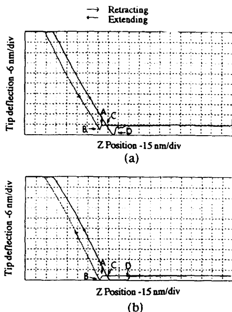
Fig. 1 Indentation curves of two metal-particle tapes (a) calendered, (b) uncalendered
