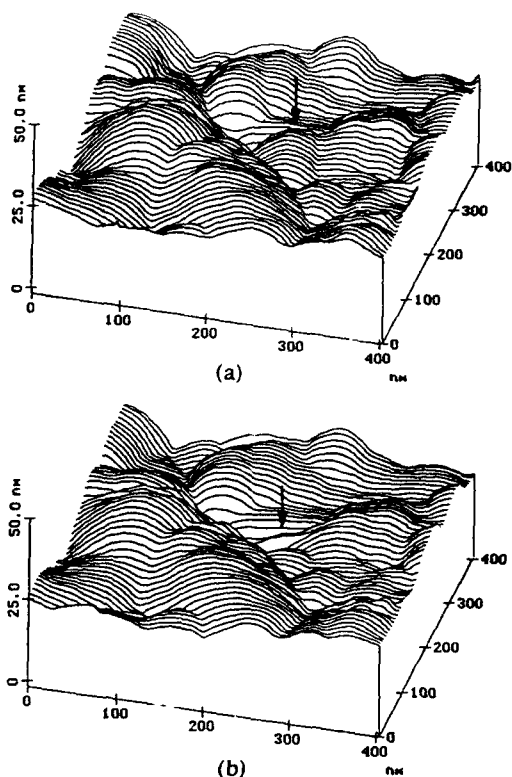
Fig. 3 Surface roughness profiles of a calendered metal-particle magnetic tape. The applied normal force was 10 nN and 100 nN for (a) and (b) respectively. Location of the change in surface topography as a result of microscratch is indicated by arrows.
