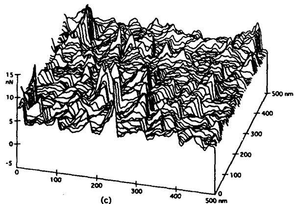
Fig. 4 (a) Surface roughness profile ( \sigma = 7.9 nm), (b) slope of the roughness profile taken along the sample sliding direction (the horizontal axis) (mean = -0.006 , \sigma = 0.300 ), and (c) friction profile (mean = 5.5 nN, \sigma = 2.2 nN) of a calendered metal-particle tape for a normal load of 70 nN. There is poor correlation between the surface roughness and friction. However, the slope of the roughness profile has an excellent correlation with the friction profile. ( \sigma is the standard deviation).
