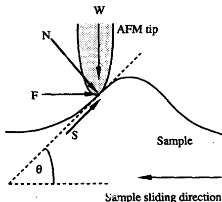
Fig. 9 Schematic illustration showing the effect of an asperity (making an angle \theta with the horizontal plane) on the surface in contact with the tip on local friction in the presence of "adhesive" friction mechanism (Tabor, 1979). W and F are the normal and friction forces, respectively. S and N are the force components along and perpendicular to the local surface of the sample at the contact point, respectively.
