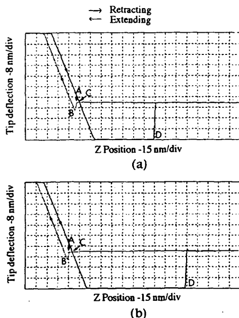
Fig. 2 Indentation curves of (a) unlubricated and (b) lubricated textured disks. The pull-off force is larger in the lubricated disk (84 nN) than in the unlubricated disk (42 nN) calculated from the horizontal distance between points C and D and the cantilever spring constant of 0.4 N/m.
