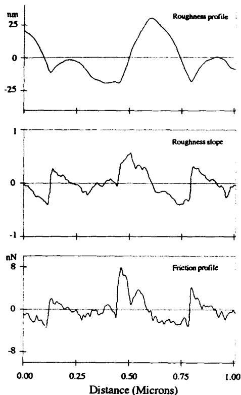
Fig. 8 Surface roughness profile ( \sigma = 15.4 nm), slope of the roughness profile (mean = -0.052 , \sigma = 0.224 ) and friction profile ( \sigma = 2.1 nN) of a polished natural (IIa) diamond crystal. The slope of the roughness profile closely resembles the friction profile.
