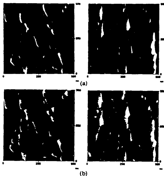
Fig. 10 Gray-scale plots of (a) the slope of the surface roughness and (b) the friction of a calendared metal-particle tape. The left side of the figure corresponds to the sample sliding from right to left and the right side of the figure corresponds to the sample sliding from left to right. Higher points (in friction or in roughness slope) are shown by lighter color.
