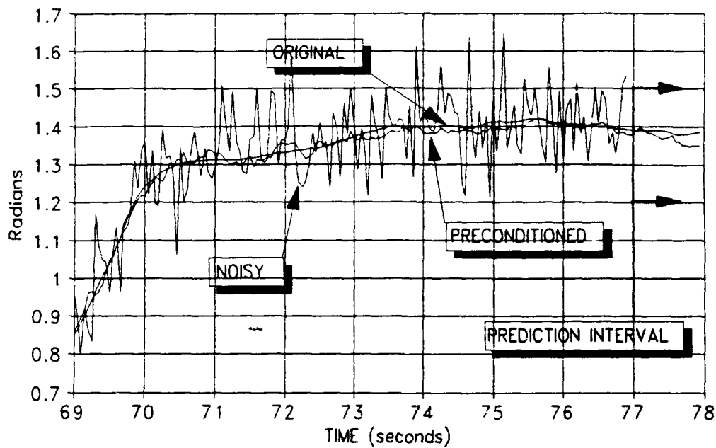
Figure 2 Trajectory Measurement Data: Roll
