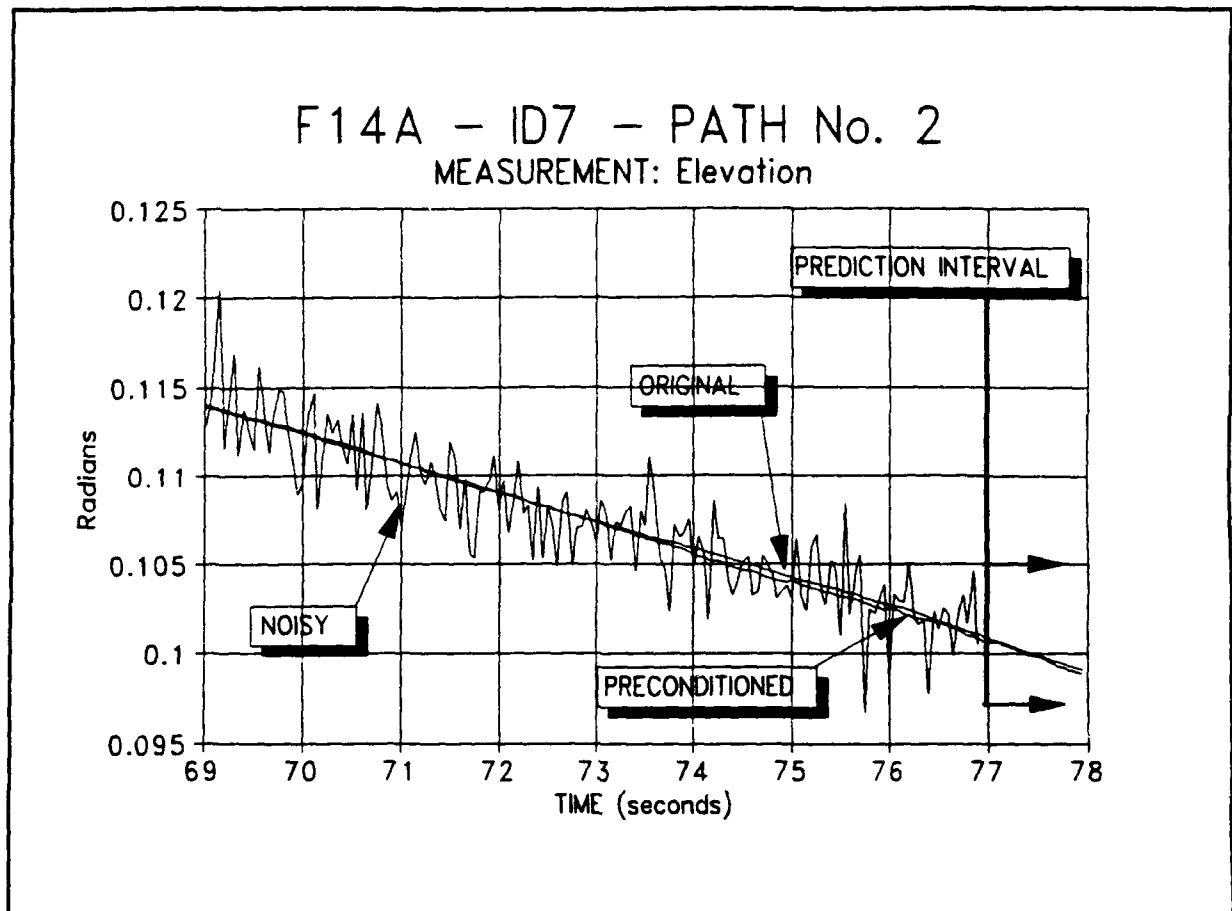
Figure 7 Trajectory Measurement Data: Elevation
