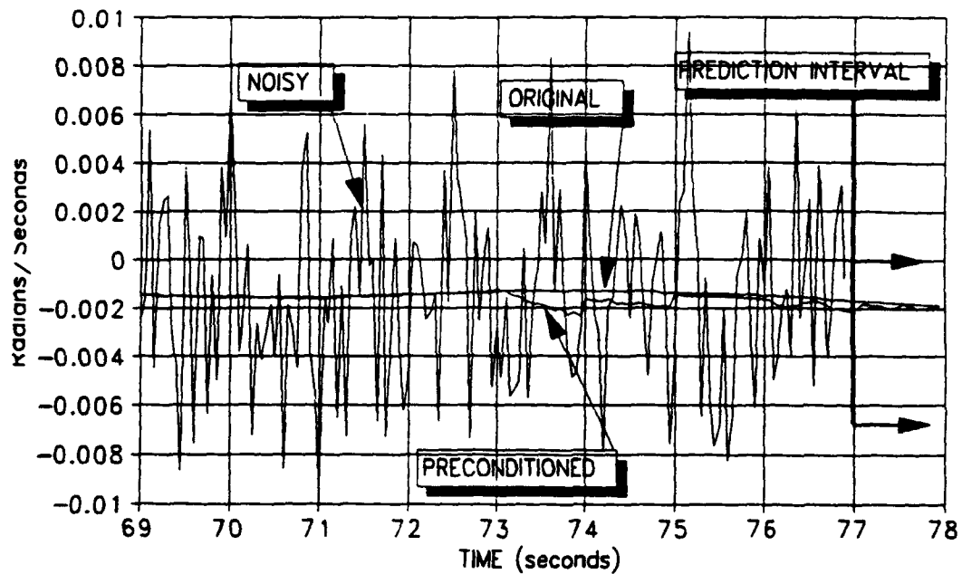
Figure 10 Trajectory Measurement Data: Elevation Rate
