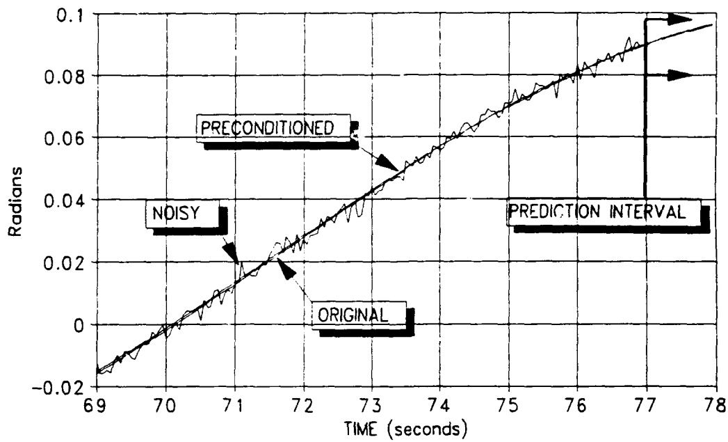
Figure 6 Trajectory Measurement Data: Azimuth
