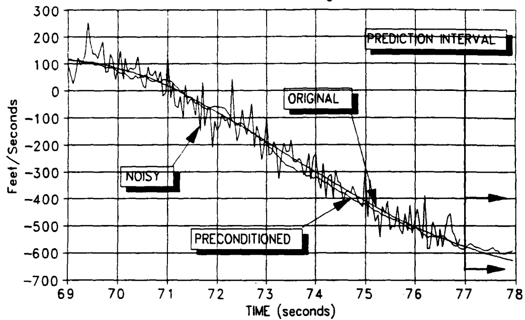
Figure 8 Trajectory Measurement Data: Range Rate
