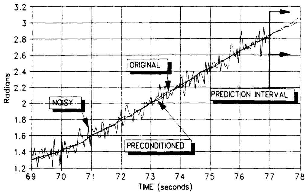
Figure 4 Trajectory Measurement Data: Yaw
