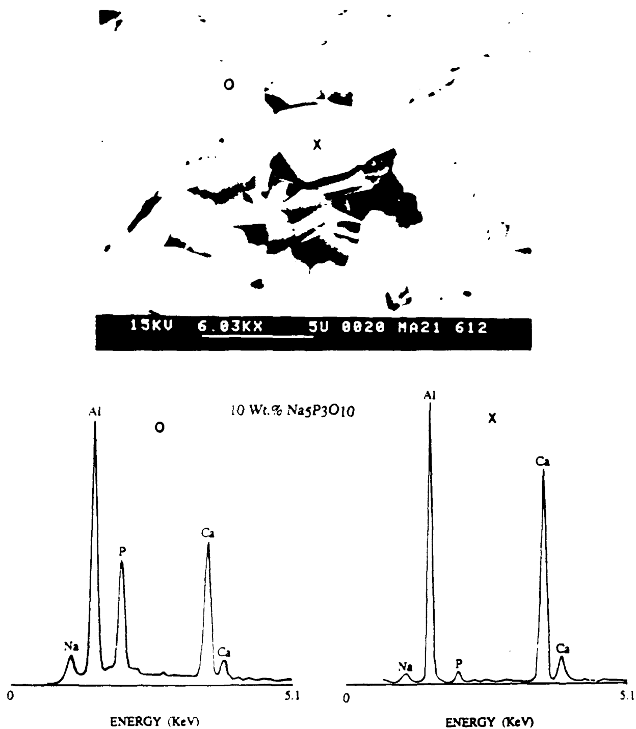
Figure 30. Morphologies and the associated EDX spectra for \text{Na}_5\text{P}_3\text{O}_{10} modified HAC
