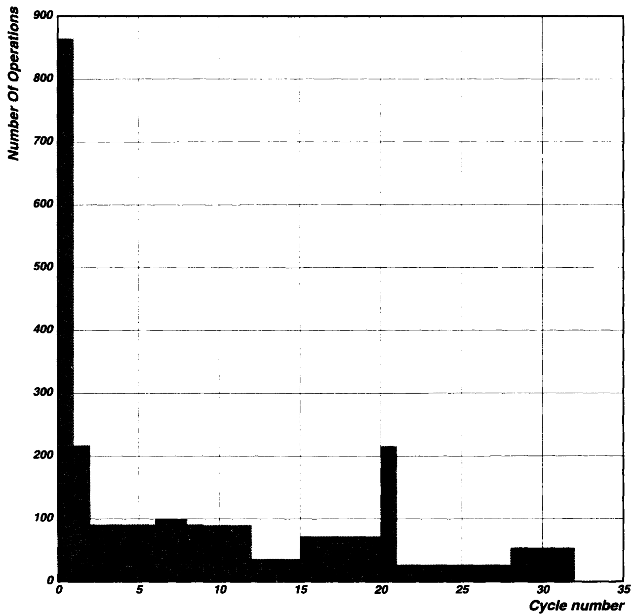
Figure 4-1: Parallelism profile of a 9 body Stormer integration[4]
