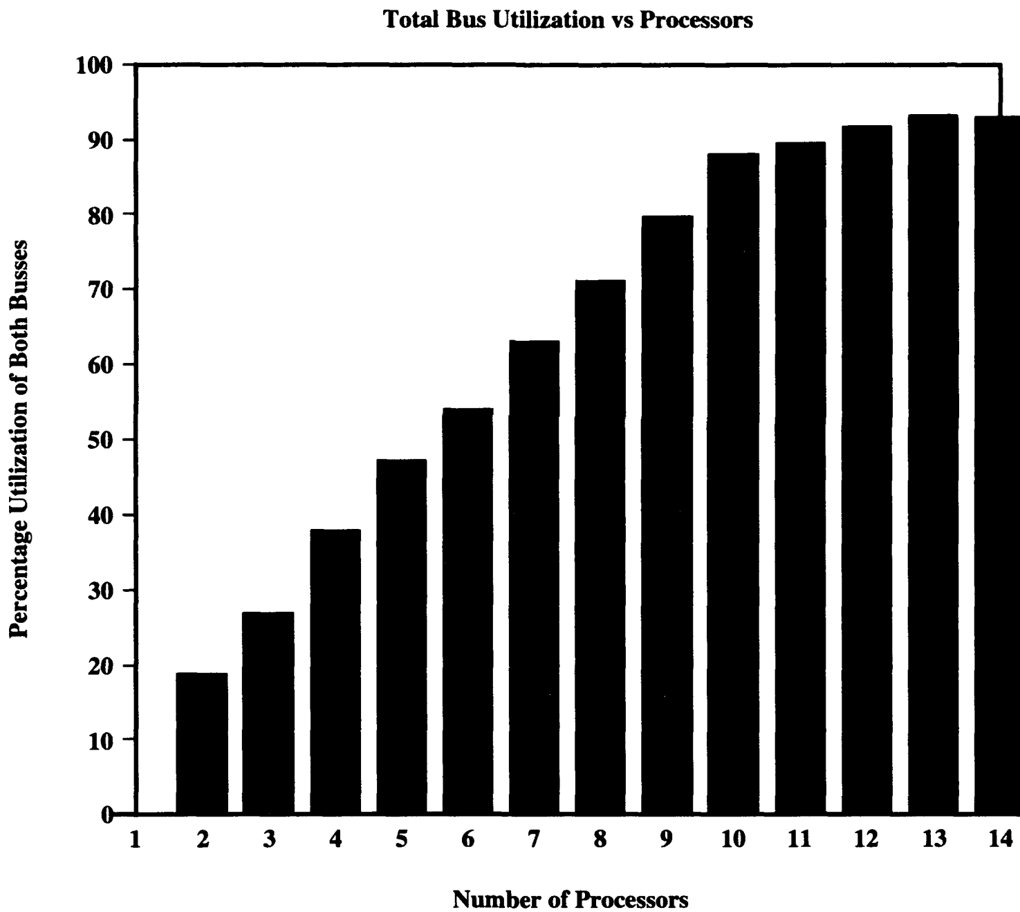
Figure 4-5: Bus Utilization vs Processors for ST9.
