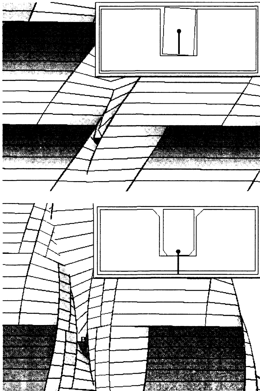
Figure 4.28: Initial (top) and final (bottom) peg-hole geometries and closeups of the motion constraints local to the goal region of a simple compliant assembly task.
