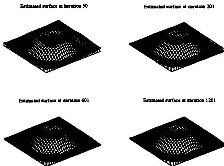
Figure 5-3: Performance of the z-only algorithm on the easy crater images. The upper-left graph shows the cost function (solid line) and RMS error of the estimated surface (dashed-line) plotted against the number of function evaluations. The upper-right graph shows the history of the \lambda cost function parameter. Also shown are images based on the estimated surface and mesh plots of the surface at different points during optimization.
