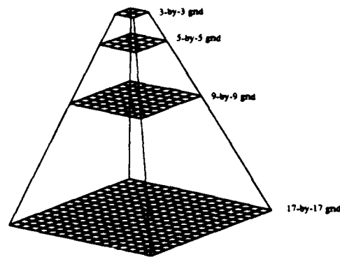
Figure 3-3: Multigrid levels
