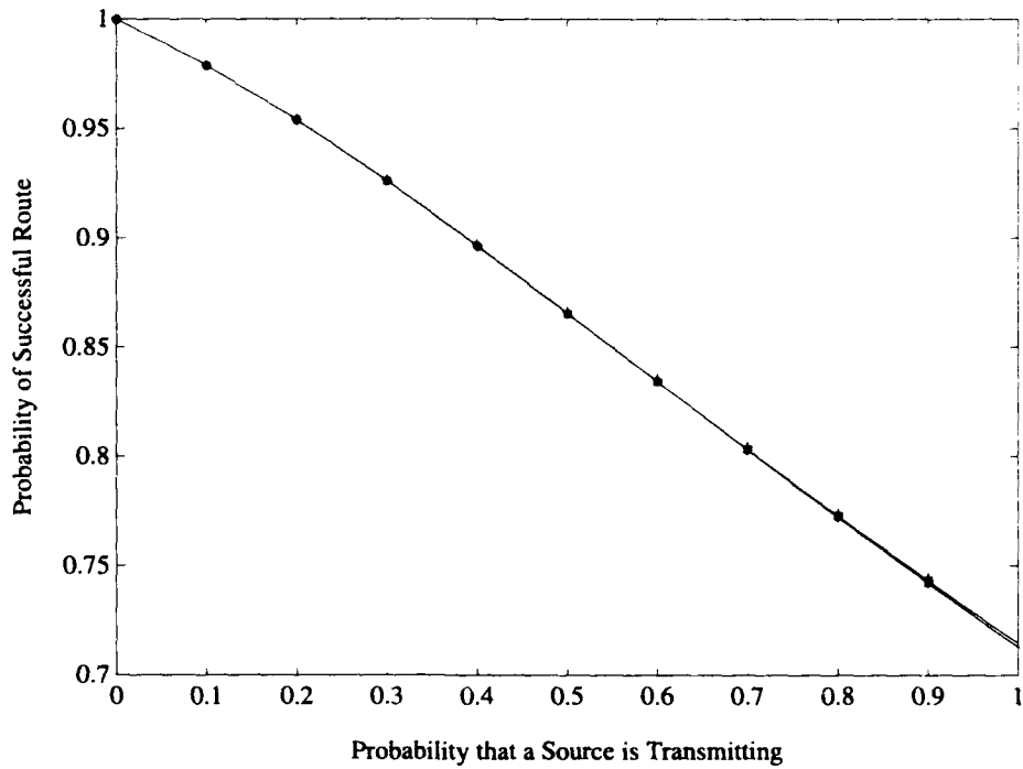
Figure 4.11: Normalized Routing Statistics for Full Fat-Trees
