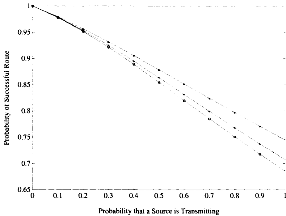
Figure 4.8: Routing Statistics for Full Fat-Tree (64 processors)
