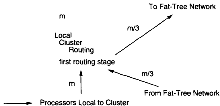
Figure 2.1: Bidelta Cluster at Leaves of Fat-Tree
