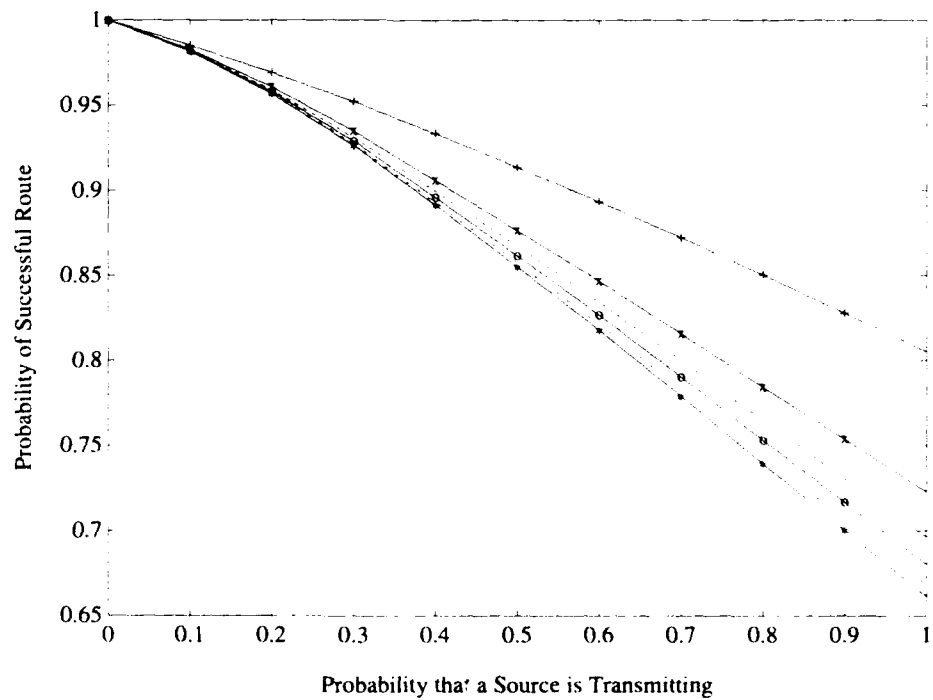
Figure 4.15: Routing Statistics for Hybrid Fat-Tree (49152 processors)
