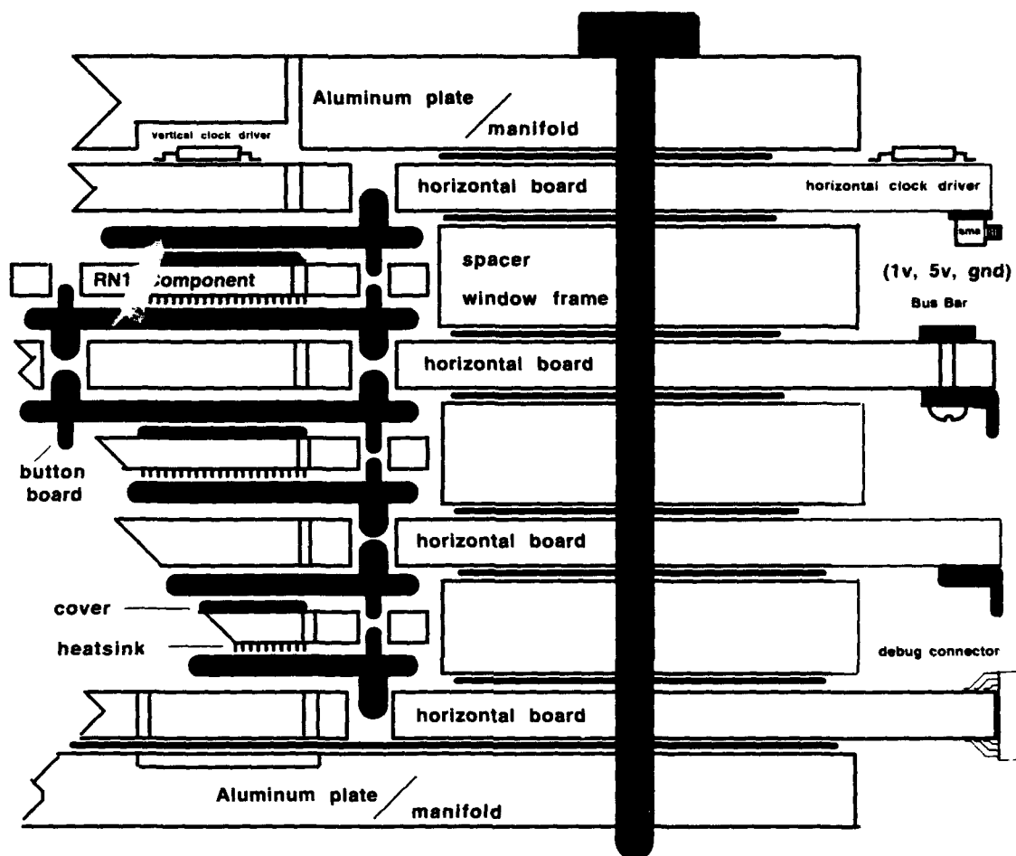
Figure 1.4: Cross-Section of Bidelta Routing Stack (Diagram courtesy of Fred Drenckhahn)
