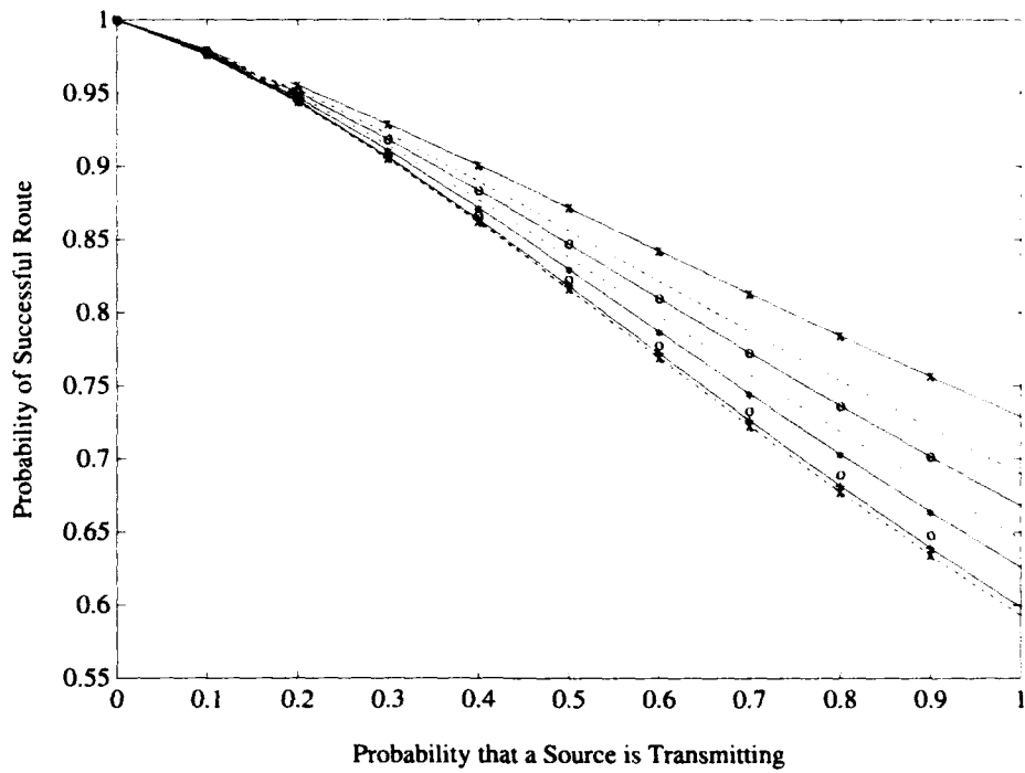
Figure 4.10: Routing Statistics for Full Fat-Tree (262144 processors)
