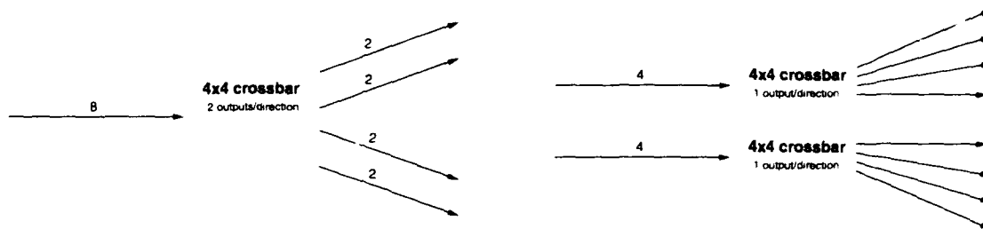
Figure 1.2: RN1 Logical Configurations
