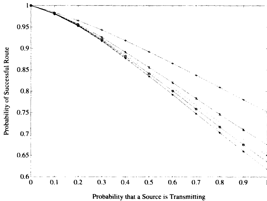
Figure 4.17: Routing Statistics for Hybrid Fat-Tree (786432 processors)
