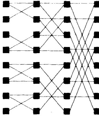
Figure 4.5: Indirect Binary Cube Topology
