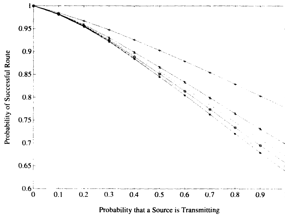
Figure 4.16: Routing Statistics for Hybrid Fat-Tree (196608 processors)
