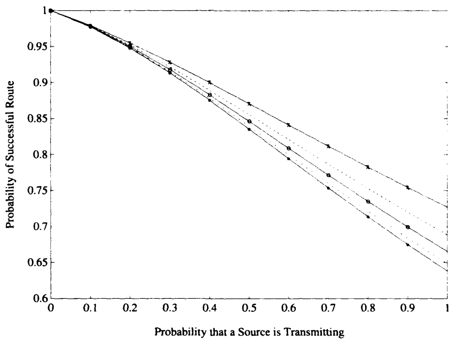
Figure 4.9: Routing Statistics for Full Fat-Tree (4096 processors)
