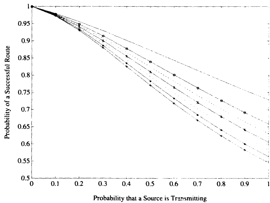
Figure 4.19: Routing Statistics for Full Bidelta Networks of Various Sizes
