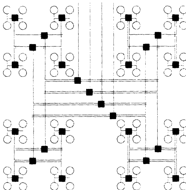
Figure 1.5: Area-Universal Fat-Tree with Constant Size Switches (Greenberg and Leiserson)
