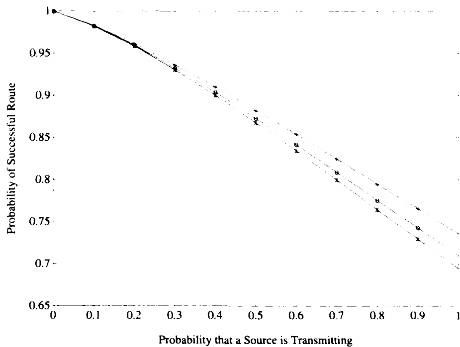
Figure 4.12: Routing Statistics for Hybrid Fat-Tree (768 processors)
