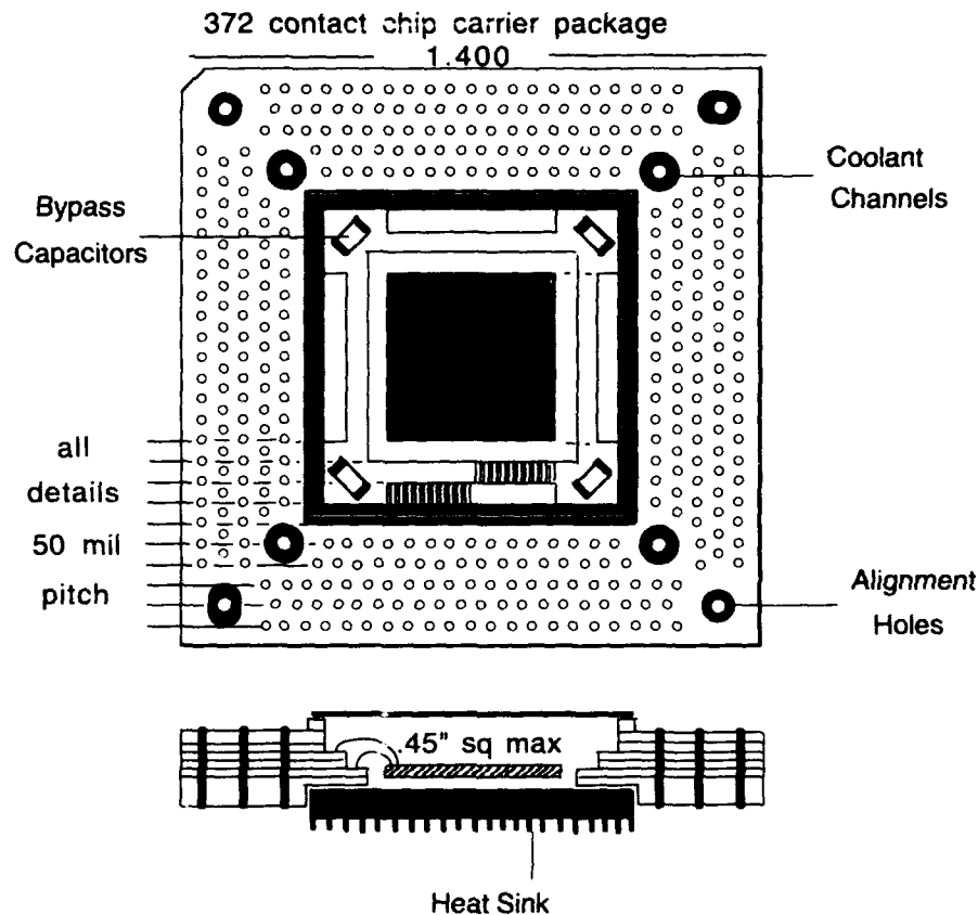
Figure 1.3: RN1 Package (Diagram courtesy of Fred Drenckhahn)
