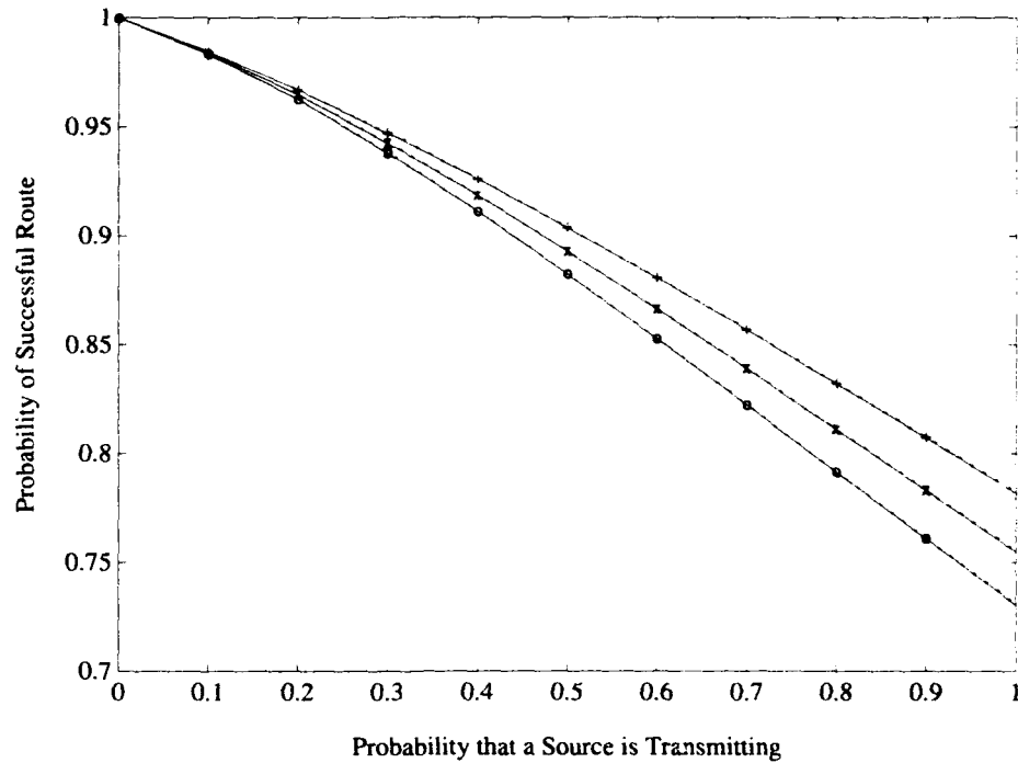
Figure 4.18: Normalized Routing Statistics for Hybrid Fat-Tree
