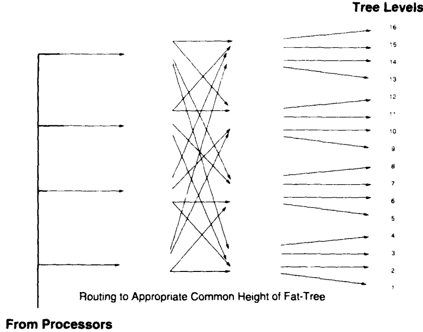
Figure 2.7: Hybrid Up Routing Scheme with \log_4 \log_4 N Stages in Up Routing Tree
