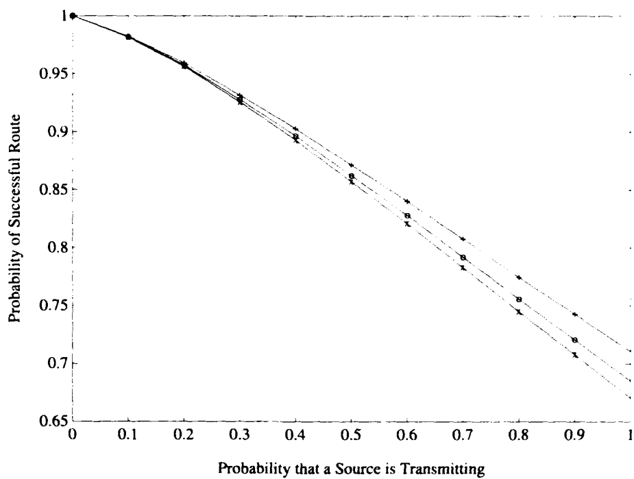
Figure 4.13: Routing Statistics for Hybrid Fat-Tree (3072 processors)
