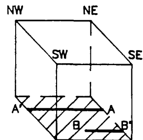
Figure 36. Plan of Unit N999, E879, showing excavated archeological features, and section lines.
