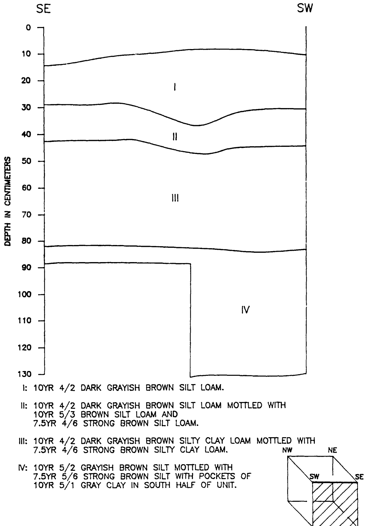
Figure 15. Stratigraphic profile of the south wall of Unit N833, E1012 at Site 16WBR18.
