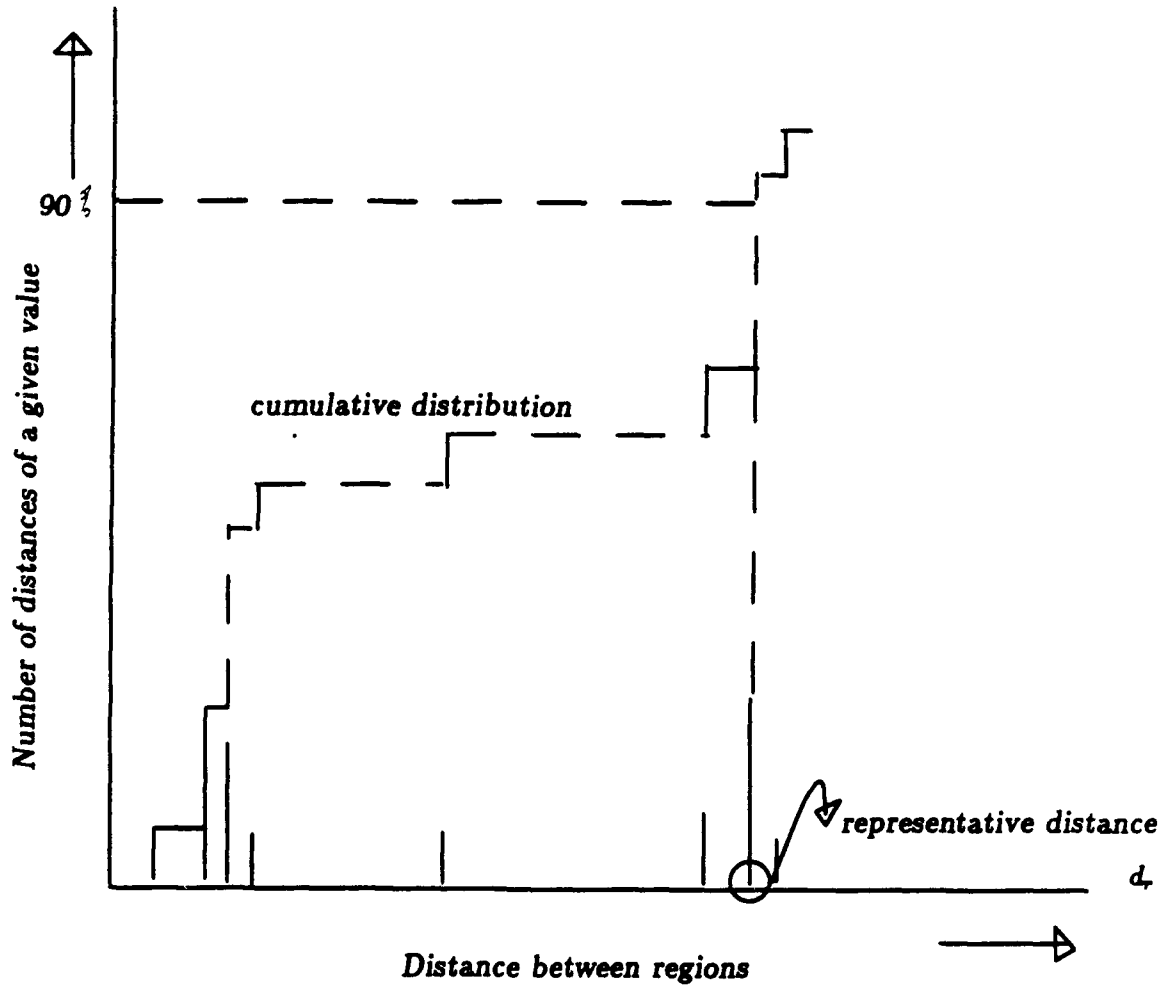
Figure 4.23: Illustration of the choice of representative distance d_r for characterizing distance distribution.
