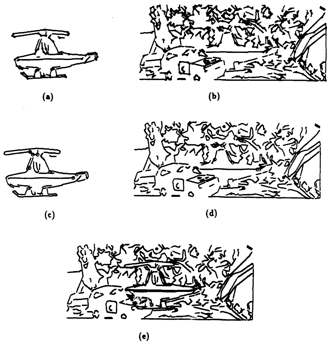
Figure 1.1: Illustration of object recognition. (a) A view of a model object with corner features (in circles) and edges. (b) A scene in which the object appears. (c)- (d) A set of matching corner features in the model and image respectively that were found to give the correct transformation. (e) The model overlaid on the image of (b) using the transformation computed from the corresponding features shown by the big circles in (c) and (d).
