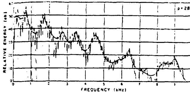
Figure 4.5: Illustration to show that the LP spectrum can be sampled at a lower rate than the Fourier transform of the signal. The plot shows a 28-pole fit to a speech spectrum and is taken from [98]. A suggested sampling rate of the LP spectrum has been superimposed on the plot.
