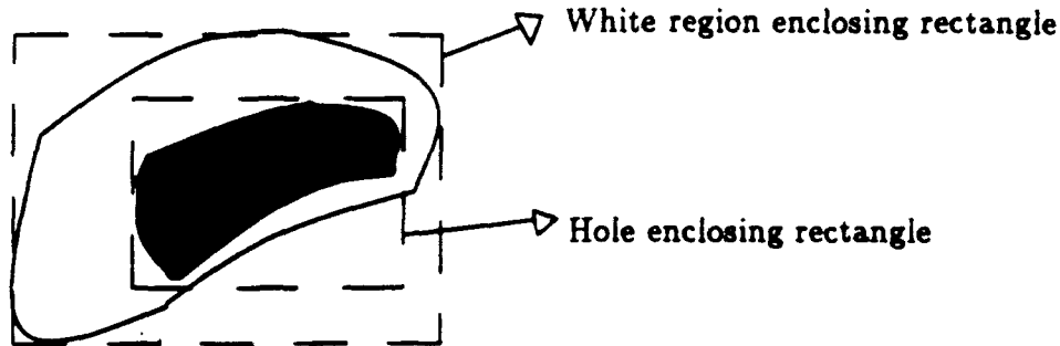
Figure 4.15: Hole detection test for binary maps. A black region is considered to be inside a white region if its enclosing rectangle is inside the enclosing rectangle of the white region.
