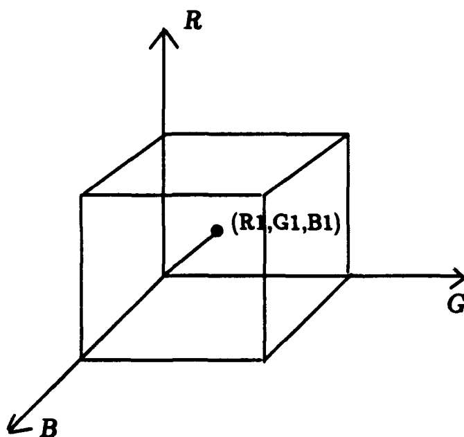
Figure 3.2: The rgb-color space. The axes here stand for the pure red, green, and blue components of intensity obtained using the respective filters.
