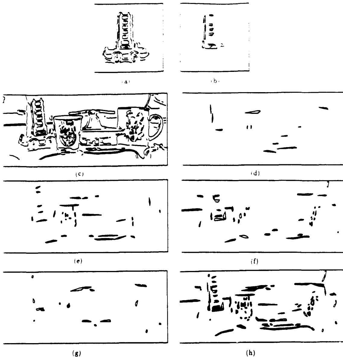
Figure 5.8: Illustration of line-groups-based model-driven selection. (a) Edge image of a model object showing instances of closely-spaced parallelism between lines. (b) Some of the line groups extracted using the grouping algorithm using the constraints of t_{\text{across}} = 5 , t_{\text{along}} = 0 , t_{\text{local-orient}} = 6 , t_{\text{global-orient}} = 10 . (c) An edge image of a scene in which the model object appears. (d) - (g) Augmented closely-spaced line groups generated using the description of the model line groups shown in (b). (h) The line groups in the image that are possible matches to the model line groups of (b) under the allowed scale and pose changes.
