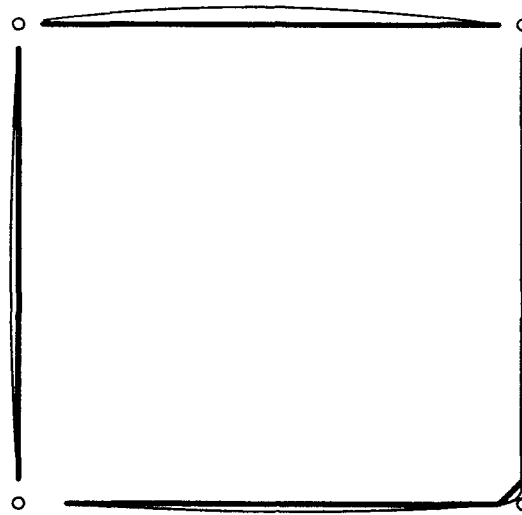
Figure 6.12: In the group shown above, a rounded corner's approximation contains a small line at the corner. If this line does not contribute to a stable corner, we may ignore it and form a corner from its neighboring lines. Edges are shown with a lighter weight, line approximations are shown in heavy weight. Circles show where we would like to find corners.
