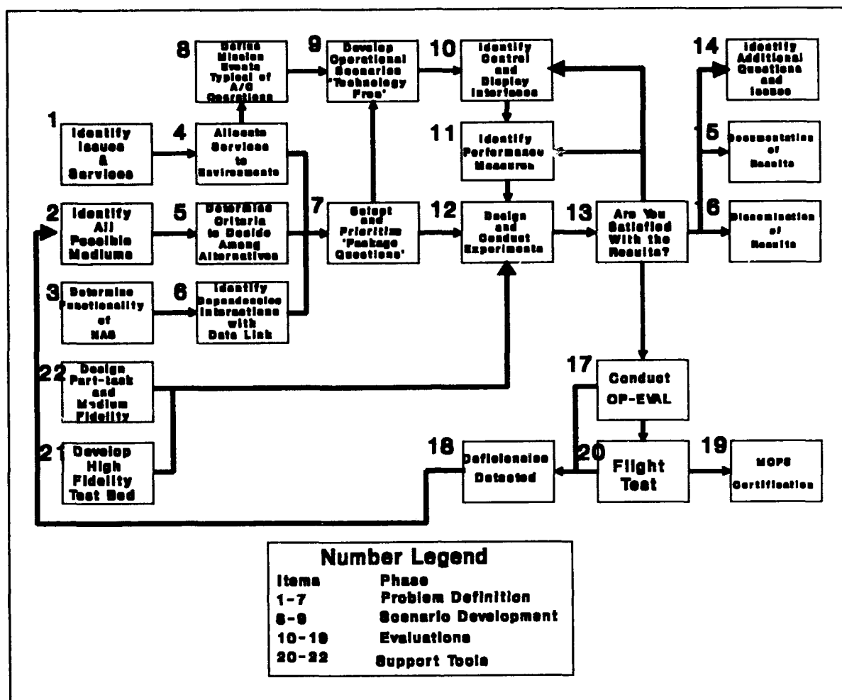
FIGURE 1. FAA TECHNICAL CENTER DATA LINK RESEARCH APPROACH
