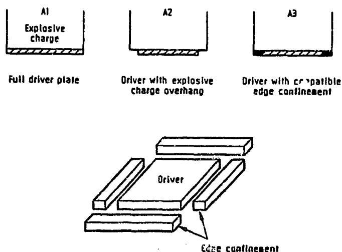
Figure 3: Driver configurations.
