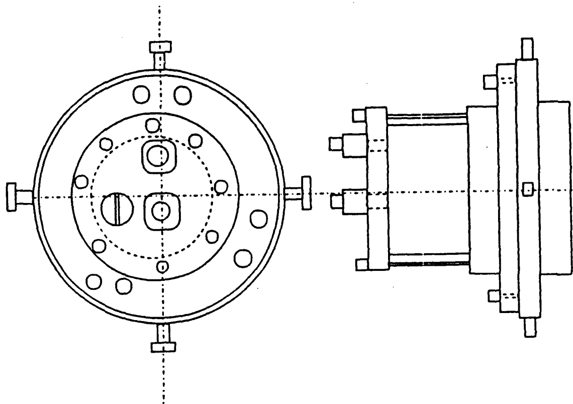
Figure 20: Front and top view of the scattering cell and its holder assembly.
