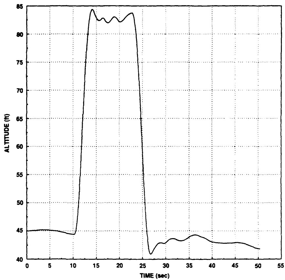
Figure C-5. Bob-up time history data for simulator (Pilot 2).
