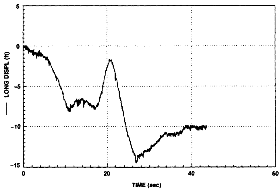
Figure C-3. Bob-up time history data for flight (Pilot 3) (Continued).
