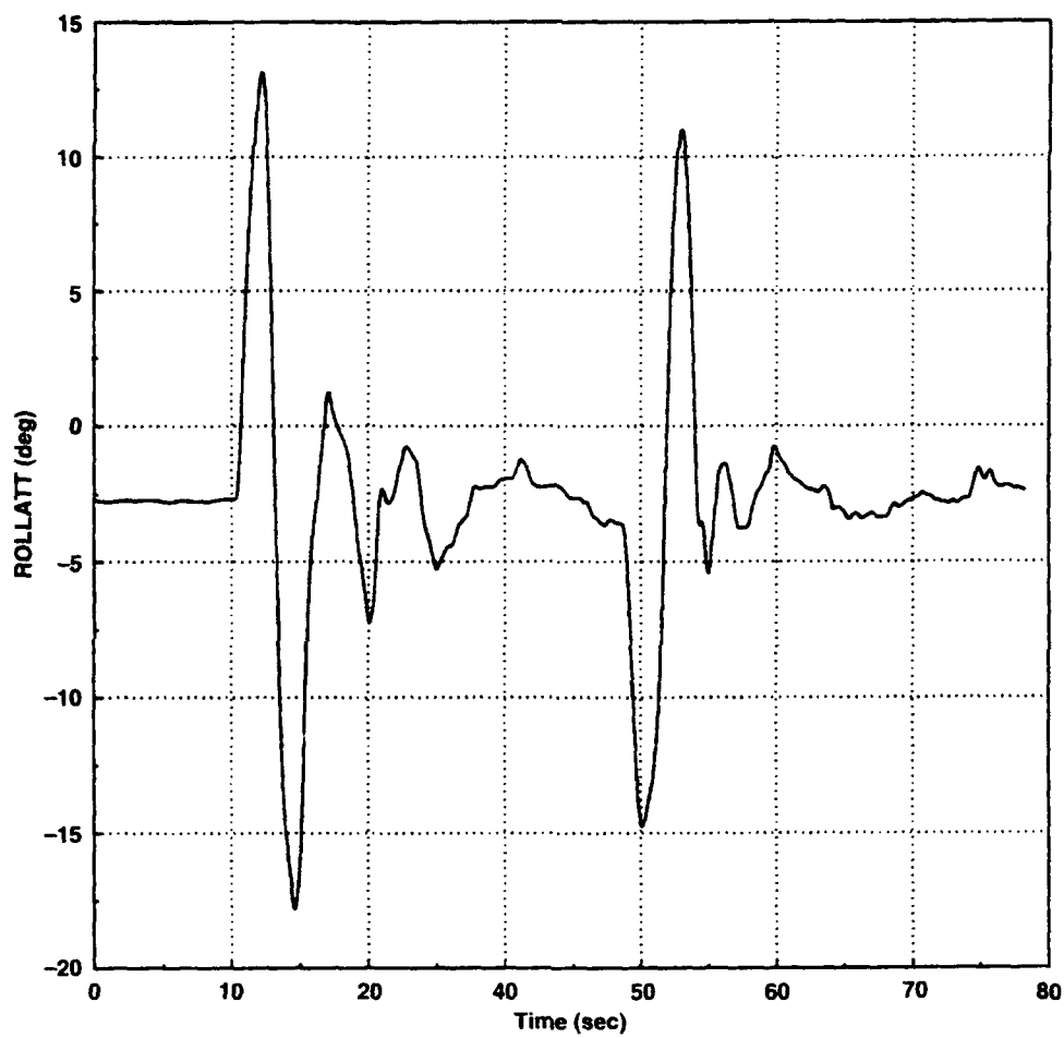
Figure C-13. Side-step time history data for simulator (Pilot 4) (Continued).
