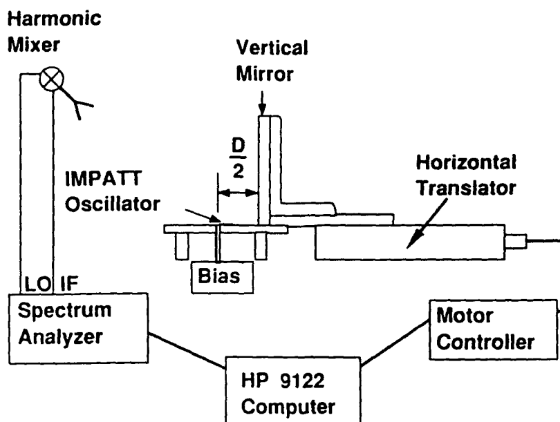
Fig. 1. Experimental setup for measurement of frequency variation versus separation distance between a single oscillator and a vertical mirror. (from Ref. [1])
