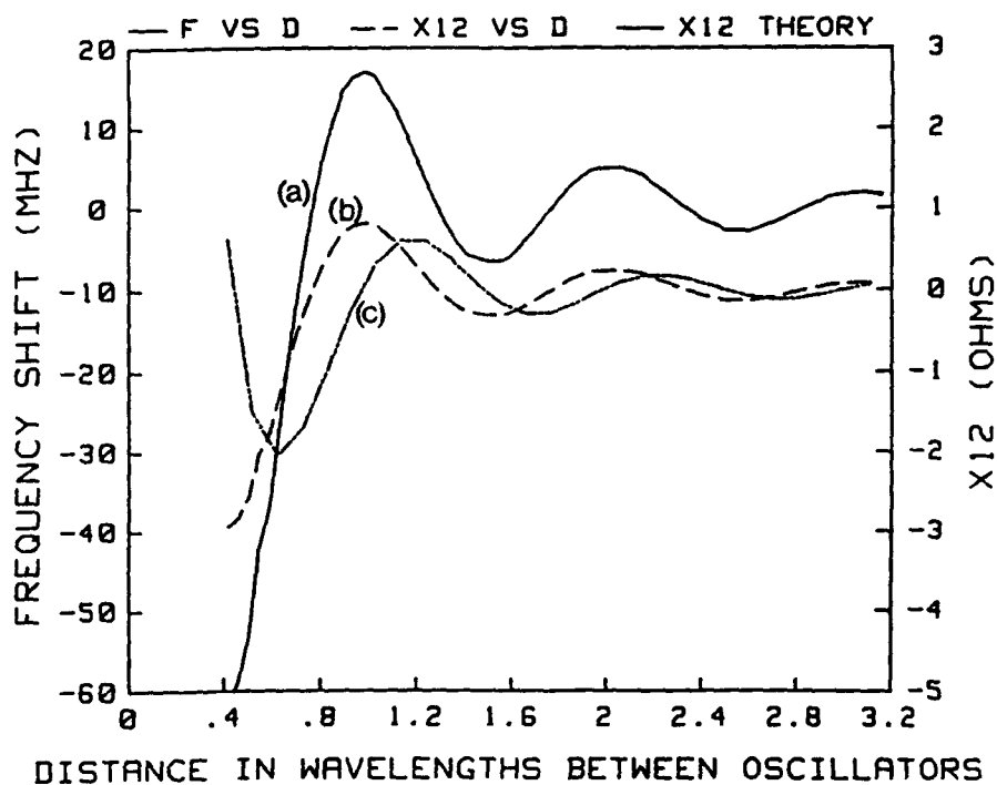
Fig. 2. (a) Measurement of \Delta f versus D (interoscillator spacing). (b) X_{12} versus D converted from frequency measurement. (c) X_{12} versus D derived from mutual impedance radiation model. (from Ref. [1])
