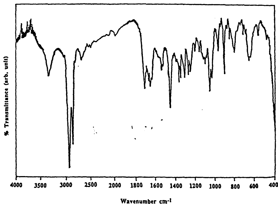
FIG. 2. FTIR of B-PMHT in KBr disc.
