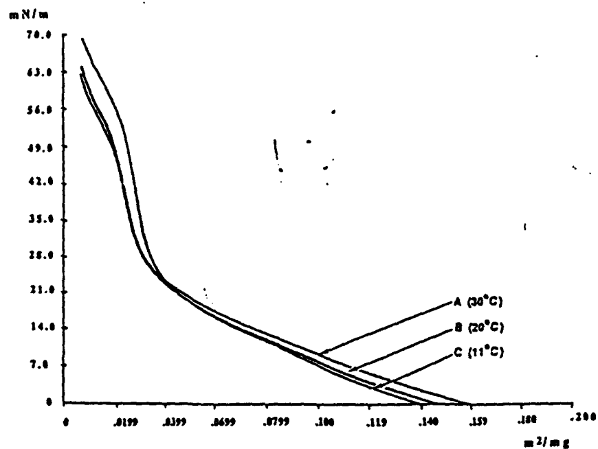
FIG. 5. Stability of B-PMHT at various temperatures.
