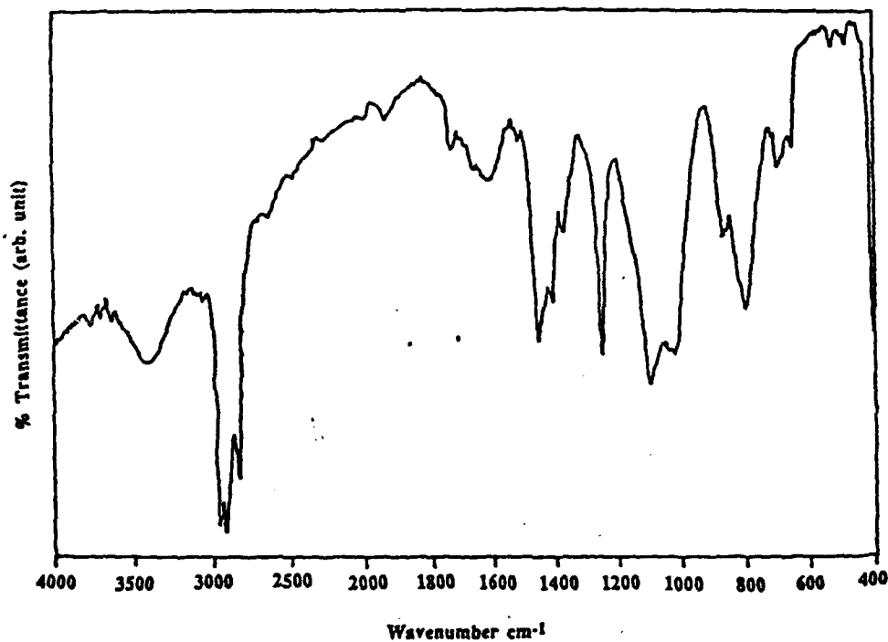
FIG. 1. FTIR of PMHT in KBr disc.
