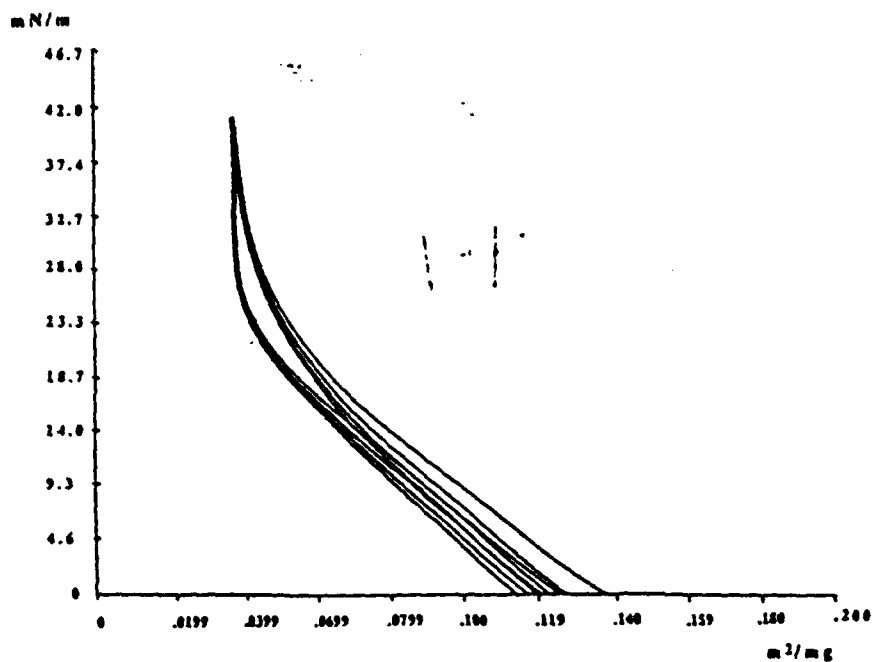
FIG. 4. Hysteresis effect upon repeated recompression and decompression cycles on B-PMHT.
