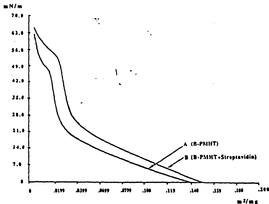
FIG. 3. Pressure-area isotherms of B-PMHT, streptavidin injected in B-PMHT.
