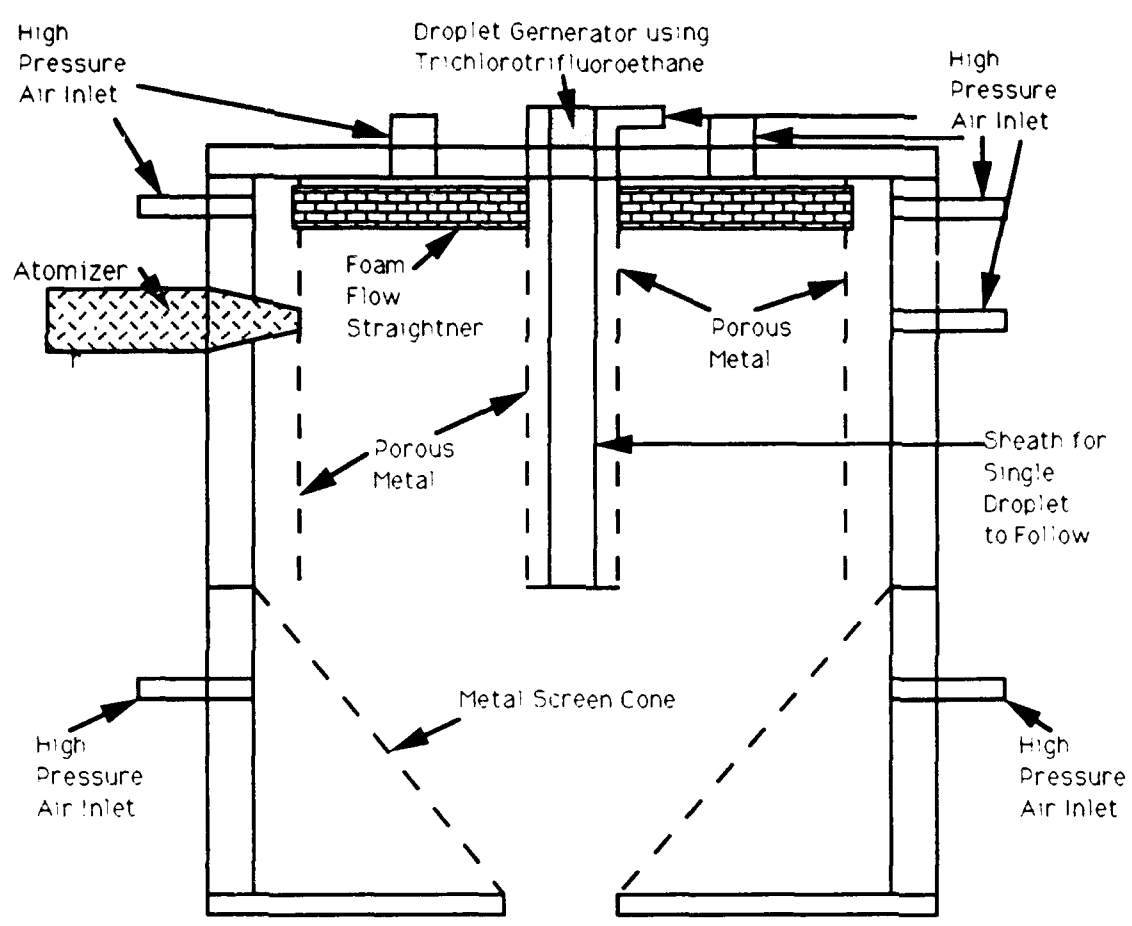
Figure 2. Experimental Apparatus for Spray Droplet Dispersion
