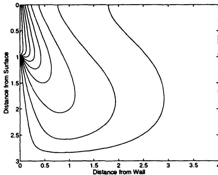
Figure 18. Steady-State Temperature Distribution ( h = 0.02 , M = 100 ): Contour plot of the temperature solution. The uniform grid spacing is reduced to 0.02 and the isotherms are very close to each other, forming a compressed region close to the wall.
