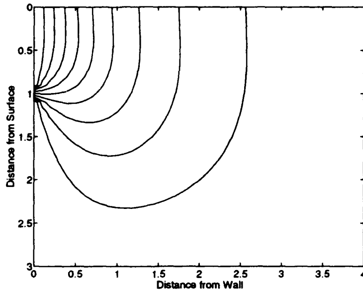
Figure 16. Steady-State Temperature Distribution ( h = 0.1 , M = 10 ): Contour plot of temperature solution shows slight evidence of convection in the flow.
