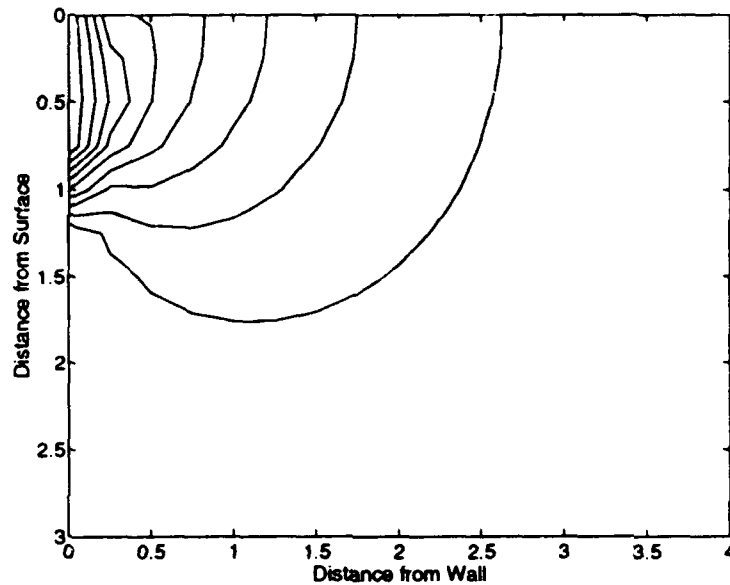
Figure 10. Temperature Distribution obtained from FORTRAN Routine ( h = 0.25 , M = 0 ): Contour plot of temperature distribution (purely conductive).
