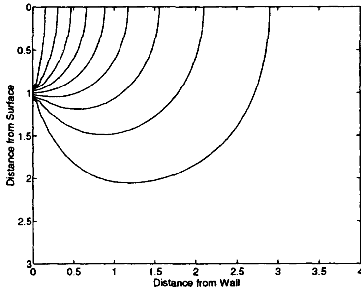
Figure 12. Steady-State Temperature Distribution from MATLAB routine ( h = 0.1 , M = 1 ): Contour plot of temperature solution showing no evidence of convection in the flow.
