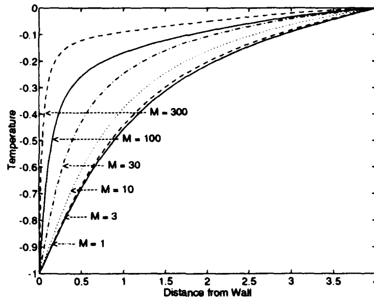
Figure 21. Steady-State Surface Temperature for Various M Values: This plot shows that as M increases, the surface temperature rises more rapidly as the distance from the wall increases. As the flow becomes more convective (high M ), the change in surface temperature is concentrated near the wall.
