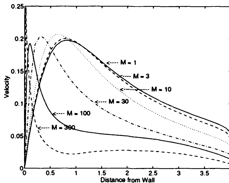
Figure 24. Steady-State Surface Velocity Profiles for Various M Values: As M increases, the surface velocity exhibits a sharper rise to its maximum value (closer to the wall), and a steeper descent into the bulk pool as well.
