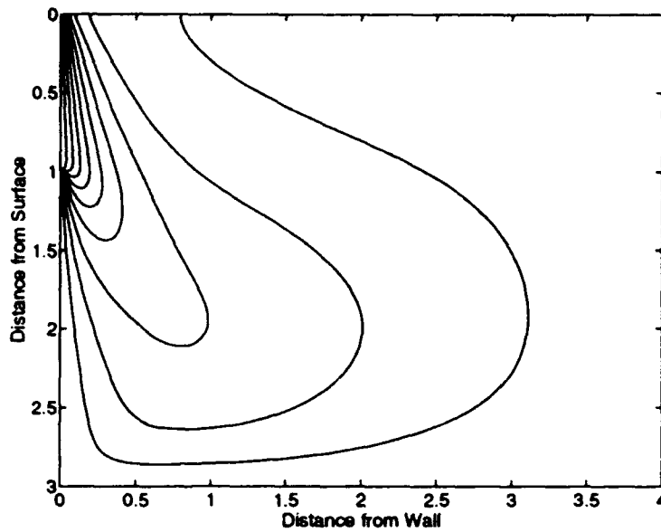
Figure 20. Steady-State Temperature Distribution ( h = 0.02 , M = 300 ): Contour plot of the temperature solution. The isotherms appear to meet at the wall-surface corner. The transition to convective behaviour is complete.
