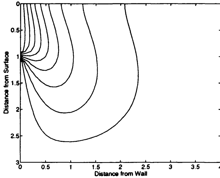
Figure 17. Steady-State Temperature Distribution ( h = 0.1 , M = 30 ): Contour plot of temperature solution shows stronger effects of convection in the flow. Closely spaced isotherms indicate rapid growth in temperature near the wall.
