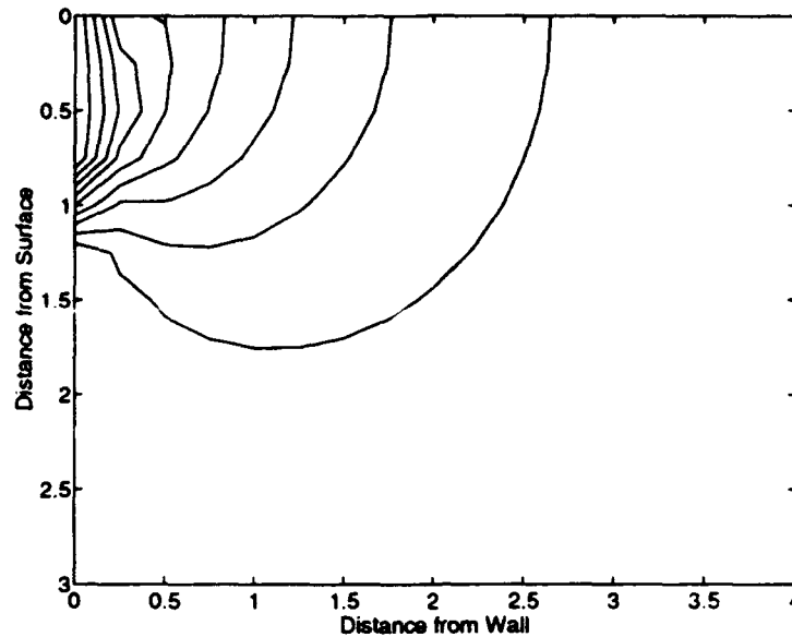
Figure 11. Temperature Distribution obtained from FORTTRAN Routine ( h = 0.25 , M = 1 ): Contour plot of temperature solution showing no evidence of convection in the flow.
